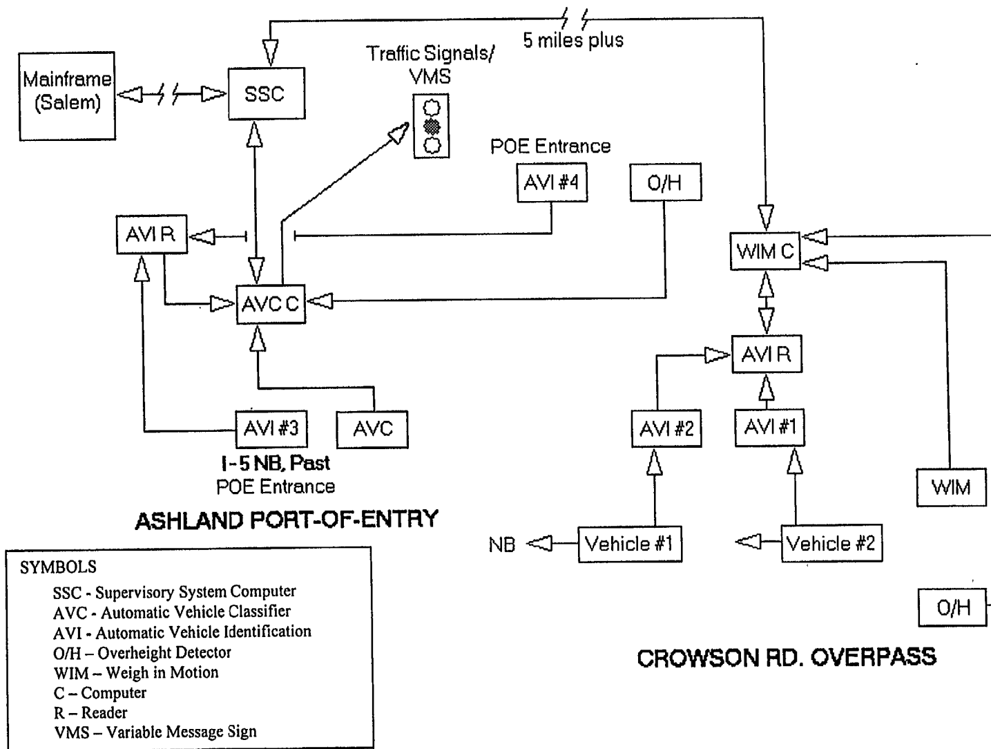
Figure 2.3: Data Flow for PASS
