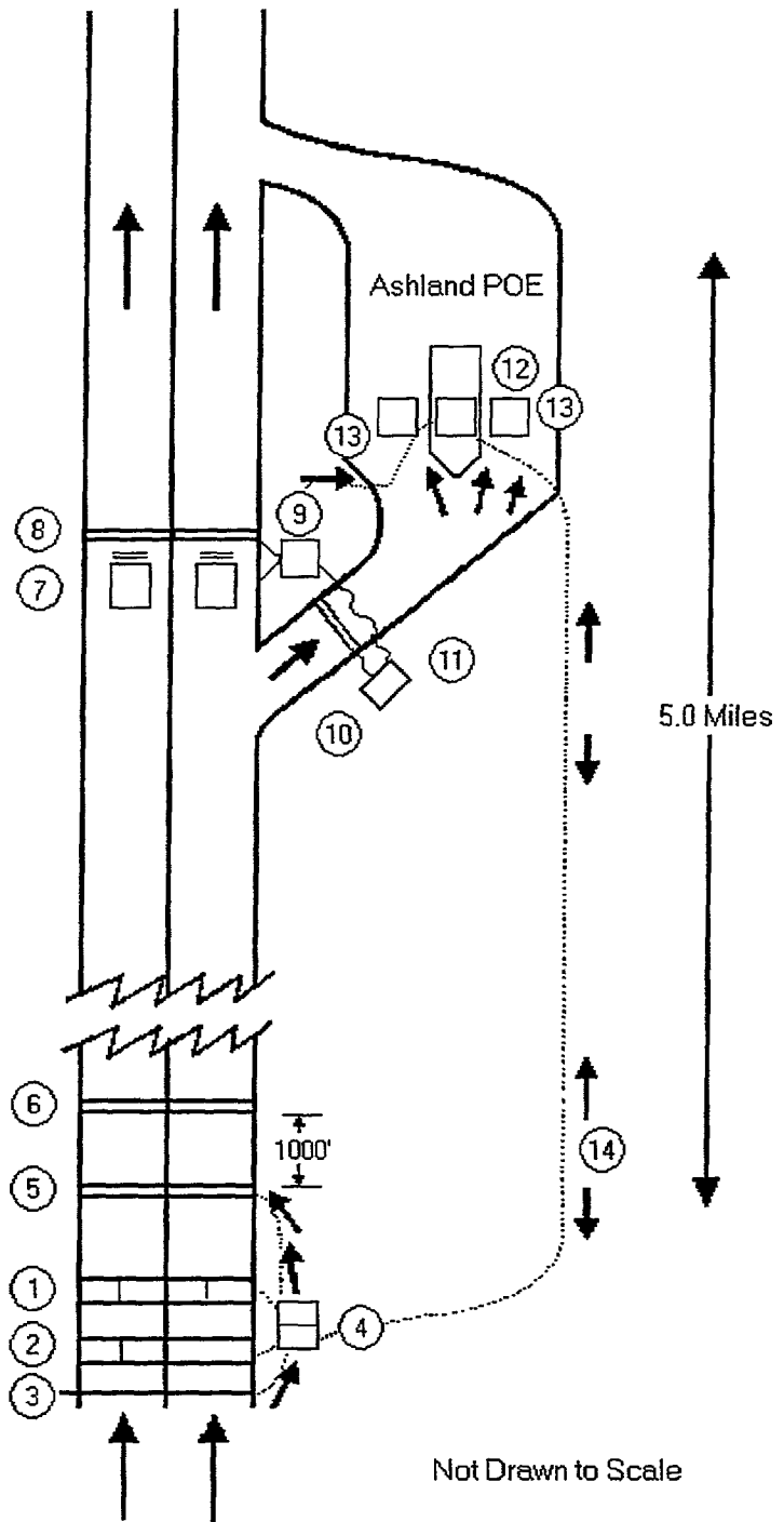
Figure 2.2: Port-of-Entry Advanced Sorting System
