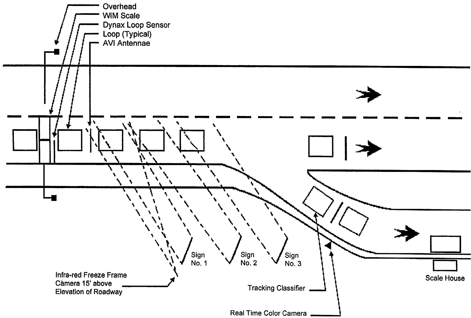
Figure 2.1: Conventional mainline sorting system
