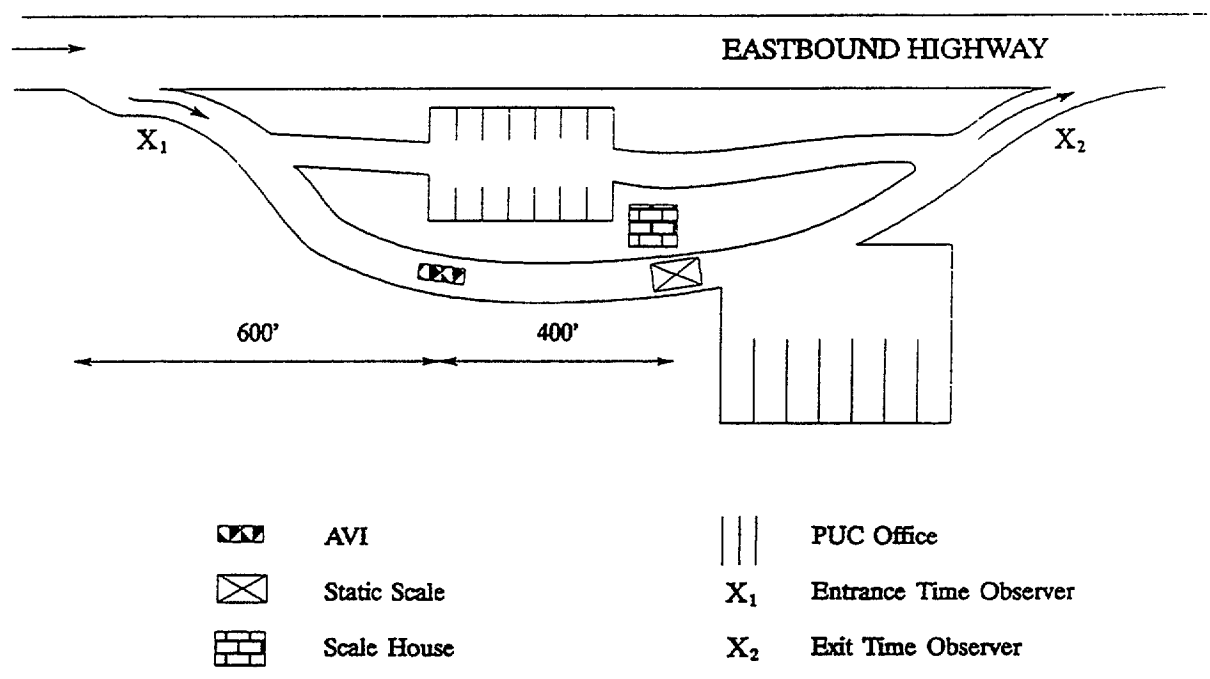
Figure 2-7. Lordsburg: Location and Layout
