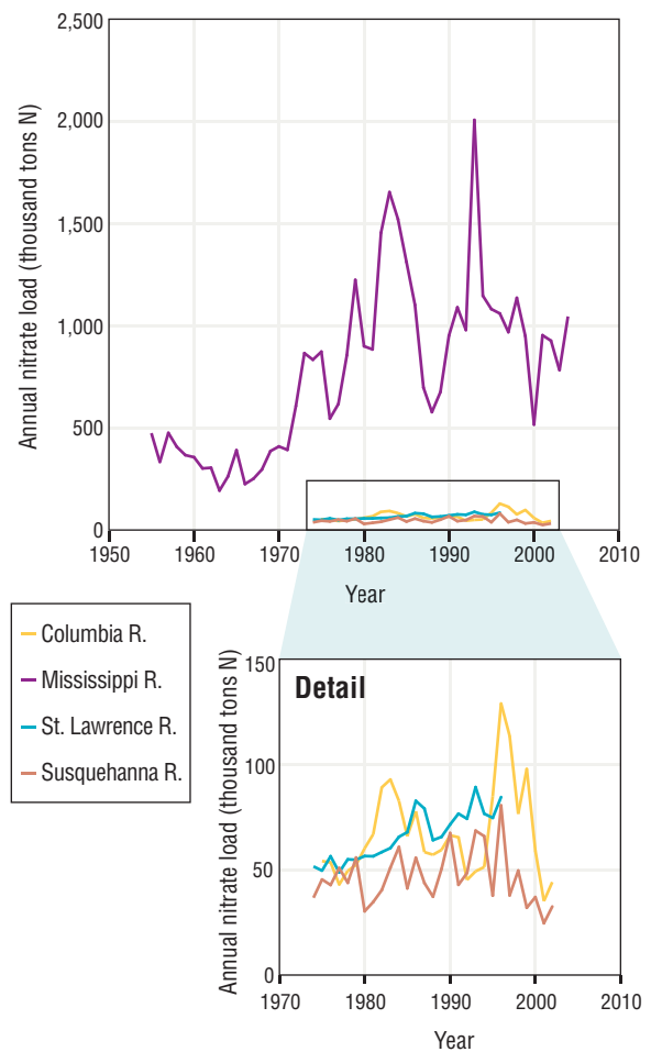
Exhibit 3-10. Nitrate loads in four major U.S. rivers, 1955-2004 a
