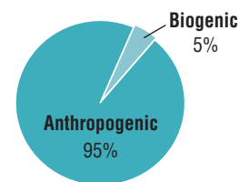
B. Relative amounts of \text{NO}_x emissions from anthropogenic and biogenic sources, 2002
