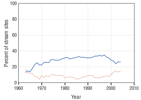
Exhibit 3-5. Changes in the maximum duration of no-flow periods in intermittent grassland/shrubland streams of the contiguous U.S., 1961-2006, compared with 1941-1960 baseline a,b
