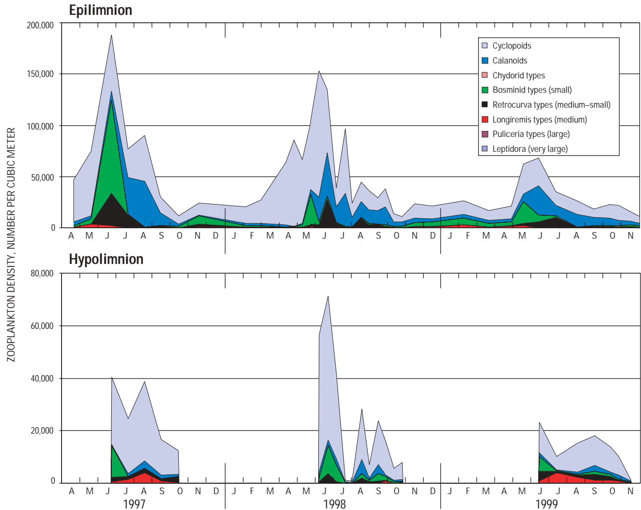
Figure 13. Zooplankton populations in the epilimnion and hypolimnion of Geneva Lake, Wisconsin (West Bay), April 1997 through November 1999.
