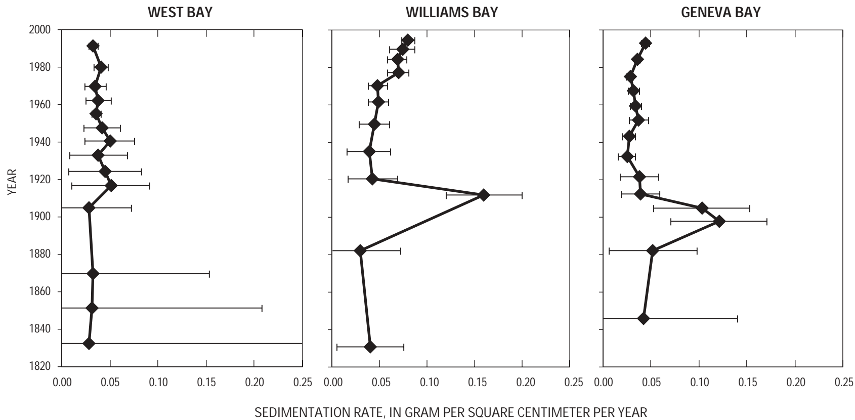
Figure 38. Sedimentation rates from three sediment cores from Geneva Lake, Wisconsin, 1830 to 1995. [Error bars are plus and minus 1 standard deviation (obtained from Garrison, 2000.)]
