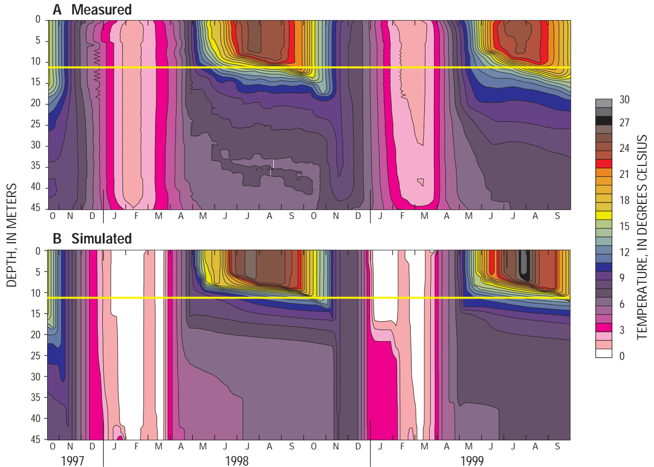
Figure 26. Water temperature distribution in Geneva Lake, Wisconsin, October 17, 1997 through September 30, 1999: (A) measured data, and (B) simulated data from the Dynamic Lake Model. (Yellow lines on plots represent the depth of the thermocline.)
