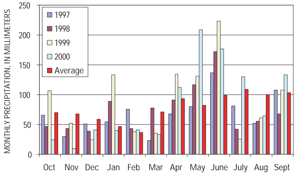
Figure 4. Monthly air temperature (departure from 30-year normal, 1961–90) and precipitation for Lake Geneva, Wisconsin, water years 1997–2000.
