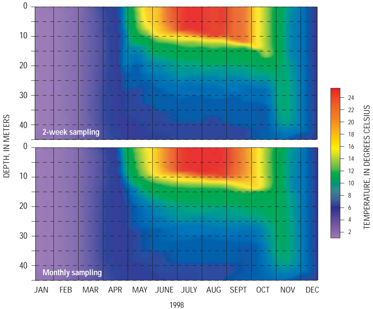
Figure 3. Water temperature distribution in Geneva Lake, Wisconsin, in 1998 based on 2-week and monthly sampling.
