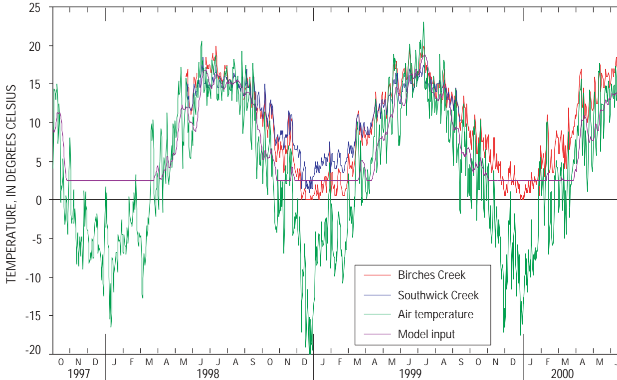
Figure 16. Water temperatures measured in Southwick and Birches Creeks and air temperatures measured at Lake Geneva, Wisconsin, October 1997 through June 2000. (Water temperatures used in model simulations also are shown.)
