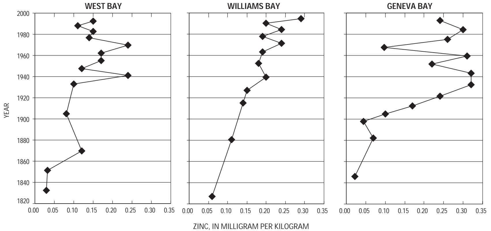
Figure 39. Profiles of zinc concentrations in three sediment cores from Geneva Lake, Wisconsin, 1830 to 1995 (obtained from Garrison, 2000).
