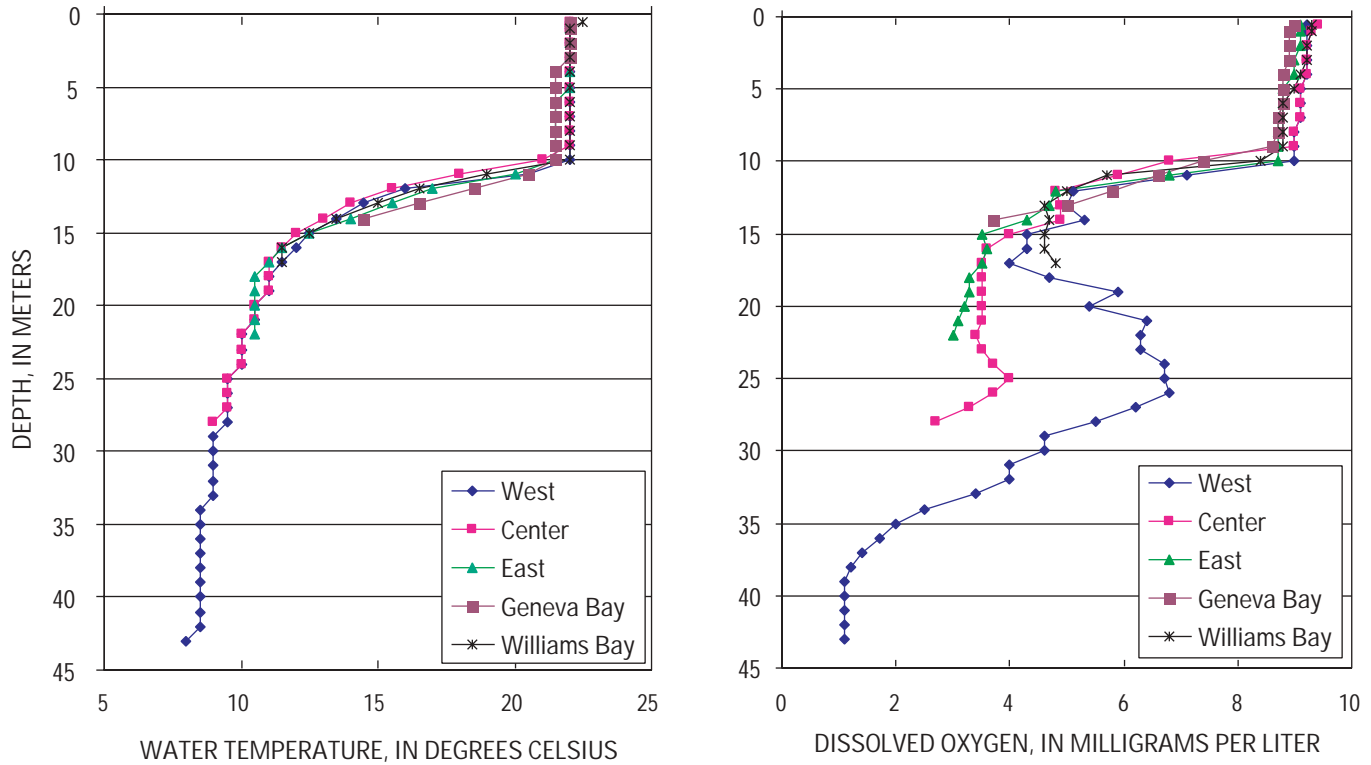
Figure 2. Temperature and dissolved oxygen profiles throughout Geneva Lake, Wisconsin, August 19, 1997.
