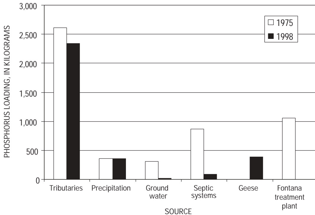
Figure 31. Comparison of phosphorus loading from individual sources in water year 1998 with that estimated for calendar year 1975 for Geneva Lake, Wisconsin. (Data for 1975 from Southeastern Wisconsin Regional Planning Commission, 1985.)
