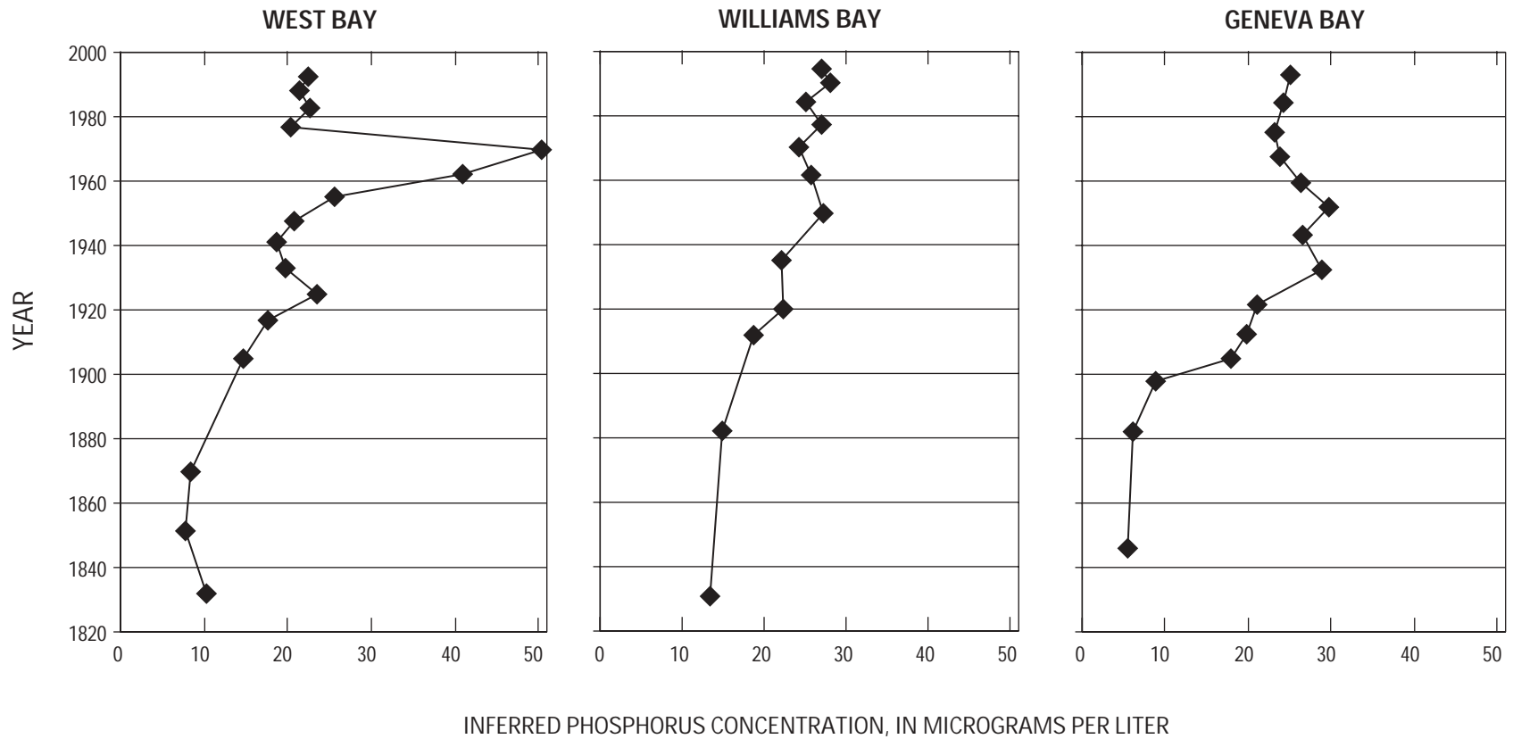
Figure 40. Inferred phosphorus concentrations for Geneva Lake, Wisconsin, 1830 to 1995, based on changes in diatom populations from three cores from the lake (obtained from Garrison, 2000).
