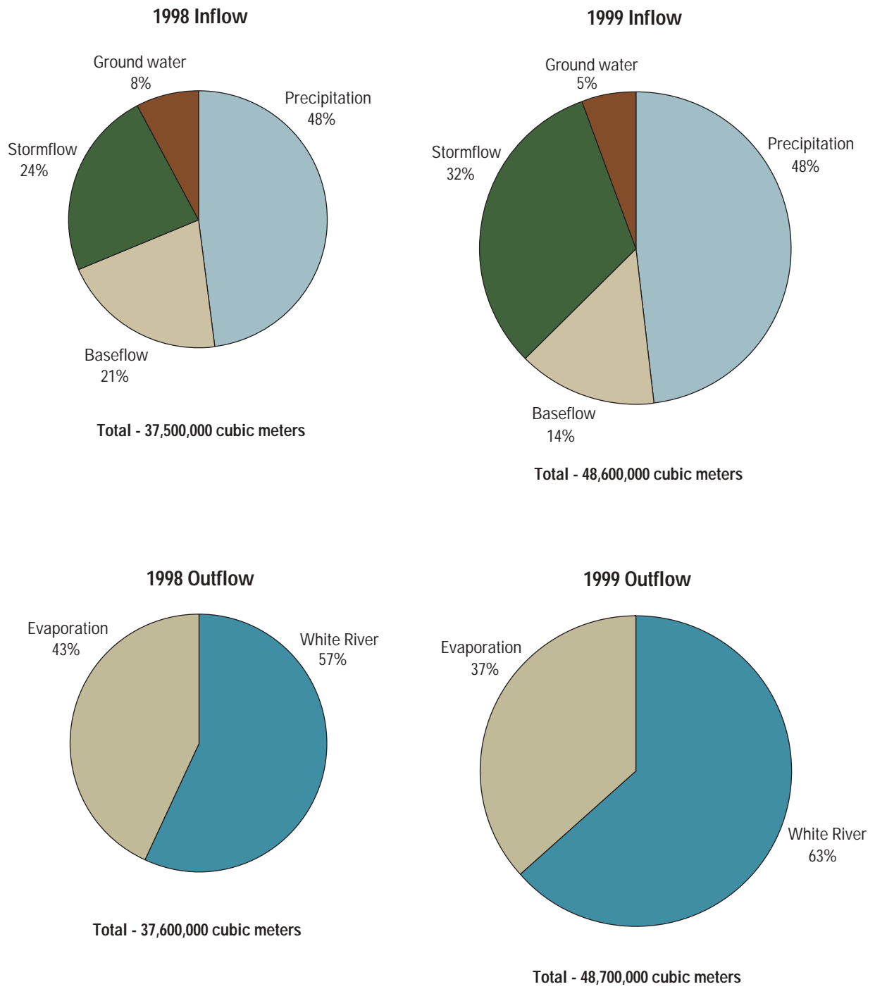
Figure 28. Hydrologic budget for Geneva Lake, Wisconsin, water years 1998 and 1999. [%, percent]
