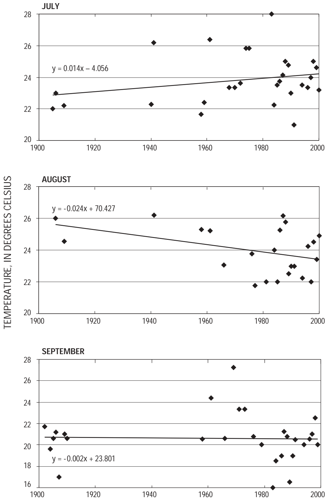
Figure 33. Near-surface water temperatures measured in Geneva Lake, Wisconsin, during July, August, and September, 1902 to 2000. (Trend lines are based on linear regression through the data.)
