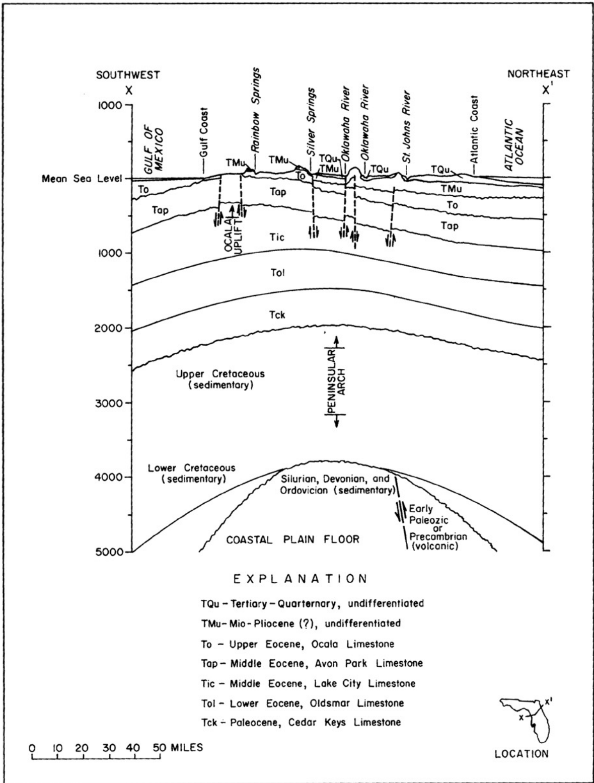
Figure 10. Geologic section (X-X') of north Peninsular through area of Cross-Florida Barge Canal.
