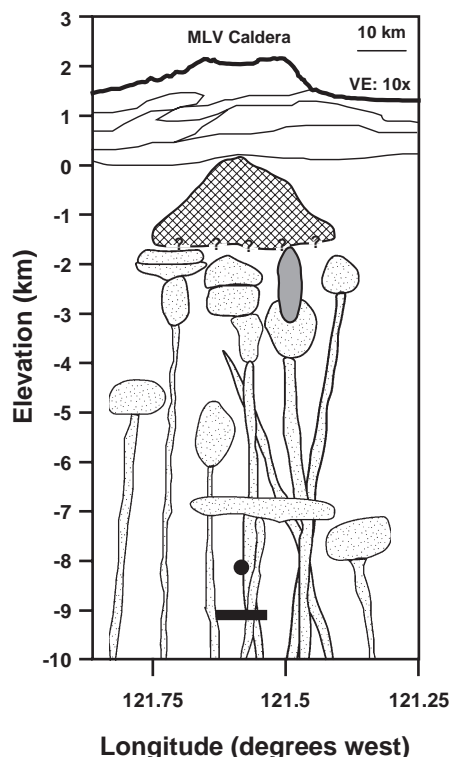
Fig. 2. Schematic E–W cross section model of the MLV subsurface, based in part on that of Donnelly-Nolan (1988). Vertical exaggeration is 10 \times . Felsic and mafic lava flows of the early MLV shield underlie the caldera (Donnelly-Nolan, 1988). A large, cone-shaped granodiorite intrusion at depths of about 1.5–4 km (cross-hatched pattern) has been identified in drill core and by geophysical investigations (Finn and Williams, 1982; Zucca et al., 1986; Fuis et al., 1987; Lowenstern, 1999; Lowenstern et al., 2003). The only area of possible liquid melt as deduced from seismic data (Evans and Zucca, 1988; Chiarabba et al., 1995) occurs at 4–6 km beneath the eastern caldera rim (gray shaded area), which was the site of the most recent volcanic eruption. An extensive complex of solidified mafic and felsic intrusive bodies (dotted pattern) is inferred beneath the granodiorite intrusion to below 10 km depth (Evans and Zucca, 1988; Lowenstern et al., 2003). The best-fitting point and dislocation sources of volume loss to leveling data determined by Dzurisin et al. (2002) are shown as a black circle and rectangle, respectively. Note that both sources are significantly below the modeled location of magma based on interpretation of seismic data (Evans and Zucca, 1988; Chiarabba et al., 1995).
