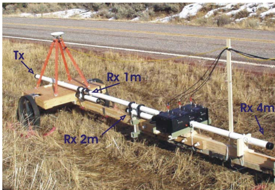
Figure 5. Photo. EM31-3 mounted on low metal content trailer.
