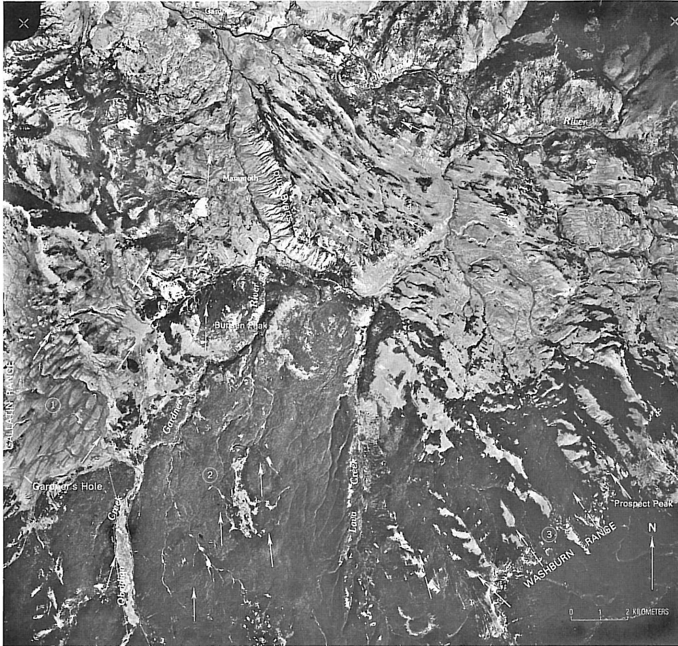
FIGURE 21.—Convergence of ice streams towards Gardiner to form the northern Yellowstone outlet glacier. 1, Drumloid topography in Gardners Hole (also frontispiece) and adjacent areas formed by northeasterly to northerly flow from the Gallatin Range icecap and the plateau icecap between the Gallatin and Washburn Ranges. 2, Northerly flow between Obsidian and Lava Creeks left striations and basalt erratics on Bunsen Peak. 3, Striations and scour features cross the crest of the northwestern part of the Washburn Range. 4, Glacial-scour features on Mount Everts and adjacent uplands indicate flow swinging from westerly to northwesterly. Dot in arrow indicates striations observed on the ground. High-altitude aerial photograph by NASA, 1969.
