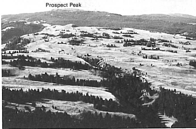
FIGURE 40.—Oblique view south along a melt-water channel known as "the cut." The channel transects ice-streaming, molding and scouring features (left to right lineation of topography) formed during full-glacial time. The channel is as much as 60 m deep and was occupied by the ice-marginal Yellowstone River as the glacier receded from the Deckard Flats position. Extensive deglaciation had occurred by the time ice-marginal melt waters flowed through "the cut", for the ice surface was more than 600 m higher when it striated Prospect Peak. (See also fig. 26.)
