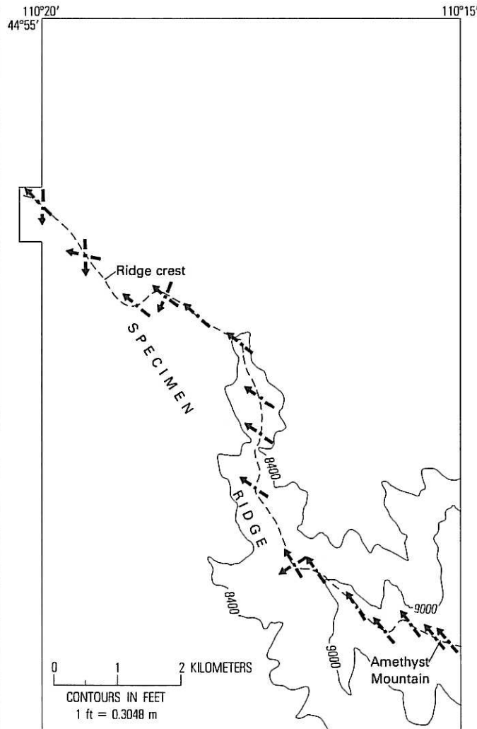
FIGURE 29.—Orientation of striations (arrows) along the crest of Specimen Ridge. Dots are localities of observation. Above an altitude of 2,750 m (9,000 ft) directional indicators (figs. 5, 28) indicate flow to the northwest. Below the 9,000-foot contour, geometric relations indicate that southerly striations are younger than the northwesterly ones. Also, erratics of Paleozoic limestone and Precambrian rocks below the 9,000-foot contour indicate an incursion of ice from the north, which occurred during the Deckard Flats readjustment. Base from U.S. Geological Survey 1:62,500 Tower Junction, 1959.
