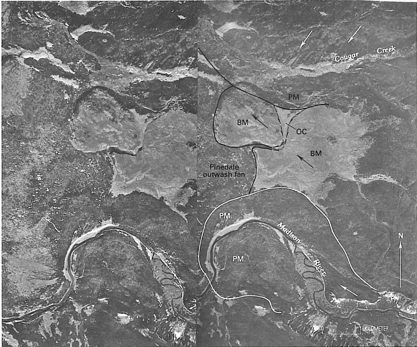
FIGURE 33.—Pinedale terminal moraines along Cougar Creek and the Madison River. As shown in figure 10 (locs. 8 and 9), a thin soil with little or no loess is present on the Pinedale moraines, PM. Arrows, ice flow direction. Note glacial-scour features indicating Pinedale flow to the southwest, oblique to Cougar Creek. Outwash channel, OC, is bracketed by single-barb arrows and extends southwestward from Pinedale moraine. BM, large meadow area, Bull Lake ground moraine and kame gravels mantled by loess. Along Madison River, Pinedale terminal moraines are locally breached by melt-water channels that extend for at least 3 km west of the moraines. Stereo-aerial photographs by AMS, 1954.
