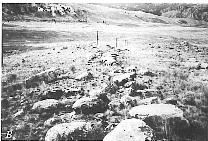
FIGURE 44.—Giant current ripples on midchannel flood bar north of Gardiner, Mont. A , Oblique aerial photograph showing form of bar and pattern of giant current ripples. Flood bar is about 500 m across and 20 m high. Crests of ripples (fig. 45) are about 2 m high and about 15 m apart. Flow was towards the camera. A longitudinal flood bar is shown in the upper right of the photograph. Photograph by J. S. Shelton, 1970. B , Ridges of boulders forming giant current ripples on the midchannel flood bar. The boulders are concentrated on the downstream (right) side of the crest.
