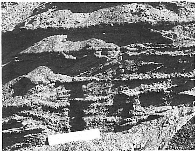
FIGURE 36.—Obsidian-sand-plain sediments. Horizontal beds about 15 cm thick have both subhorizontal and steeply inclined crossbedding. The inclined crossbeds of pea-sized gravel are generally openwork (have no matrix). Scale is 18 cm long. Photograph by W. B. Hamilton, 1959.
