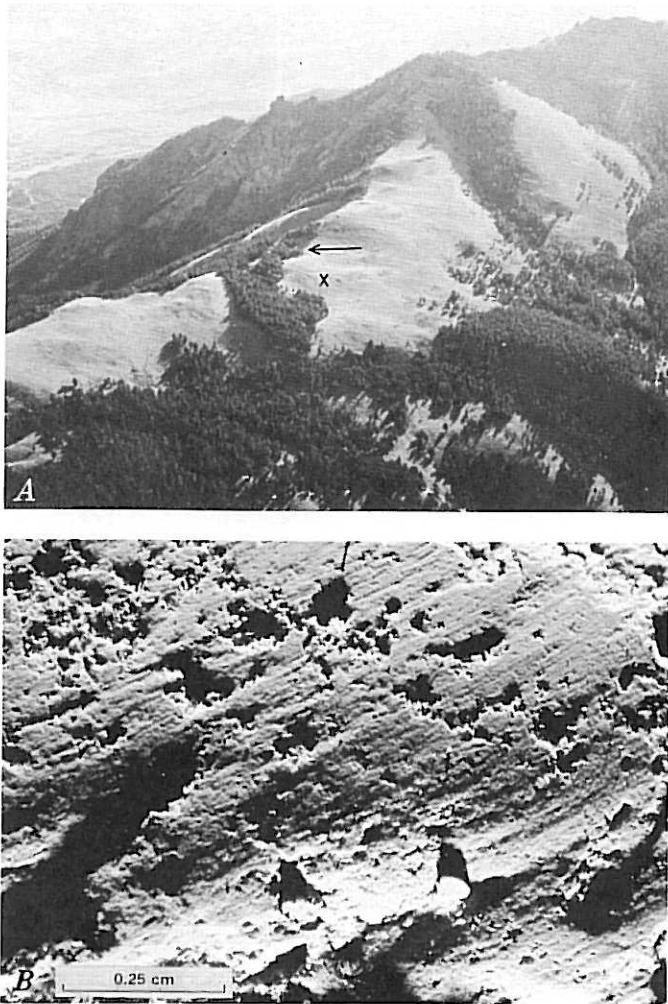
FIGURE 20.—Glacial-scour features on the north spur of Sepulcher Mountain. A, Oblique aerial photograph showing glacial scouring of Eocene bedrock. Scour extends to the top of the grassy area along the ridge crest, 1,100 m above the Yellowstone valley floor. Arrow indicates ice flow from right to left. Photograph by W. B. Hall. X, site of B. Photomicrograph of striated and polished bedrock outcrop showing degree of preservation of striations and polish.
