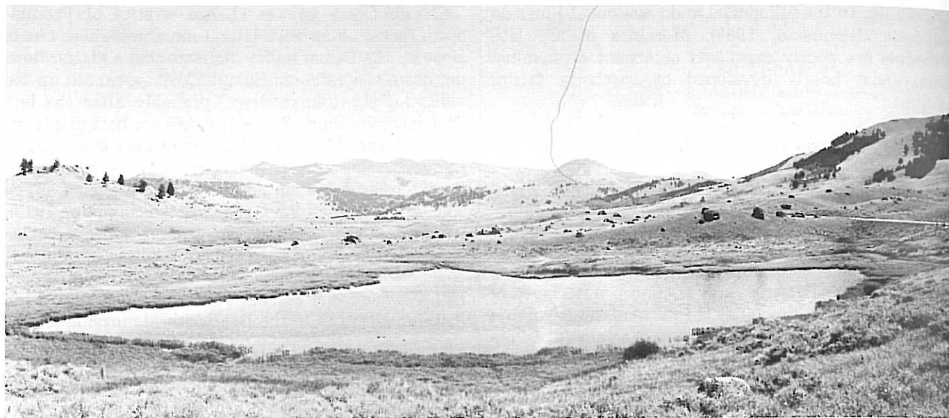
FIGURE 42.—Pond and large erratics in moraines of late Pinedale age near Junction Butte. View is to the southeast; glacier source mostly out of sight in the left distance. Photograph by W. R. Keefer.
