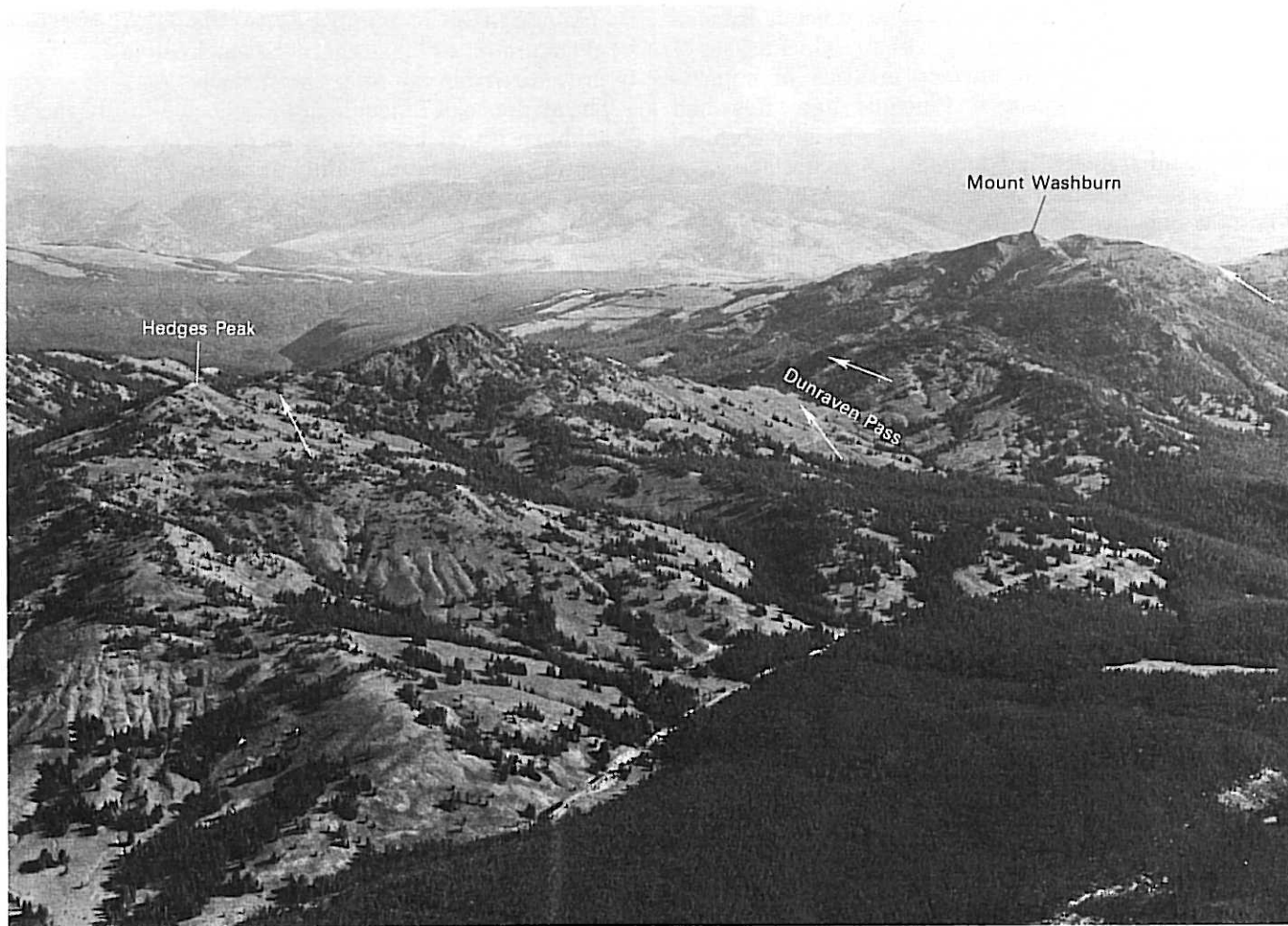
FIGURE 23.—Oblique view, looking northward, of the southeastern part of the Washburn Range, showing its smoothed and rounded appearance. This form is thought to reflect overriding of the entire range by a Pinedale icecap whose axis lay just south of the range (pl. 1A). Bedrock is commonly present within 0.3 m or so of the surface at altitudes above 2,680 m (8,800 ft), and fresh striations indicating glacial flow to the north occur all along the range crest. Dunraven Pass has a glacially rounded, U-shaped form, and striations on the north side of the pass indicate flow northward through the pass. Photograph by W. B. Hall.
