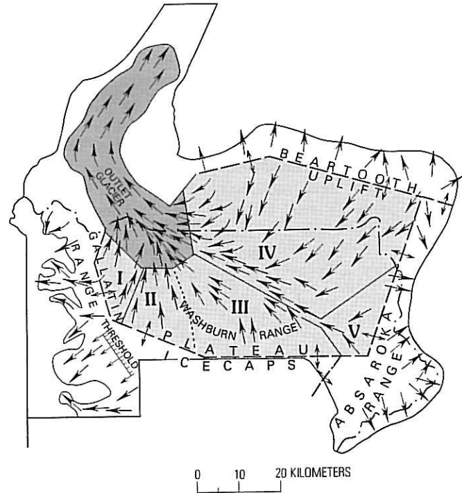
FIGURE 50.—The northern Yellowstone glacier, showing its major source areas and its outlet glacier. Heavy dashed line with double-headed arrows indicates ice divides. Smaller arrows, direction of ice flow. Boundary between areas II and III is dotted to indicate these two areas are both part of the plateau icecap.
