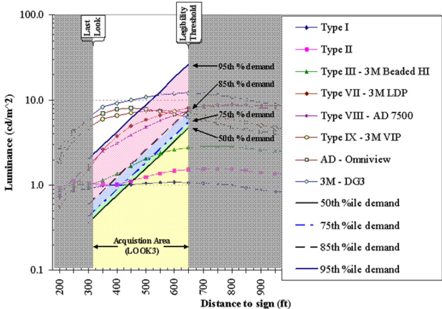
Figure 2. Computer evaluation of supply and demand curves for overhead guide sign mounted 25-feet high, centered on travel lane with no tilt, illuminated by UMTRI 2004 headlamp and viewed from NCHRP 4-29 heavy vehicle.
