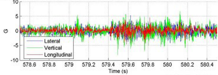
File 061805_24.AB3, Location = 579.5 s, Brake Mount Tube Accelerations W/ABTEC/SAB-W/ABCO Test Axle
