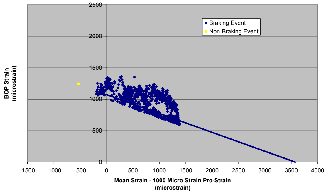
Figure 3.72. Mean Strain versus Alternating Strain, Center WABTEC/SAB-WABCO Supplied Brake Disc, Spokes 6 and 3–June 17, 2005
