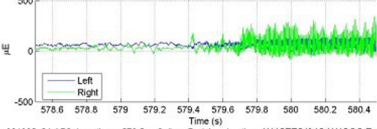
File 061805_24.AB3, Location = 579.5 s, Caliper Pad Accelerations W/ABTEC/SAB-W/ABCO Test Axle
