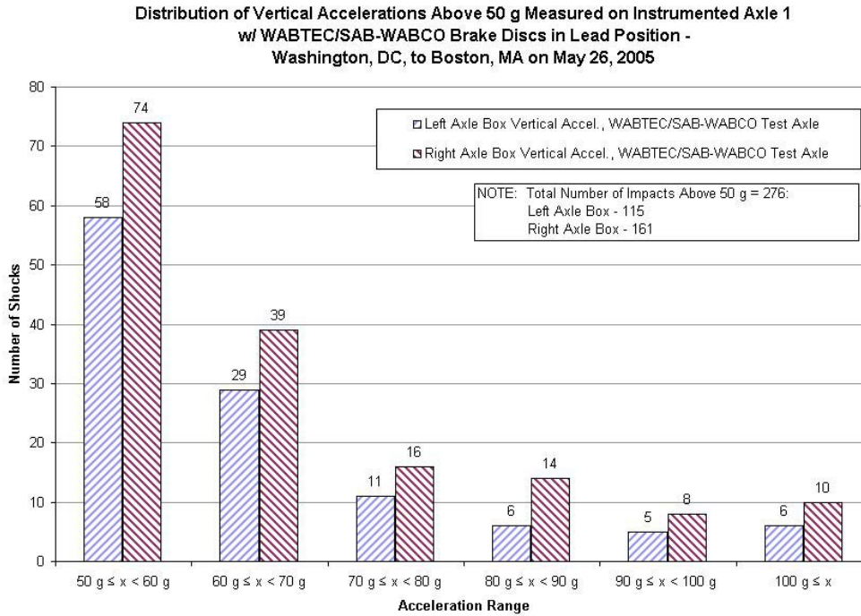
Figure 3.25a. Distribution of Vertical Accelerations Above 50 g Measured on Instrumented Axle 1 with WABTEC/SAB-WABCO Supplied Brake Discs in Lead Position—Washington, DC, to Boston, MA, on May 26, 2005
