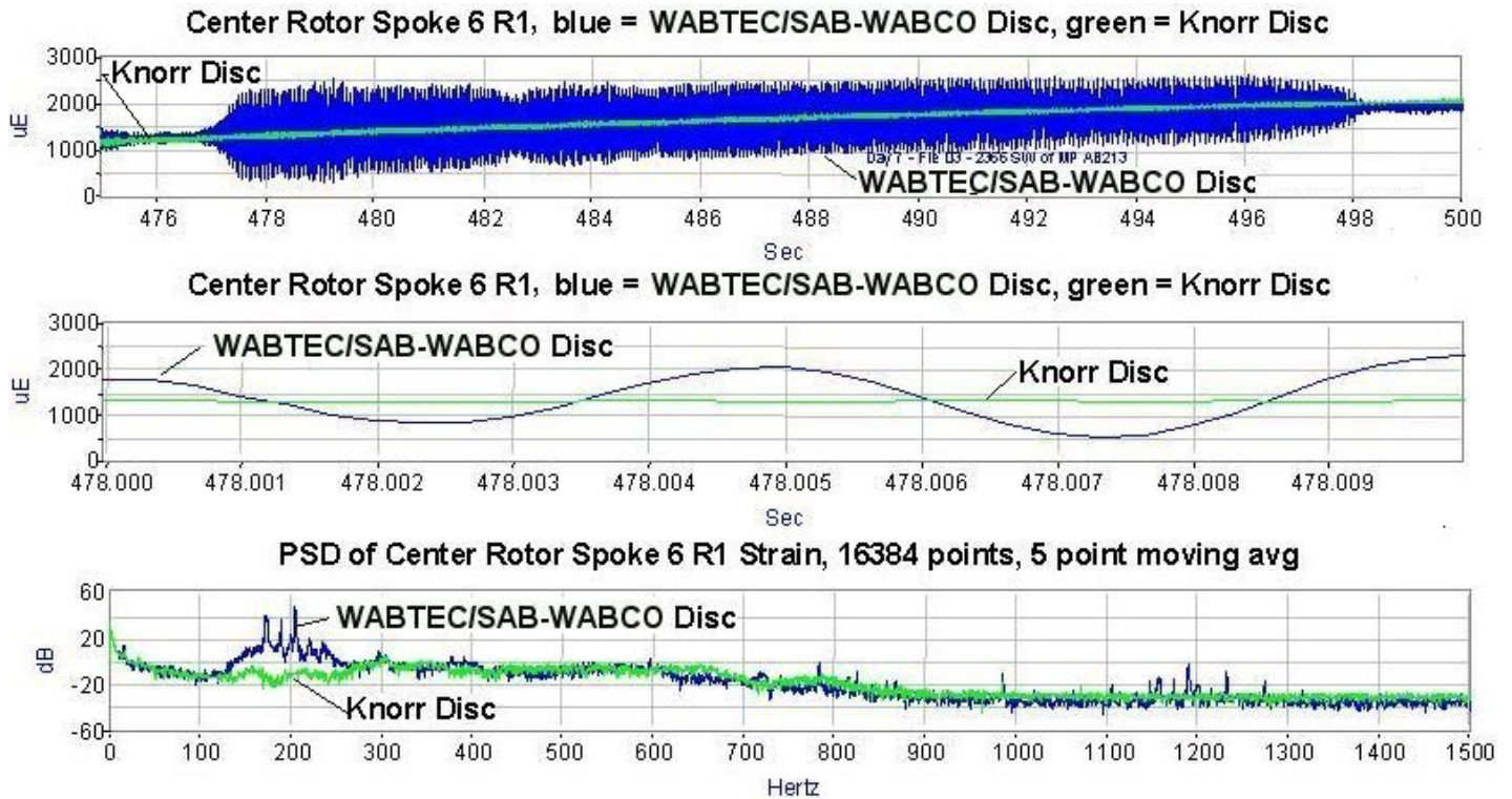
Figure 3.50. Comparison of WABTEC/SAB-WABCO Supplied Disc and Knorr Disc During a Brake Application From 116 MPH with Sustained Oscillations (File 061805_03.AB3)–June 18, 2005
