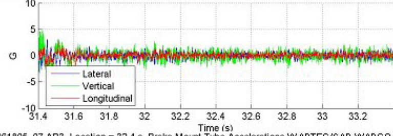
File 061805_07_AB3, Location = 32.4 s, Brake Mount Tube Accelerations W/ABTEC/SAB-W/ABC0 Test Axle
