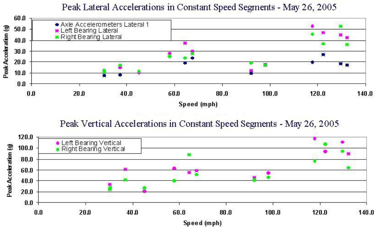
Figure 3.27. Peak Lateral and Vertical Accelerations Observed in Near-Constant Speed Segments as a Function of Speed—May 26, 2005
