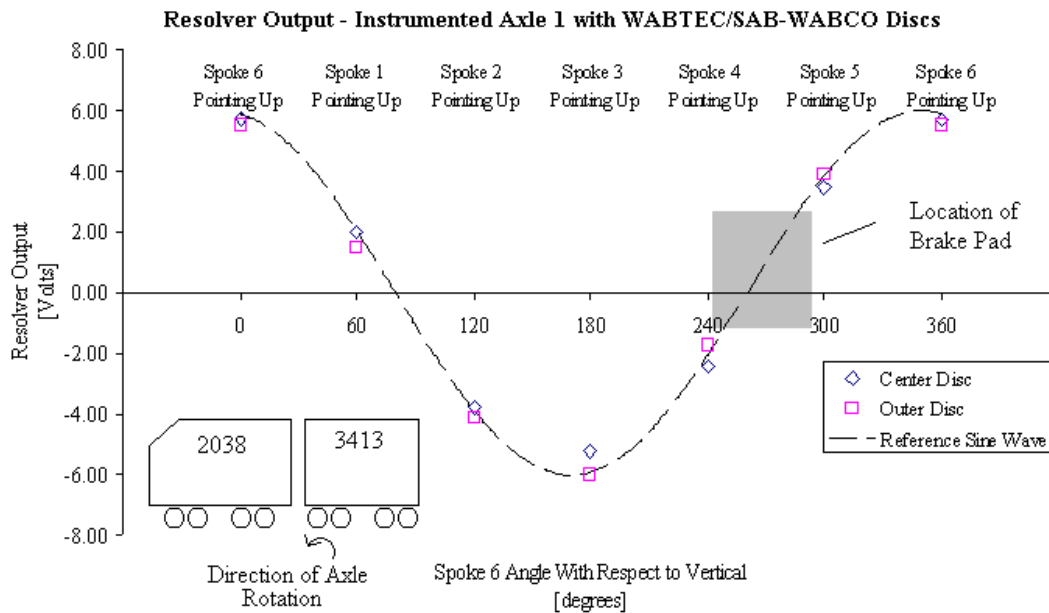
Figure 2.23. Instrumented Spoke Phase Based on Wheel Angular Position, WABTEC/SAB-WABCO Supplied Discs
