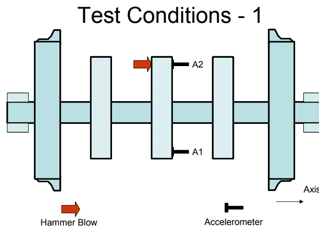
Figure 2.28. Illustration of Typical Setup for Modal Assessment of Brake Discs
