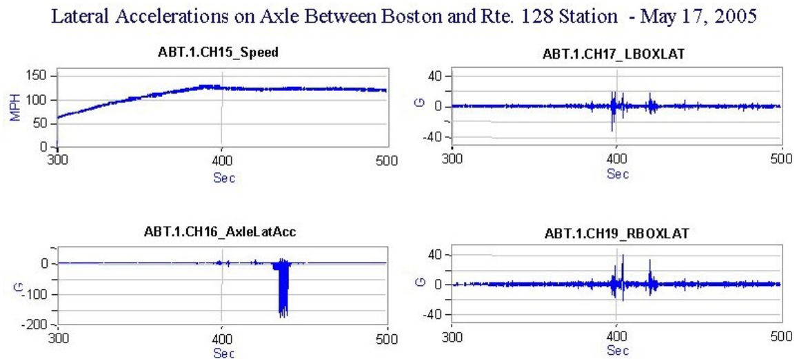
Figure 3.5. Lateral Accelerations Measured on Instrumented Axle 1 Between Boston and Rte 128 Station (File 051705_02.ABT)–May 17, 2005
