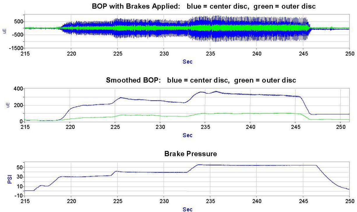
Figure 3.22. Brake Cylinder Pressure and BOP Strains Recorded on WABTEC/SAB-WABCO Supplied Brake Discs During Braking Near MP E17 (File 051705_17.ABT)–May 17, 2005
