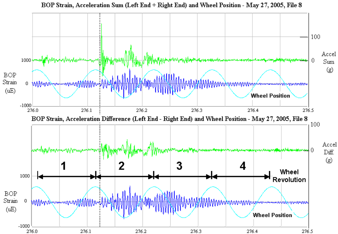
Figure 3.32. BOP Strains on WABTEC/SAB-WABCO Supplied Center Disc Resulting from Vertical Shocks on Both Ends of Test Axle (File 052705_08.AB2)–May 27, 2005
