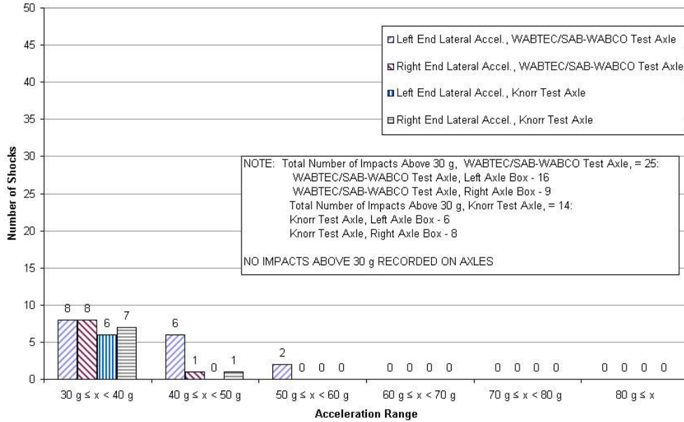
Figure 3.47b. Distribution of Lateral Accelerations Above 30 g Measured on Instrumented Axles 1 and 2 in Lead Position—Boston, MA, to Washington, DC, on June 18, 2005
