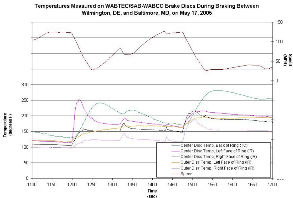
Figure 3.20. Extreme Temperature Measurements Made During Testing Between Wilmington, DE, and Baltimore, MD–May 17, 2005
