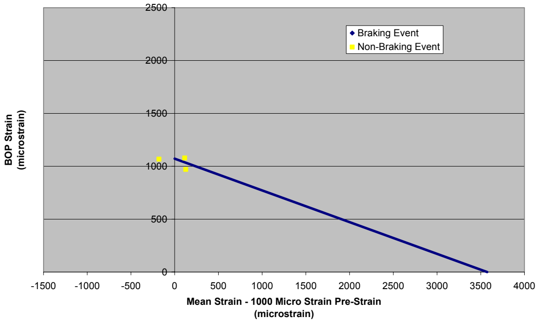
Figure 3.68. Mean Strain versus Alternating Strain, Center and Outer WABTEC/SAB-WABCO Supplied Brake Discs, Spoke 6–May 16, 2005
