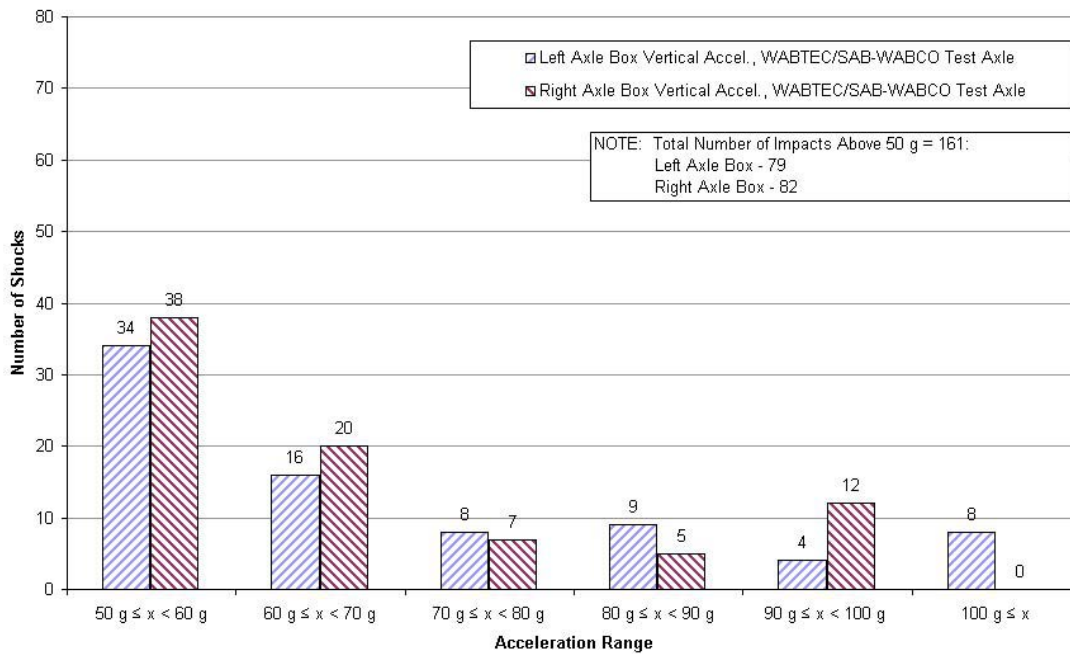
Figure 3.6b. Distribution of Vertical Accelerations Above 50 g Measured on Instrumented Axle 1 with WABTEC/SAB-WABCO Supplied Brake Discs in Lead Position-- Boston, MA, to Washington, DC, on May 17, 2005
