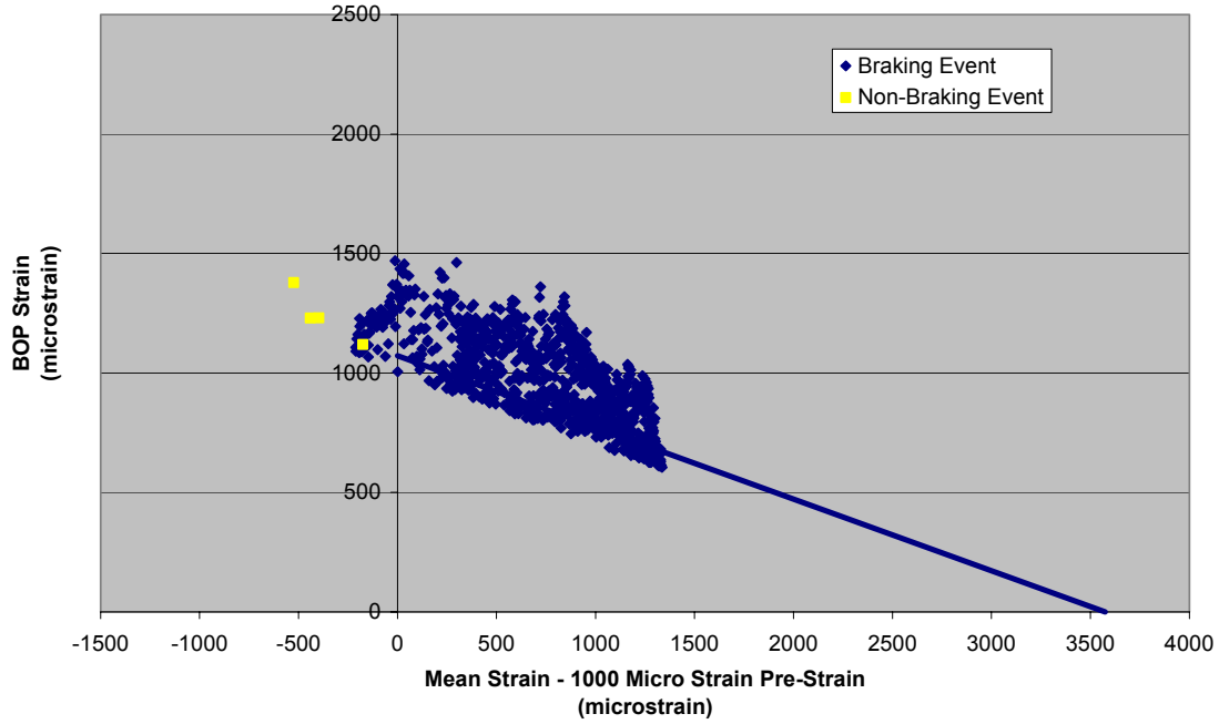
Mean Strain vs. Alternating Strain, Center WABTEC/SAB-WABCO Disc, Spoke 3 - June 17, 2005
