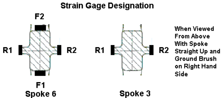
Figure 3.29. Designation of Strain Gages Used on Spoke 6 and Spoke 3 of Instrumented Center WABTEC/SAB-WABCO Supplied Disc During Phase 2 Testing
