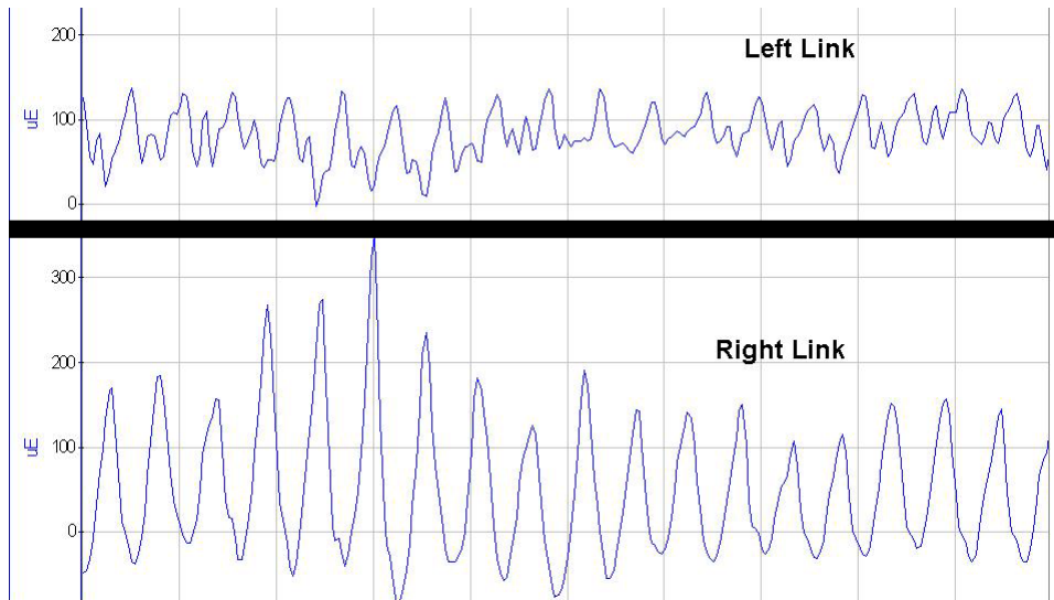
Figure 3.64. Strains Recorded on Caliper Links During Sustained Oscillations of WABTEC/SAB-WABCO Supplied Brake Disc While Braking (File 061805_24.AB3)–June 18, 2005
