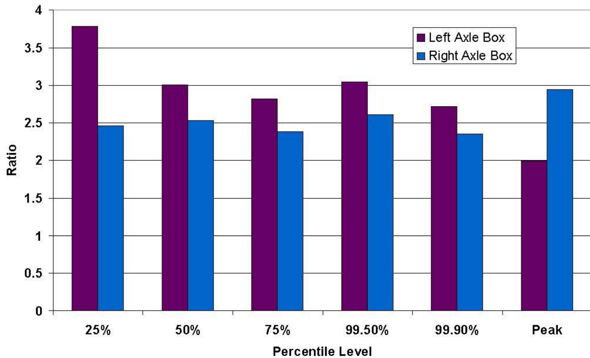
Figure 3.28. Vertical to Lateral Acceleration Ratios Determined for Data Collected in Near-Constant Speed Segments at 122 MPH–May 26, 2005
