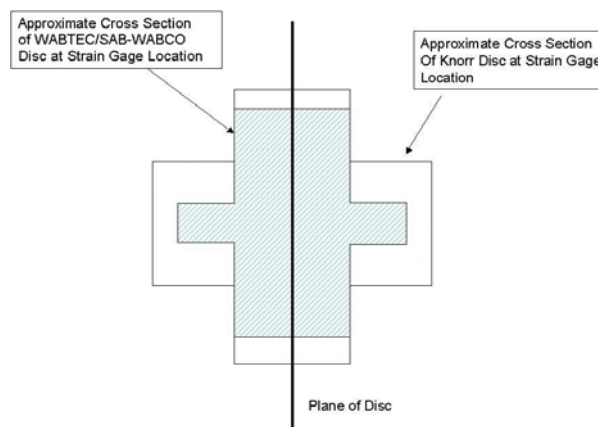
Figure 3.51. Comparison of Cross Sections of Spokes from WABTEC/SAB-WABCO Supplied and Knorr Brake Discs
