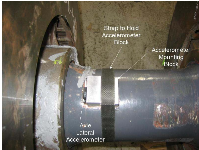
Figure 2.12. Lateral Accelerometer Mounted Near Center Disc on WABTEC/SAB-WABCO Test Axle During Phase 1 of Acela Brake Disc Study
