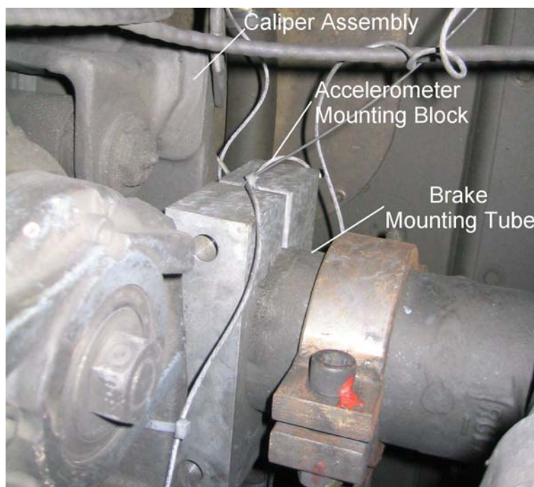
Figure 2.16. Tri-Axial Accelerometer Mounted on Brake Mounting Tube Over WABTEC/SAB-WABCO/Knorr Test Axles, Phase 3 of Acela Brake Disc Study
