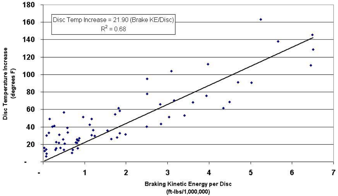
Figure 3.56. Comparison of Disc Temperature Changes versus Dissipated Kinetic Energy for Knorr and WABTEC/SAB-WABCO Supplied Brake Discs—June 18, 2005
