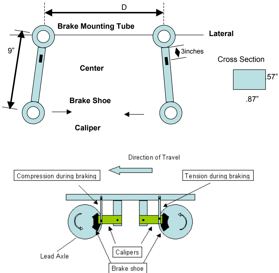
Figure 3.61. Illustration of Instrumented Brake Links and Locations within Truck
