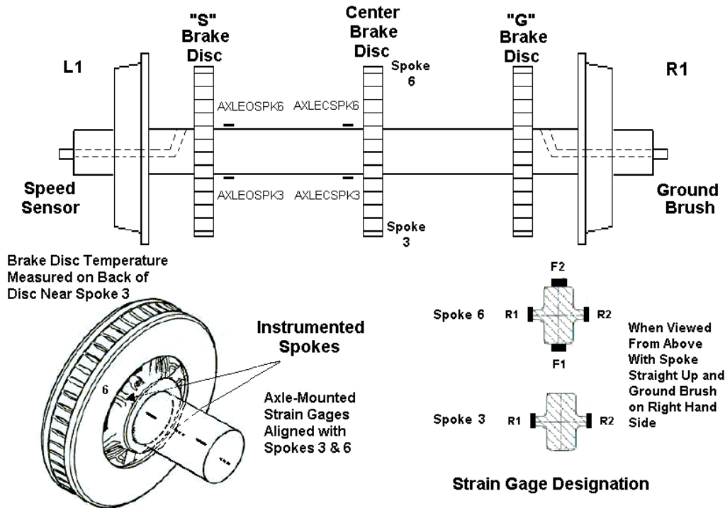
Figure 2.6. Location of Strain Gages on WABTEC/SAB-WABCO Test Axle During Phase 2 of Study
