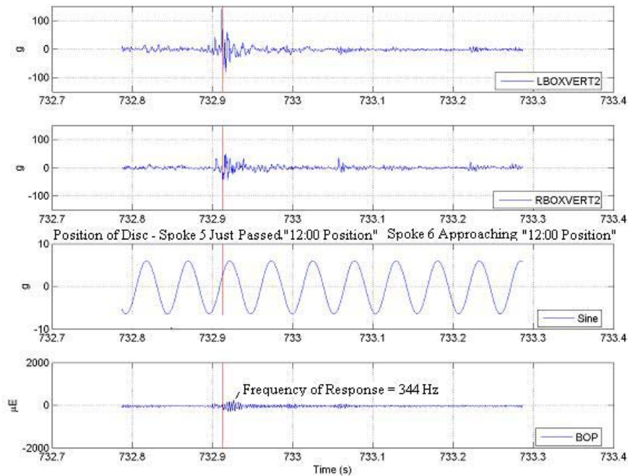
Figure 3.49. Vertical Shock and BOP Spoke Strain Response of Knorr Brake Disc Measured Near Lane Interlocking (File 061805_30.AB3)–June 18, 2005
