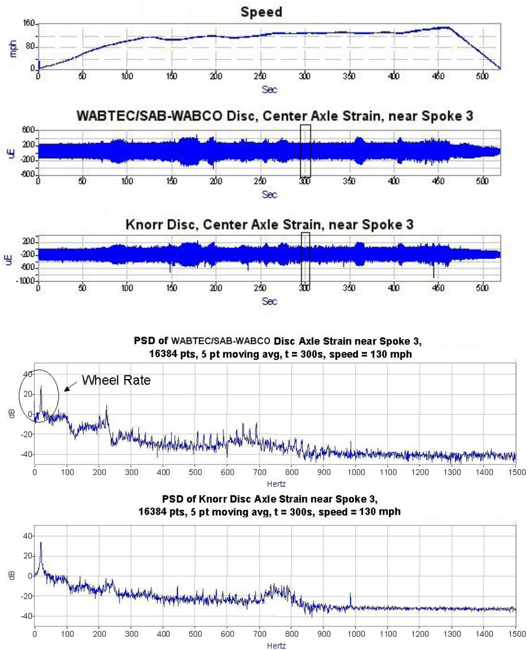
Figure 3.53. PSD of Axle Strains Collected Over Tangent Section of Track (File 061805_03.AB3)–June 18, 2005
