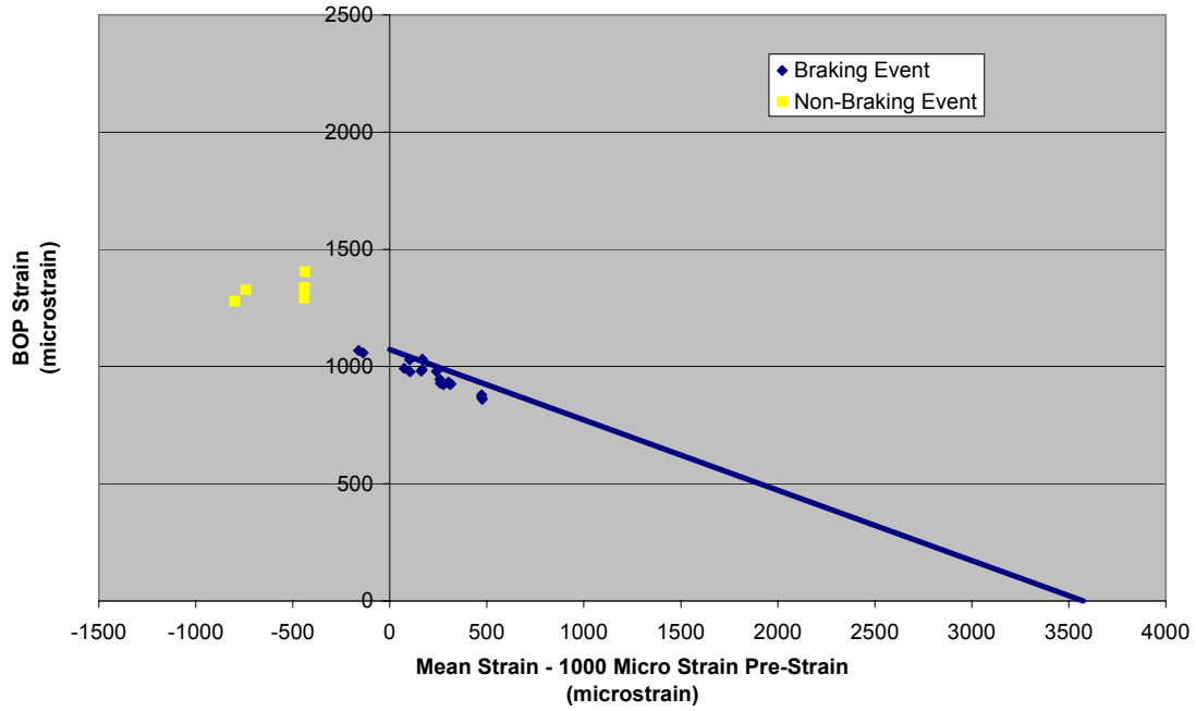
Mean Strain vs. Alternating Strain, Center WABTEC/SAB-WABCO Disc, Spoke 3 - May 26, 2005
