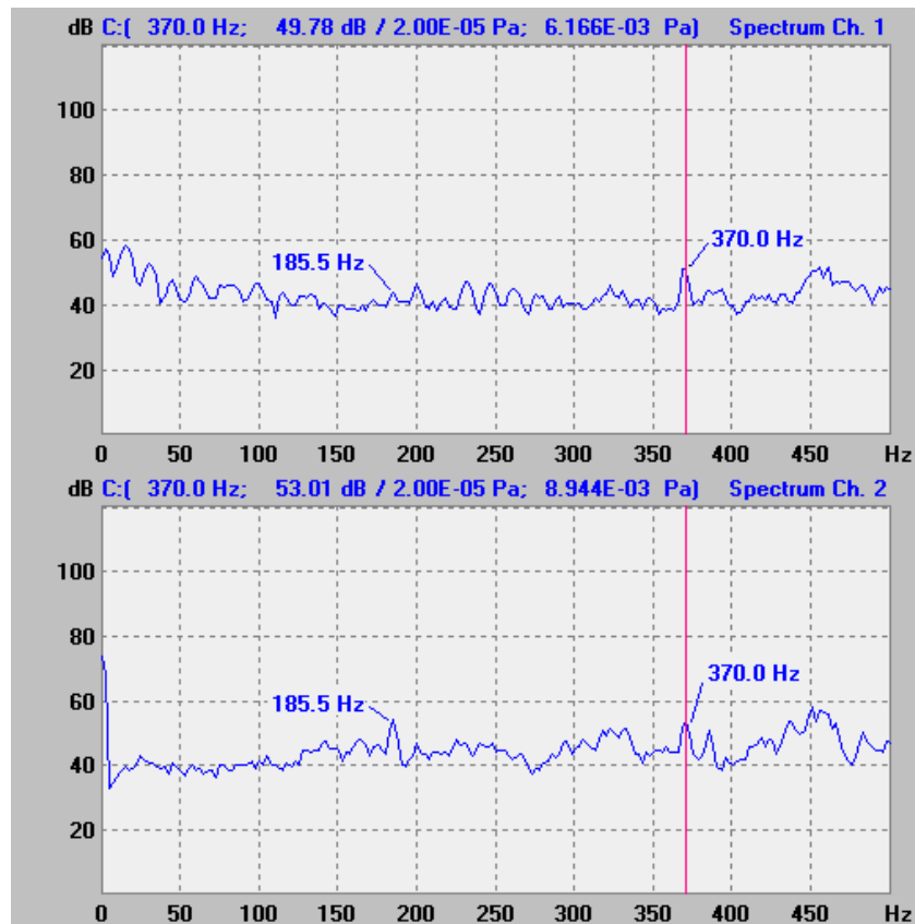
Figure 3.43. Analysis of Sound Recorded During Sustained Oscillations While Braking Near MP AB 179—May 26, 2005
