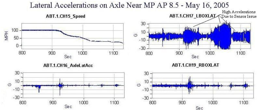
Figure 3.4. Lateral Accelerations Measured on Instrumented Axle 1 Near MP AP 8.5 (File 051605_08.ABT)–May 16, 2005
