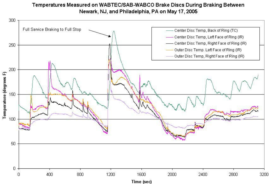
Figure 3.19. Temperature Measurements Made During Testing Between Newark, NJ, and Philadelphia, PA–May 17, 2005
