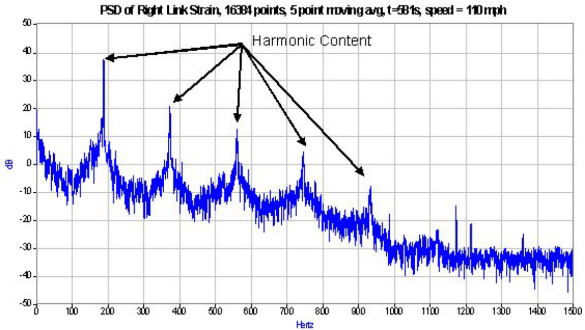
Figure 3.63. Frequency Spectrum of Strains Recorded on Caliper Link During Sustained Oscillations While Braking (File 061805_24.AB3)–June 18, 2005
