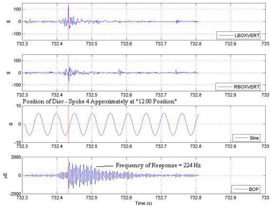
Figure 3.48. Vertical Shock and BOP Spoke Strain Response of WABTEC/SAB-WABCO Supplied Brake Disc Measured Near Lane Interlocking (File 061805_30.AB3)–June 18, 2005
