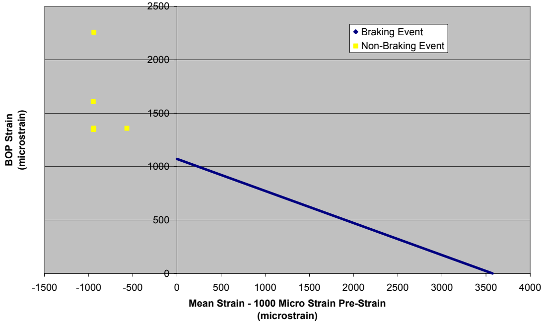
Mean Strain vs. Alternating Strain, Center WABTEC/SAB-WABCO Disc, Spoke 3 - May 27, 2005
