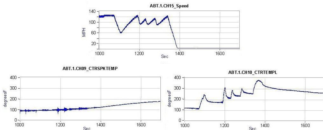
Figure 3.18. Friction Ring and Spoke Temperatures Measured on Center WABTEC/SAB-WABCO Supplied Brake Disc During Brake Applications (File 051605_09.ABT)–May 16, 2005
