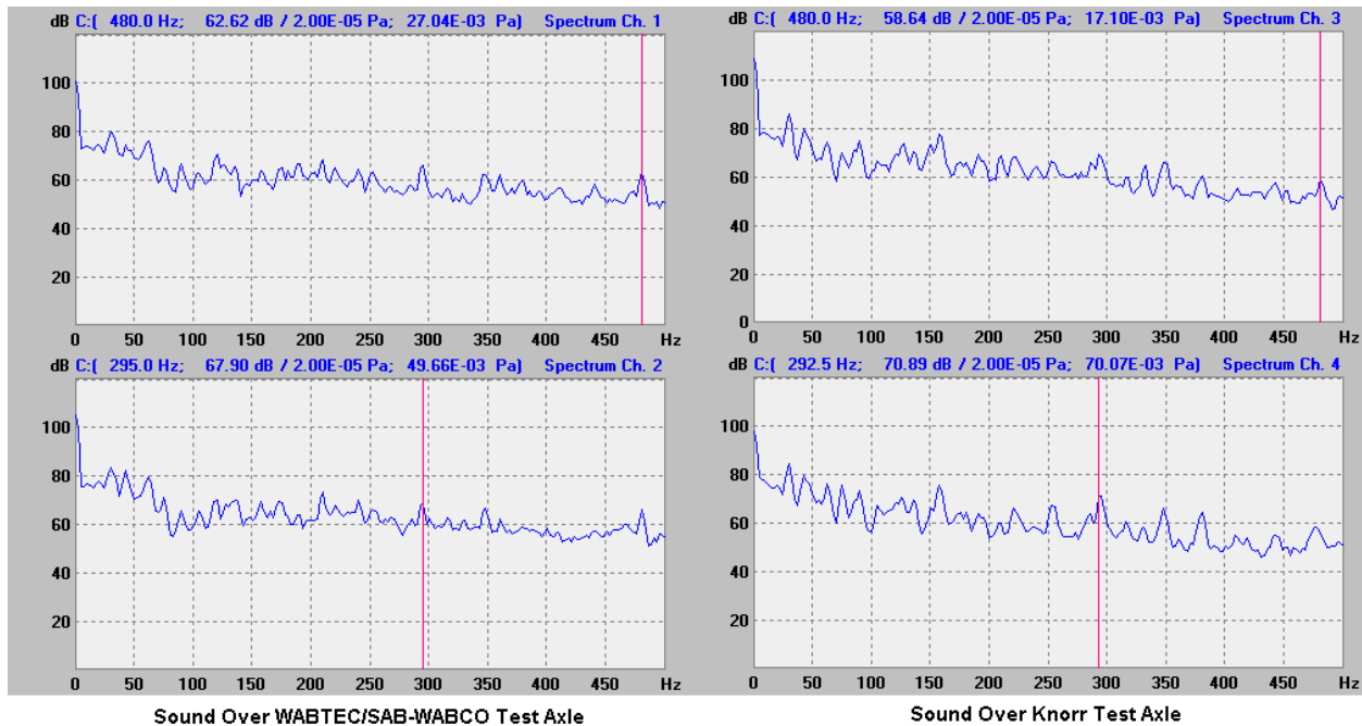
Figure 3.67. Analysis of Sound Recorded Over Both Test Axles During Mild Case of Sustained Oscillations on WABTEC/SAB-WABCO Supplied Disc During Braking Near MP AB 179–June 17, 2005
