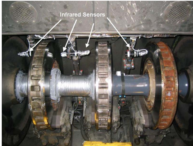
Figure 2.18. Infrared Sensors Mounted to Measure Surface Temperatures of WABTEC/SAB-WABCO Supplied Discs in Center and Outer Positions During Phase 1 of Acela Brake Disc Study
