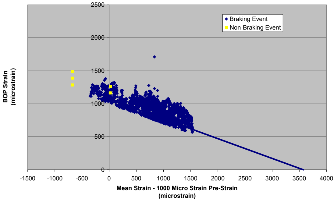
Mean Strain vs. Alternating Strain, Center WABTEC/SAB-WABCO Disc, Spoke 3 - June 18, 2005
