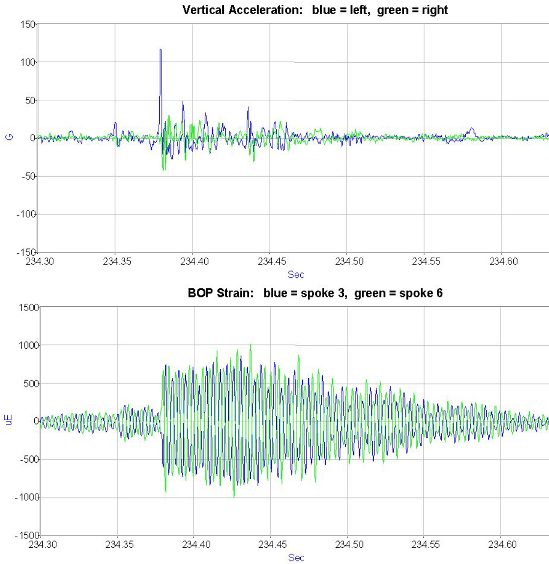
Figure 3.30. Vertical Shock and BOP Strains Recorded on Center WABTEC/SAB-WABCO Supplied Brake Disc During Phase 2 Testing (File 052605_18.AB2)–May 26, 2005
