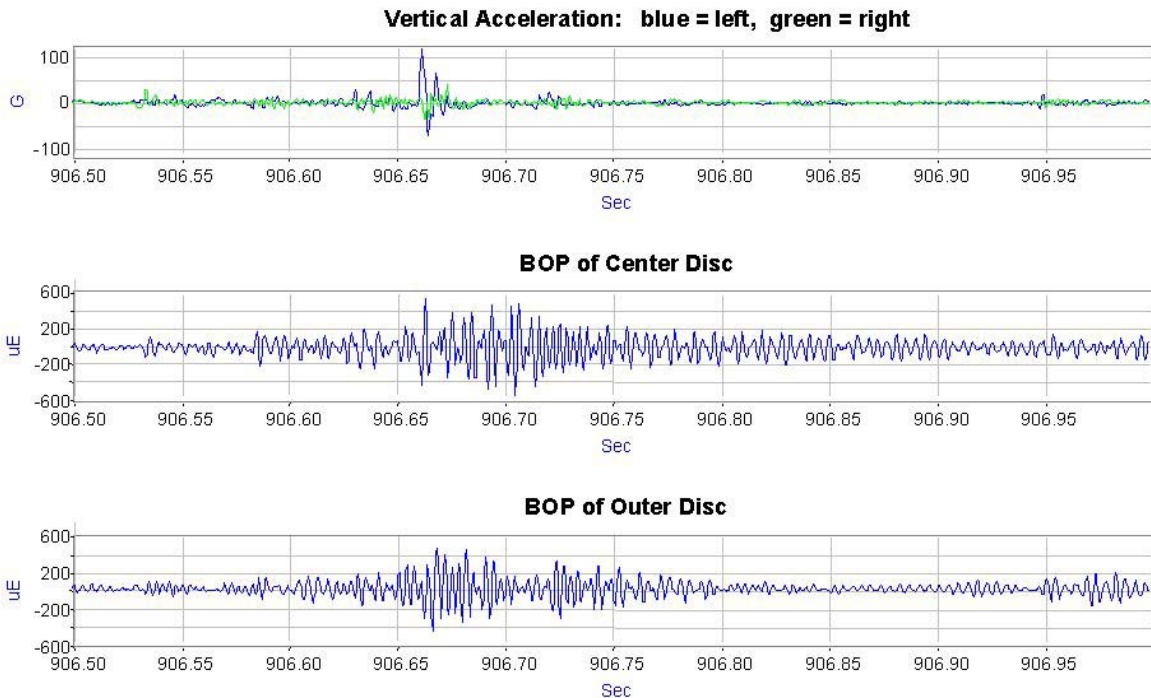
Figure 3.9. Vertical Accelerations and BOP Strains on Spoke 6 of Center and Outer WABTEC/SAB-WABCO Supplied Brake Discs During Vertical Shock (File 051705_19.ABT)– May 17, 2005
