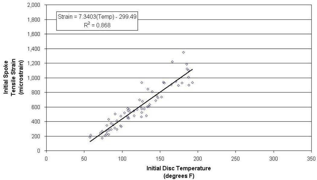
Figure 3.42. Brake Disc Temperature versus Initial Spoke Tensile Strain Before Brake Applications, Center WABTEC/SAB-WABCO Supplied Disc, Spoke 6–May 27, 2005
