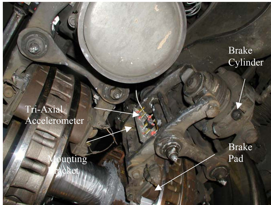
Figure 2.15. Tri-Axial Accelerometer Mounted on Brake Caliper Assemblies Near Brake Pads for WABTEC/SAB-WABCO Test Axle, Phase 1 of Acela Brake Disc Study
