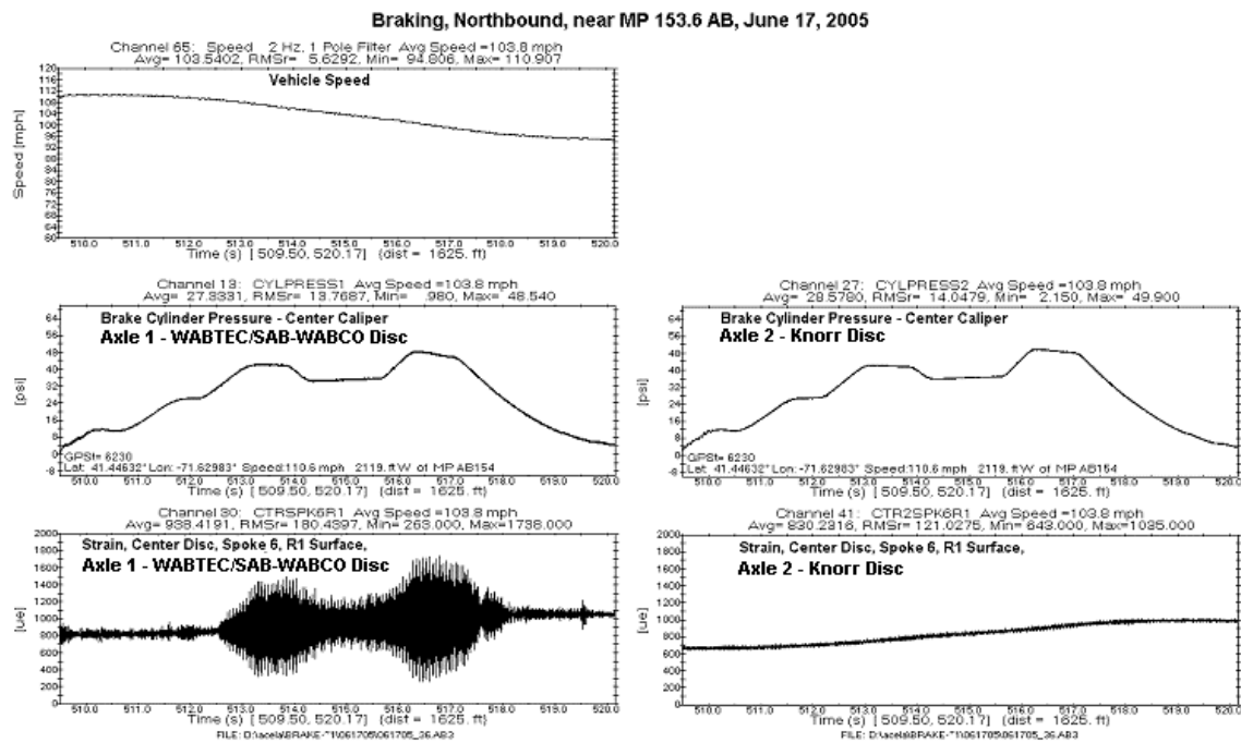
Figure 3.65. Brake Cylinder Pressure and Strains Recorded on Side of WABTEC/SAB-WABCO Supplied and Knorr Brake Disc Spokes During Short Case of Sustained Oscillations (File 061705_36.AB3)–June 17, 2005
