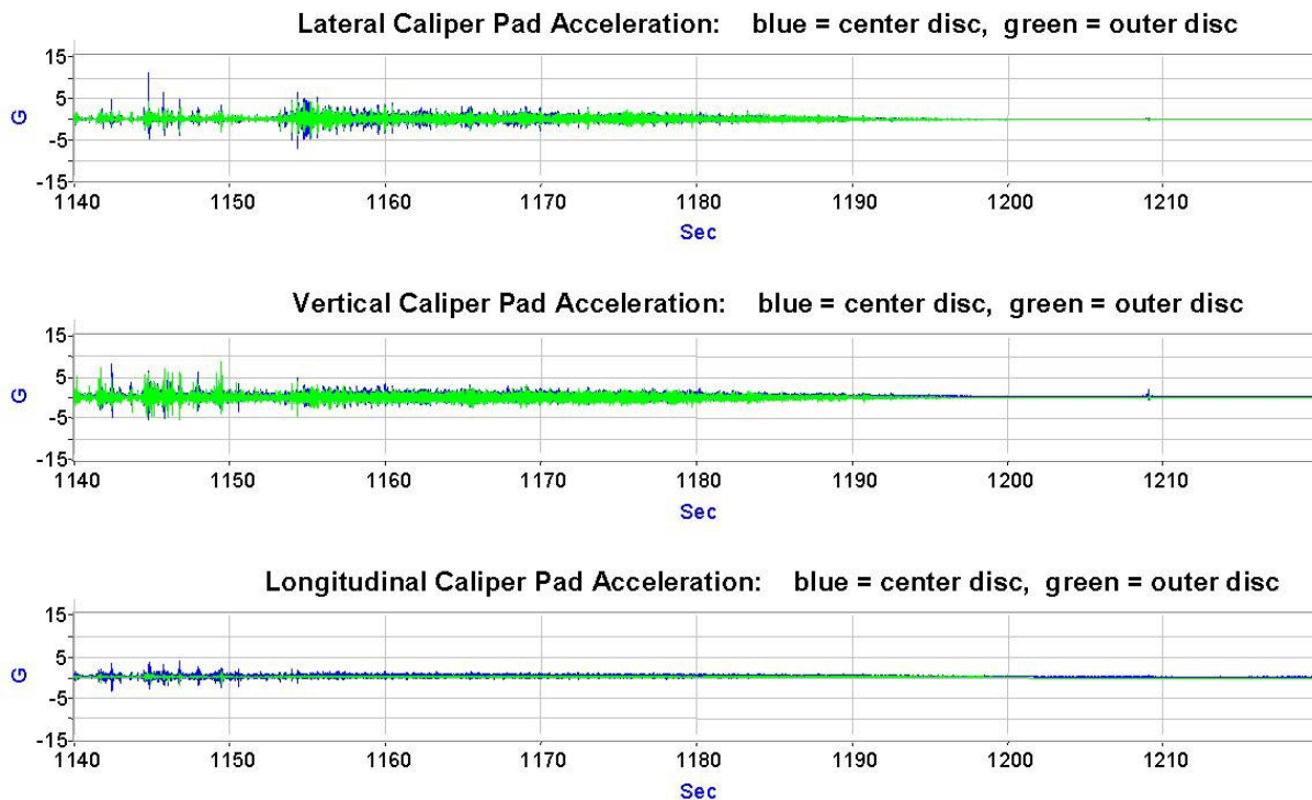
Figure 3.15. Accelerations Measured on Center and Outer Calipers Near Pads During Normal Brake Application (File 051705_19.ABT)–May 17, 2005
