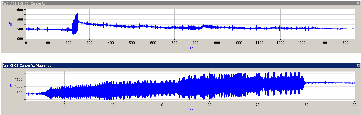
Figure 3.11. Strain Recorded on Gage R1 of Center WABTEC/SAB-WABCO Supplied Brake Disc During Braking Near MP E17 (File 051705_17.ABT)–May 17, 2005
