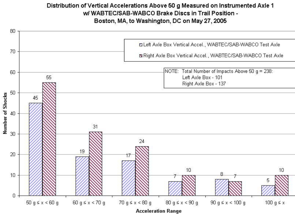
Figure 3.25b. Distribution of Vertical Accelerations Above 50 g Measured on Instrumented Axle 1 with WABTEC/SAB-WABCO Supplied Brake Discs in Trail Position—Boston, MA, to Washington, DC, on May 27, 2005
