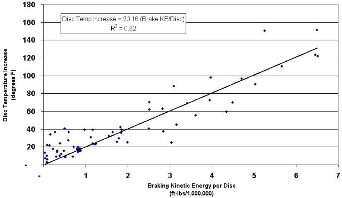
Disc Temperature Change vs. Braking Kinetic Energy/Disc WABTEC/SAB-WABCO Disc - June 18, 2005
