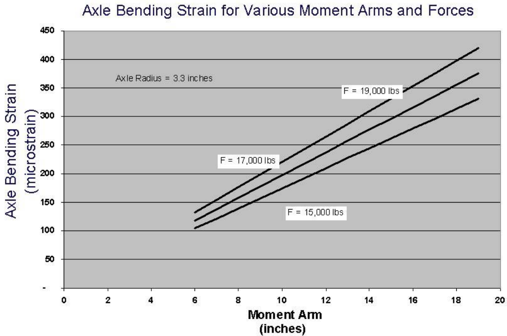
Figure 3.37. Axle Bending Strain as a Function of Bearing Force and Moment Arm
