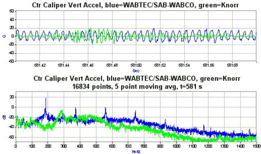
Figure 3.59. Time History and PSD of Brake Caliper Pad Vertical Accelerations During Sustained Oscillations While Braking (File 061805_24.AB3)–June 18, 2005
