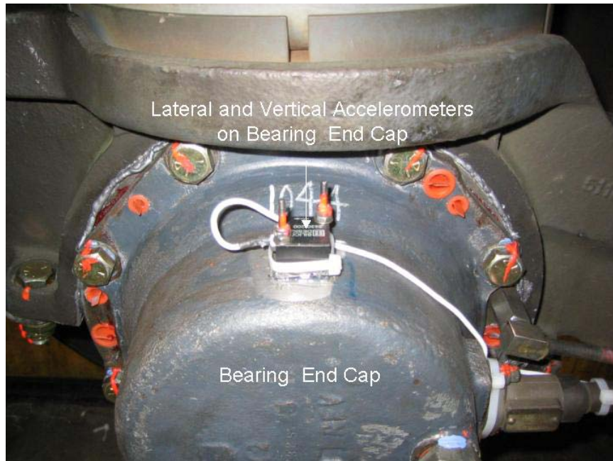
Figure 2.11. Tri-Axial Accelerometer Originally Used to Measure Lateral and Vertical Accelerations on Ends of Test Axle
