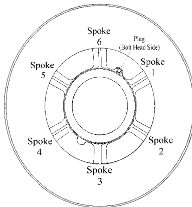
Figure 2.2. Spoke Designations for the WABTEC/SAB-WABCO Supplied Brake Disc
