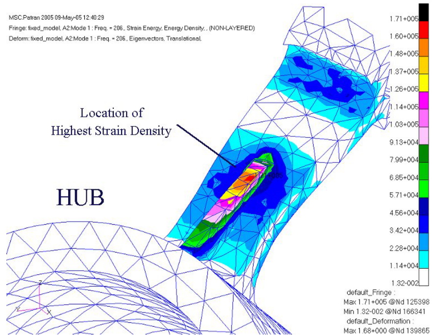
Figure 3.2. Location of Highest Strain for Out-of-Plane Bending Mode Determined from FEA
