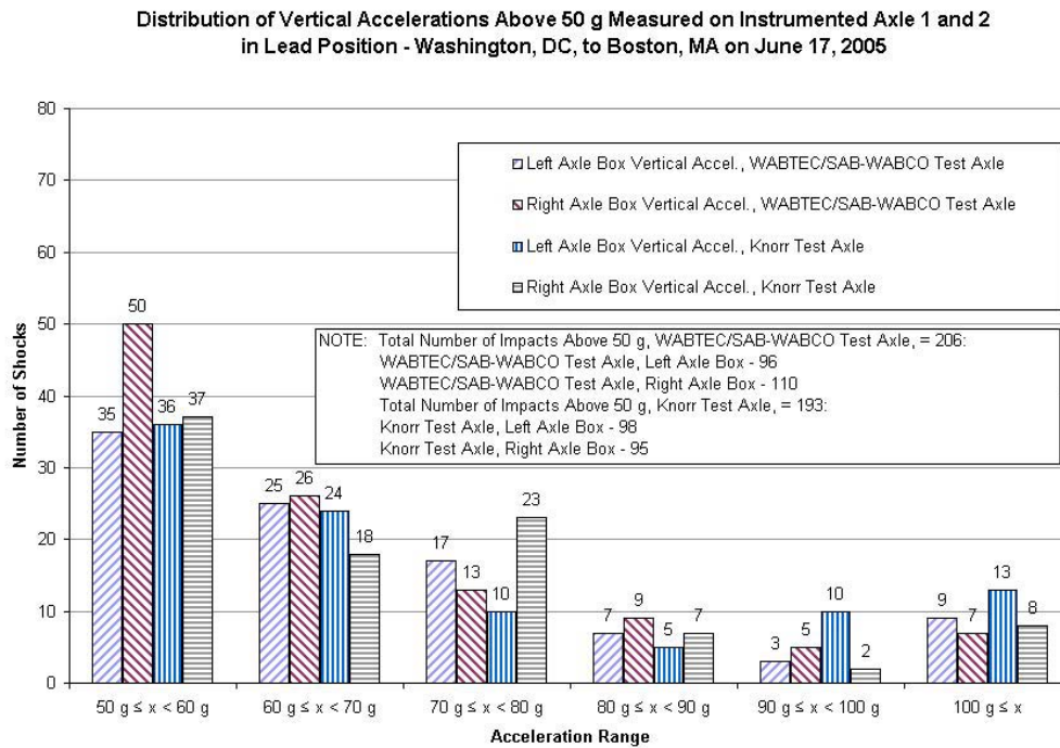
Figure 3.46a. Distribution of Vertical Accelerations Above 50 g Measured on Instrumented Axles 1 and 2 in Lead Position—Washington, DC, to Boston, MA, on June 17, 2005
