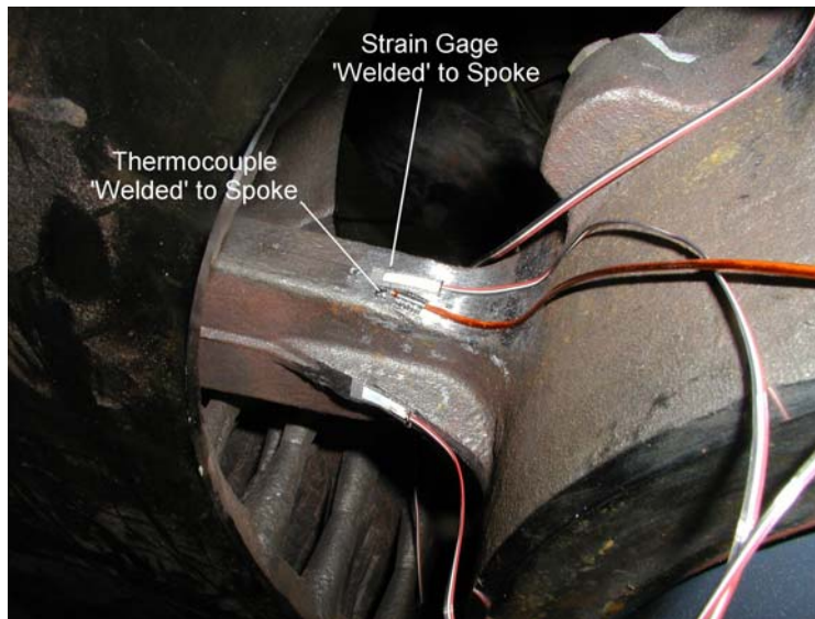
Figure 2.19. Thermocouple Applied to Spoke on Instrumented WABTEC/SAB-WABCO Supplied Disc During Phase 1 of Acela Brake Disc Study
