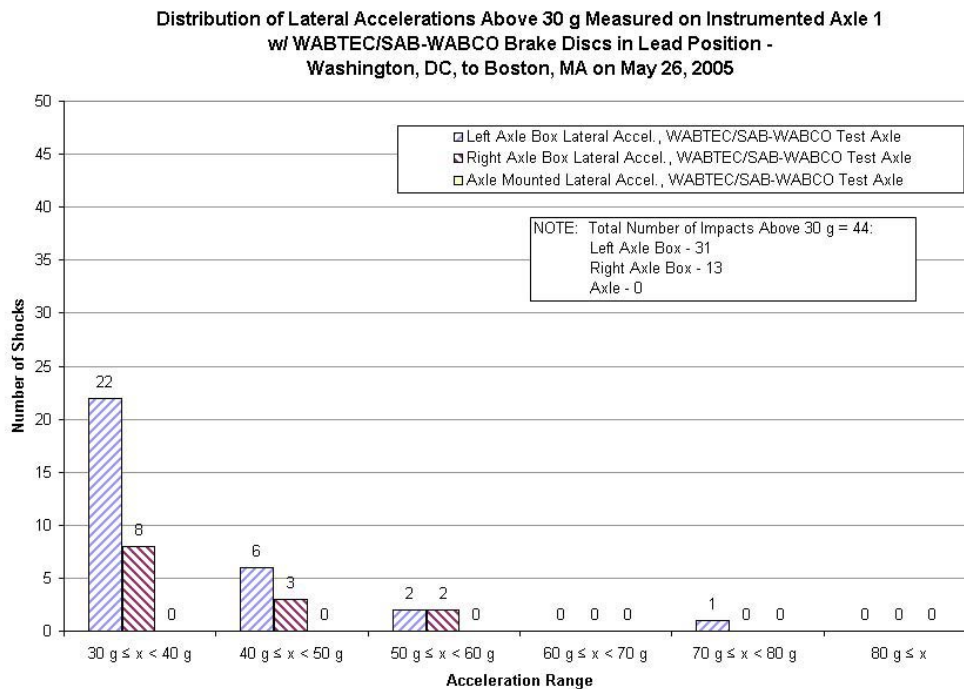
Figure 3.26a. Distribution of Lateral Accelerations Above 30 g Measured on Instrumented Axle 1 with WABTEC/SAB-WABCO Supplied Brake Discs in Lead Position—Washington, DC, to Boston, MA, on May 26, 2005
