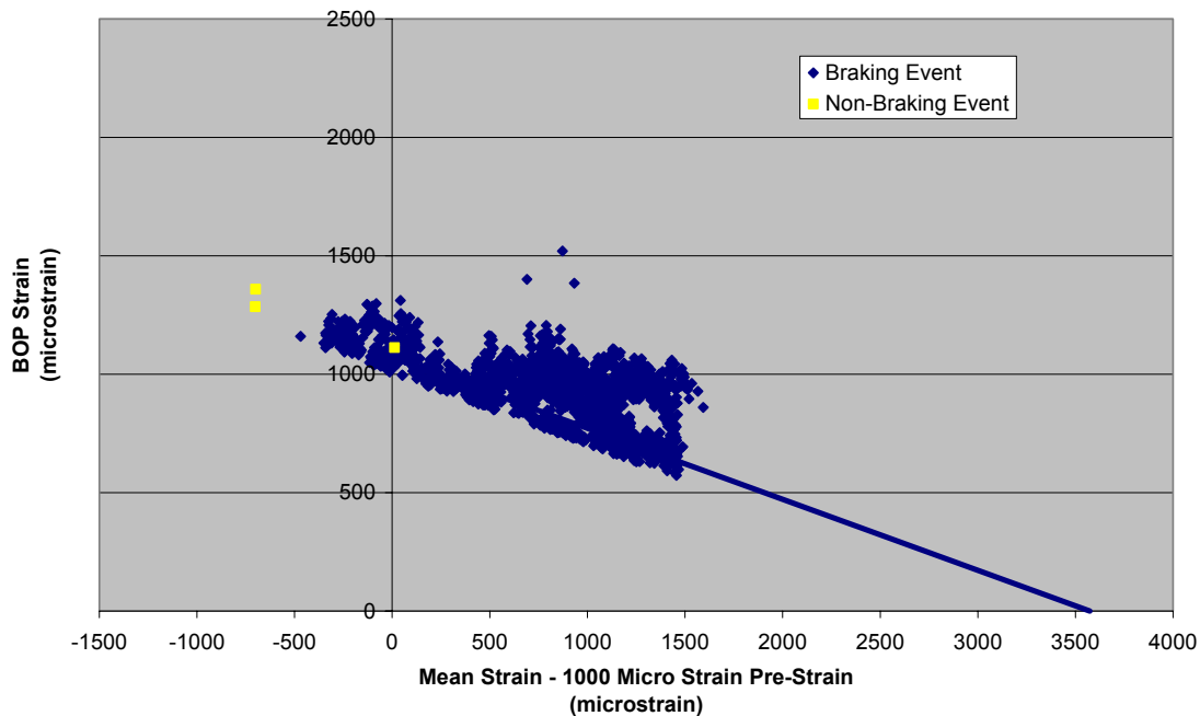
Figure 3.73. Mean Strain versus Alternating Strain, Center WABTEC/SAB-WABCO Supplied Brake Disc, Spokes 6 and 3–June 18, 2005
