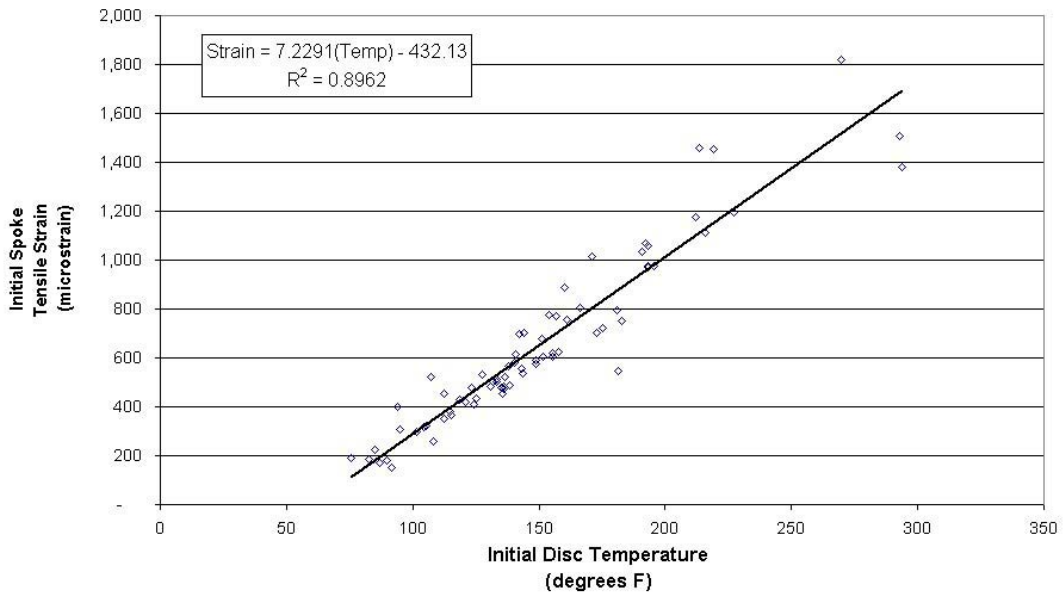
Figure 3.41. Brake Disc Temperature versus Initial Spoke Tensile Strain Before Brake Applications, Center WABTEC/SAB-WABCO Supplied Disc, Spoke 6–May 26, 2005
