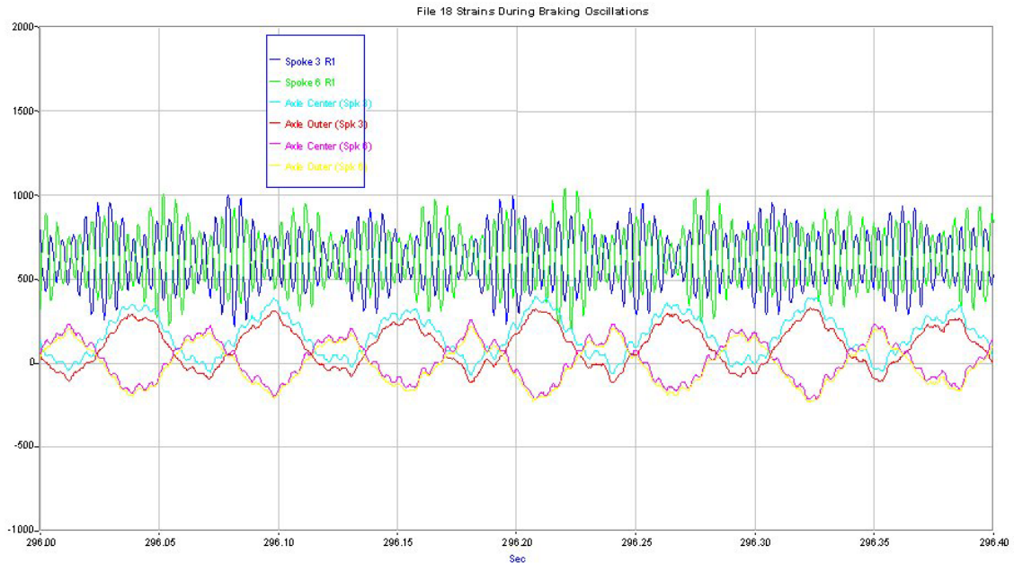
Figure 3.39. Axle Bending Strains Recorded During Case of Small Oscillating BOP Strains During Brake Application (File 052605_18.AB2)–May 26, 2005
