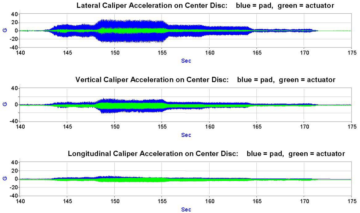
Figure 3.16. Accelerations Measured on Center Caliper During Brake Application with High BOP Strains (File 051705_19.ABT)–May 17, 2005
