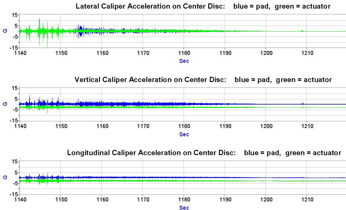
Figure 3.14. Accelerations Measured on Center Caliper During Normal Brake Application (File 051705_19.ABT)–May 17, 2005
