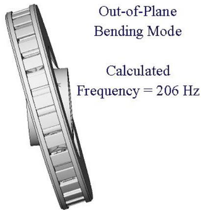
Figure 3.1. Out-of-Plane Bending Mode Determined from FEA
