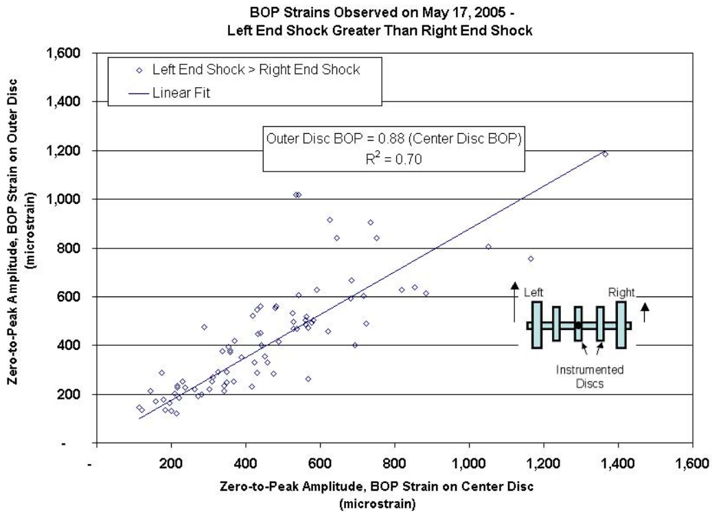
Figure 3.10a. Comparison of BOP Amplitudes of WABTEC/SAB-WABCO Supplied Center and Outer Discs Measured During Vertical Impacts, Left End Shock Greater Than Right End Shock—May 17, 2005
