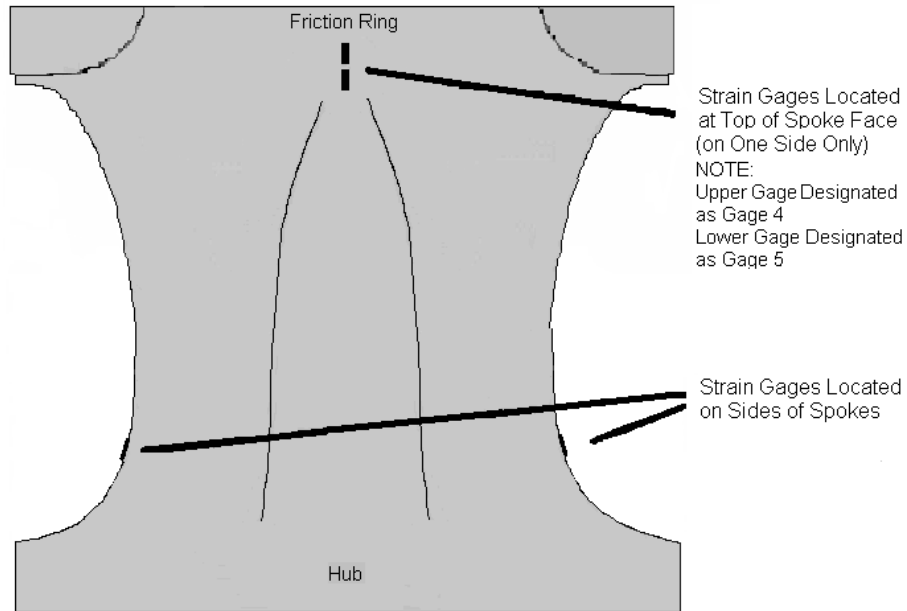
Figure 2.7. Illustration of Strain Gage Locations on Knorr Disc Used During Phase 3 of Acela Brake Disc Study
