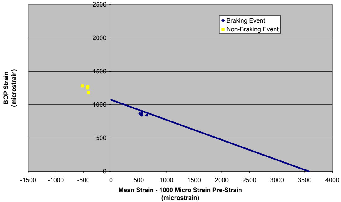
Figure 3.70. Mean Strain versus Alternating Strain, Center WABTEC/SAB-WABCO Supplied Brake Disc, Spokes 6 and 3—May 26, 2005
