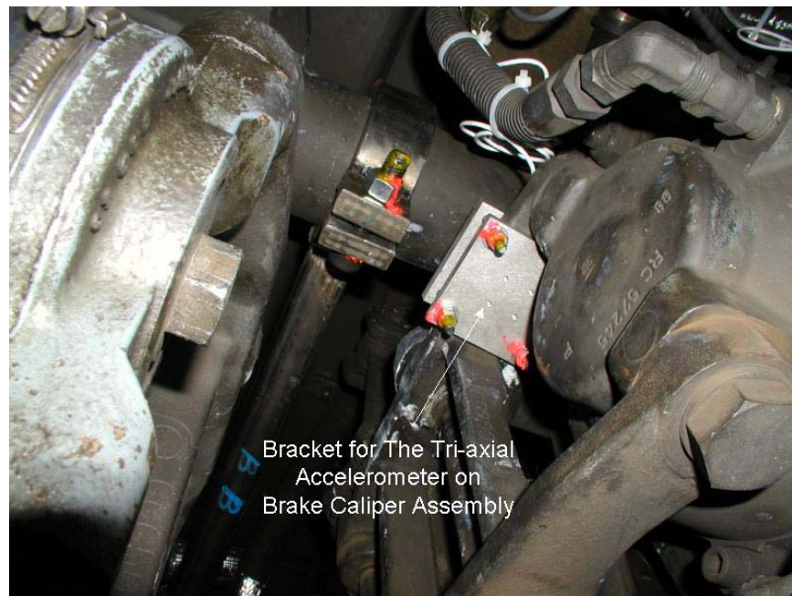
Figure 2.14. Tri-Axial Accelerometer Mounted on Center Brake Caliper Assembly Near Actuator for WABTEC/SAB-WABCO Test Axle, Phase 1 of Acela Brake Disc Study
