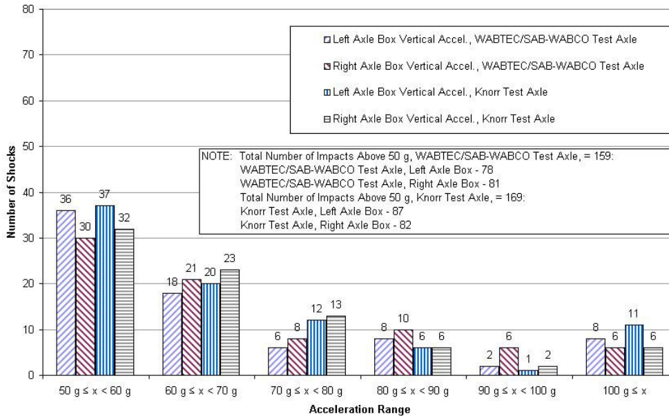
Figure 3.46b. Distribution of Vertical Accelerations Above 50 g Measured on Instrumented Axles 1 and 2 in Lead Position—Boston, MA, to Washington, DC, on June 18, 2005
