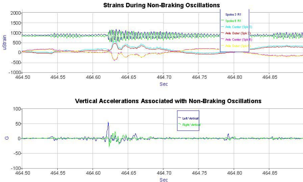
Figure 3.40. Axle Bending Strains Recorded During Response of WABTEC/SAB-WABCO Supplied Brake Disc to Vertical Impact (File 052605_18.AB2)–May 26, 2005
