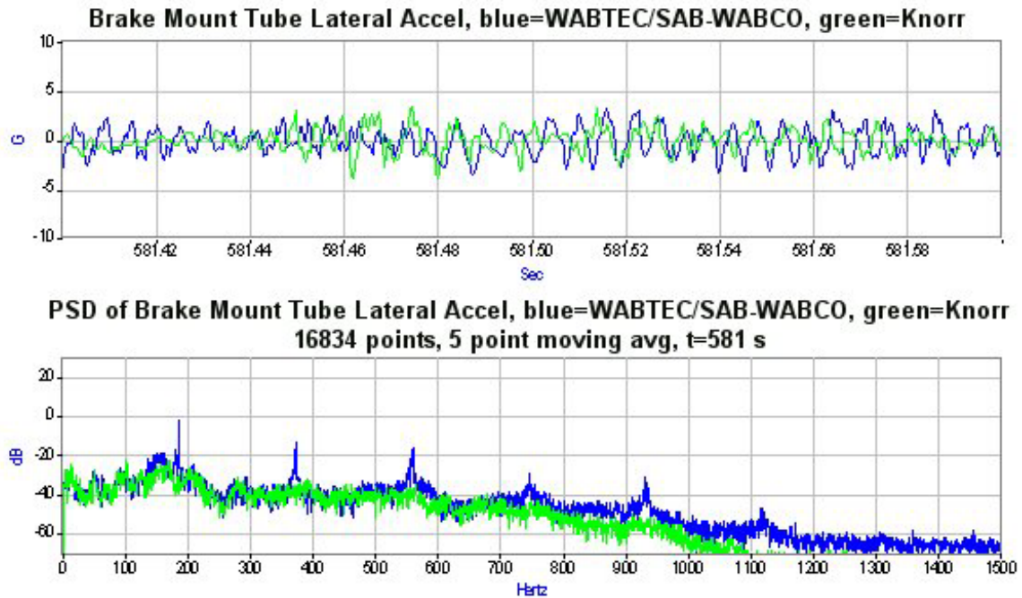
Figure 3.58. Time History and PSD of Brake Mounting Tube Lateral Accelerations During Sustained Oscillations While Braking (File 061805_24.AB3)–June 18, 2005
