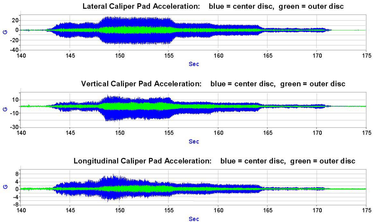
Figure 3.17. Accelerations Measured on Center and Outer Calipers Near Pads During Brake Application with High BOP Strains (File 051705_19.ABT)–May 17, 2005
