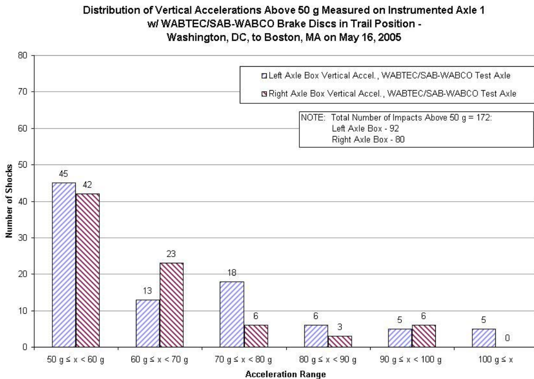
Figure 3.6a. Distribution of Vertical Accelerations Above 50 g Measured on Instrumented Axle 1 with WABTEC/SAB-WABCO Supplied Brake Discs in Trail Position— Washington, DC, to Boston, MA, on May 16, 2005
