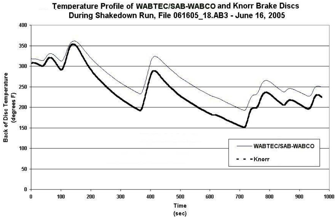
Figure 3.55. Temperature Profiles from Back of WABTEC/SAB-WABCO Supplied and Knorr Brake Discs During Shakedown Run (File 061605_18.AB3)–June 16, 2005
