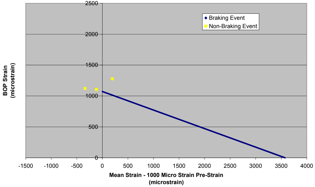
Mean Strain vs. Alternating Strain, Outer WABTEC/SAB-WABCO Disc, Spoke 6 - May 16, 2005
