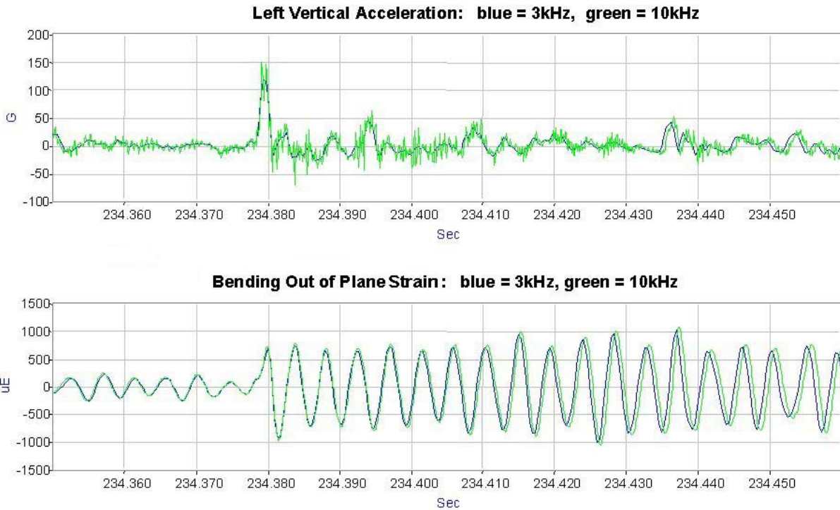
Figure 3.24. Comparison of Vertical Shock and BOP Strains Recorded with 3,000 Hz and 10,000 Hz Sampling Rates (Files 052605_18.AB2 [3,000 Hz Data] and File 052605_18.001 [10,000 Hz Data])–May 26, 2005
