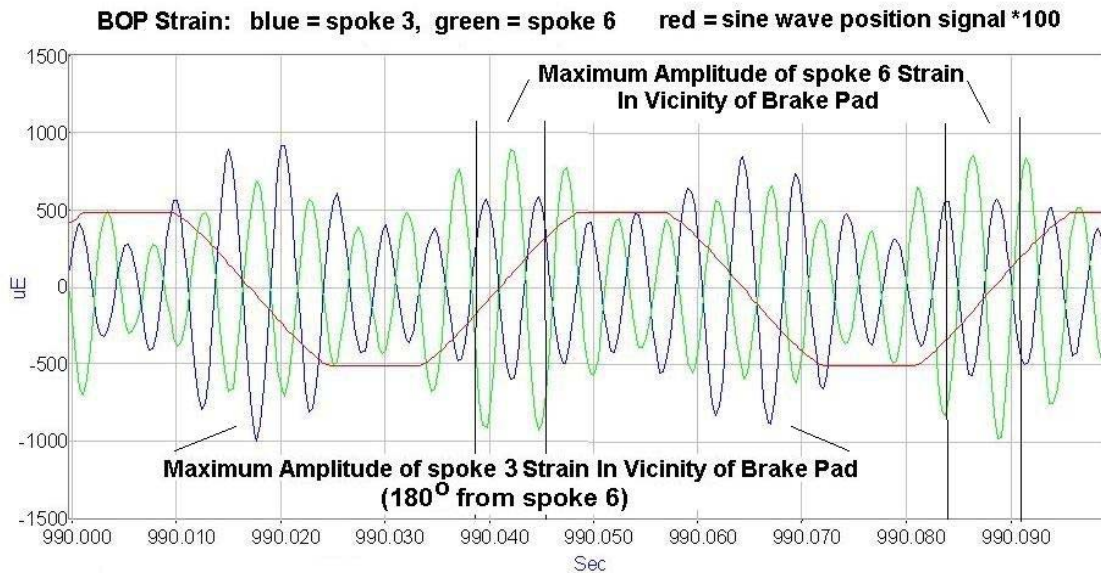
Figure 3.31. BOP Strains Recorded During Braking on Center WABTEC/SAB-WABCO Supplied Brake Disc Near MP AB 158 During Phase 2 Testing (File 052605_15.AB2)–May 26, 2005
