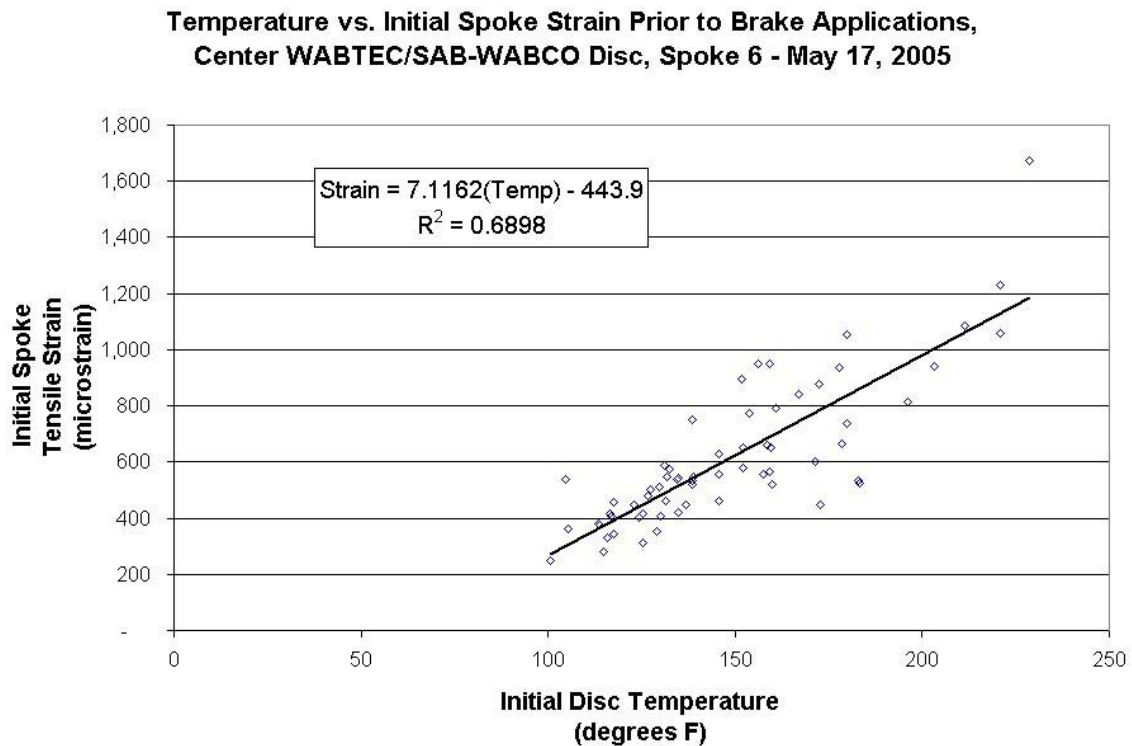
Figure 3.21. Brake Disc Temperature versus Initial Spoke Tensile Strain Before Brake Applications, Center WABTEC/SAB-WABCO Supplied Disc, Spoke 6–May 17, 2005
