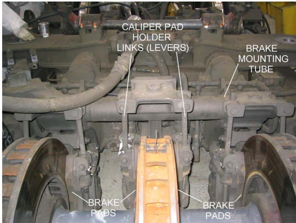
Figure 2.10. Brake Caliper Support Links and Mounting Tube (Shown on Removed Truck for Clarity)
