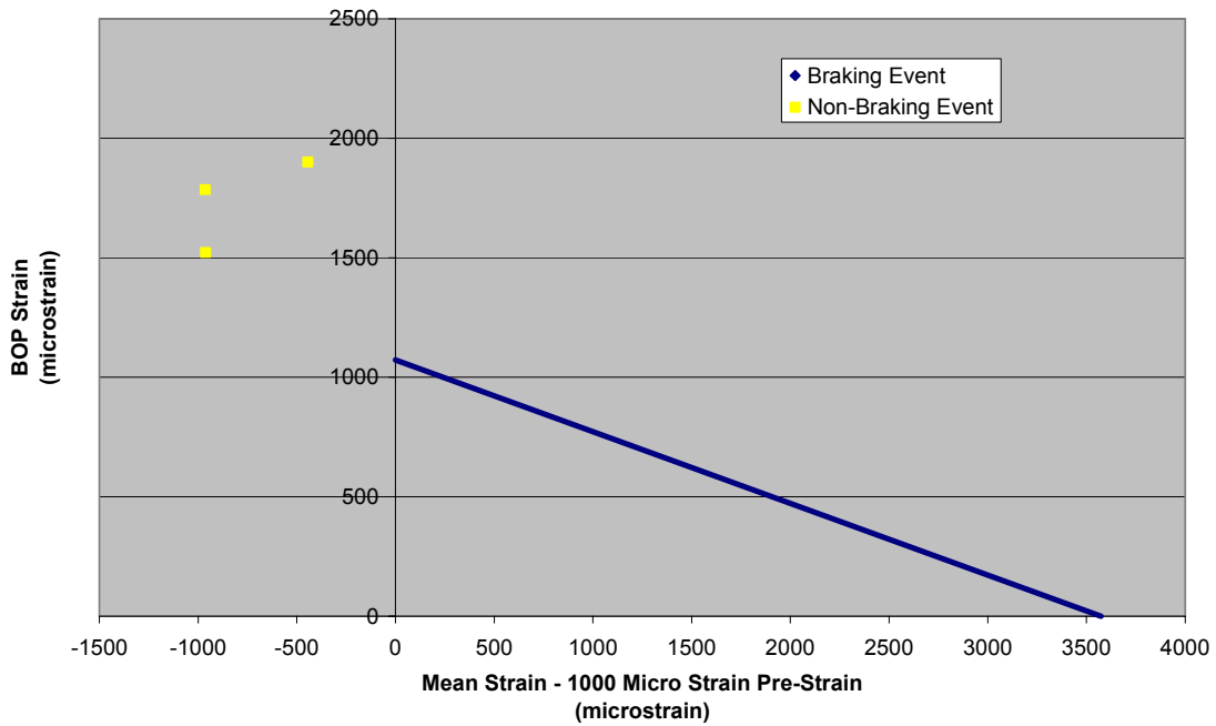
Figure 3.71. Mean Strain versus Alternating Strain, Center WABTEC/SAB-WABCO Supplied Brake Disc, Spokes 6 and 3—May 27, 2005
