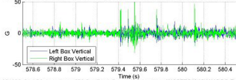
File 061805_24.AB3, Location = 579.5 s, Truck Frame Accelerations W/ABTEC/SAB-W/ABCO Test Axle
