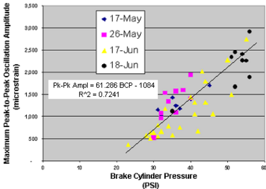
Figure 3.66. Relationship of Peak-to-Peak Sustained Oscillations to Brake Cylinder Pressure, Data Collected Throughout Test Effort
