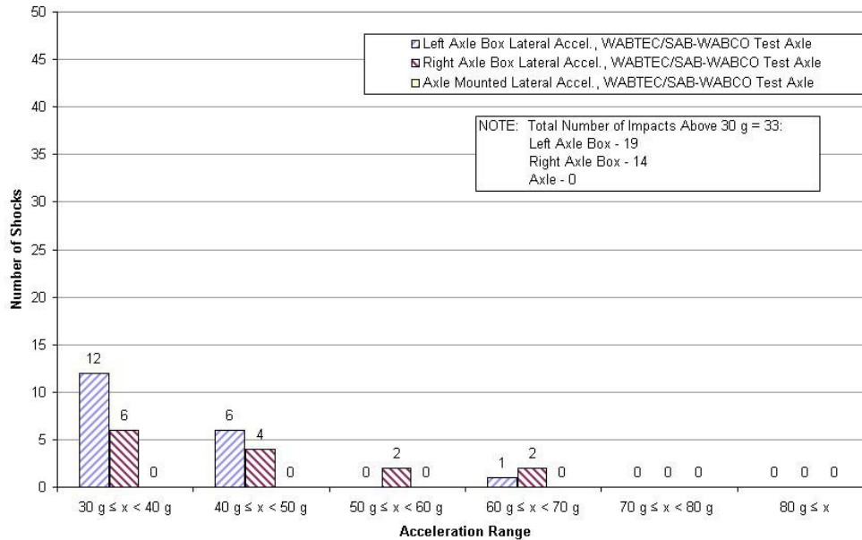
Distribution of Lateral Accelerations Above 30 g Measured on Instrumented Axle 1 w/ WABTEC/SAB-WABCO Brake Discs in Trail Position - Boston, MA, to Washington, DC, on May 27, 2005
