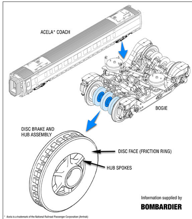
Figure 1.1. Typical Acela Coach, Bogie and Brake Disc
