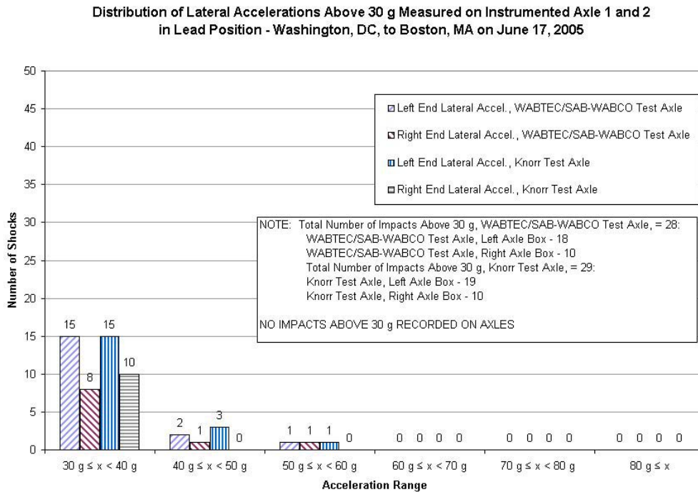
Figure 3.47a. Distribution of Lateral Accelerations Above 30 g Measured on Instrumented Axles 1 and 2 in Lead Position—Washington, DC, to Boston, MA, on June 17, 2005
