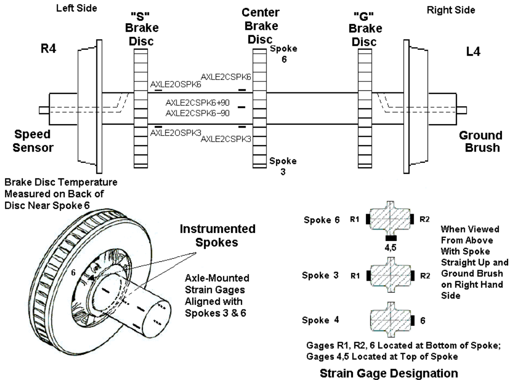
Figure 2.9b. Location of Strain Gages on Knorr Test Axle During Phase 3 of Acela Brake Disc Study
