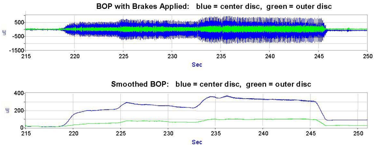
Figure 3.12. BOP Strain Recorded on Center and Outer WABTEC/SAB-WABCO Supplied Brake Discs During Braking Near MP E17 (File 051705_17.ABT)–May 17, 2005
