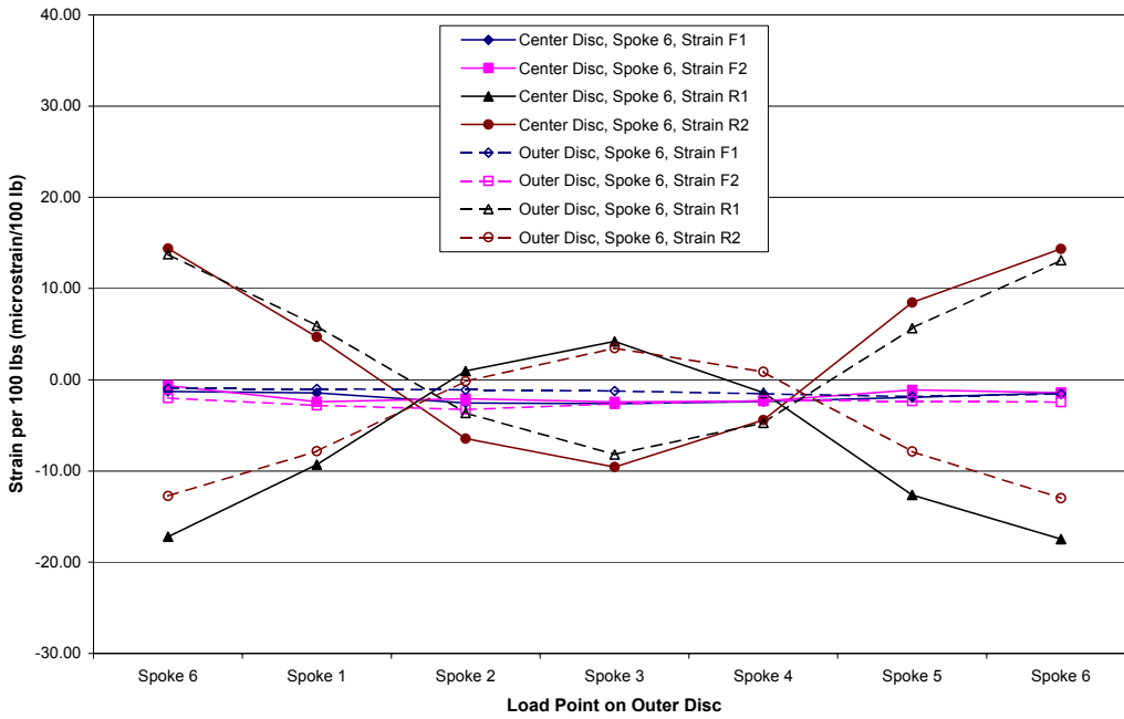
Figure 3.23b. Strains Measured During Spreader Bar Test, Load Aligned with Spokes of Outer Disc
