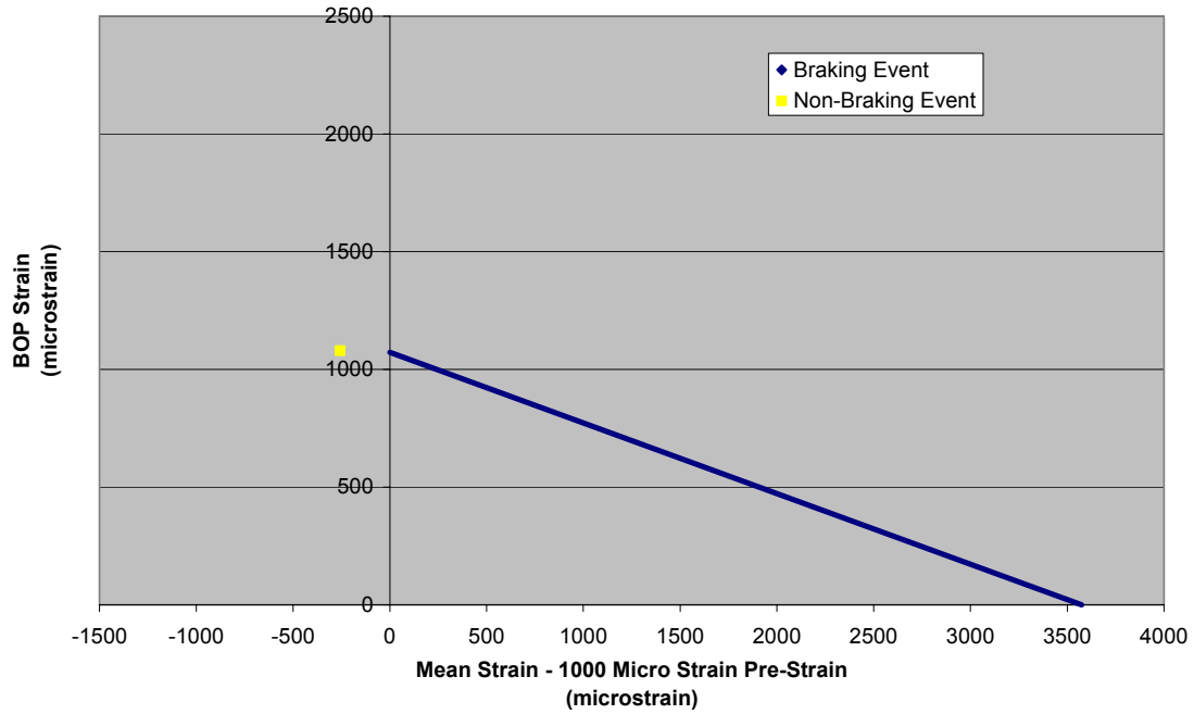
Figure 3.69. Mean Strain versus Alternating Strain, Center and Outer WABTEC/SAB-WABCO Supplied Brake Discs, Spoke 6–May 17, 2005
