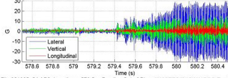
File 061805_24.AB3, Location = 579.5 s, Bending Out of Plane W/ABTEC/SAB-W/ABCO Test Axle
