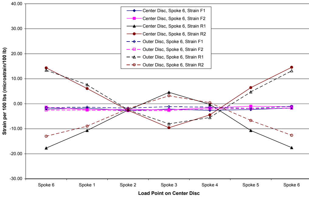
Figure 3.23a. Strains Measured During Spreader Bar Test, Load Aligned with Spokes of Center Disc
