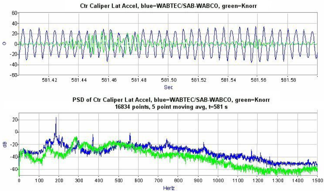
Figure 3.60. Time History and PSD of Brake Caliper Pad Lateral Accelerations During Sustained Oscillations While Braking (File 061805_24.AB3)–June 18, 2005
