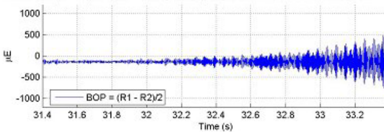
File 061805_07_AB3, Location = 32.4 s, Bending Out of Plane W/ABTEC/SAB-W/ABC0 Test Axle
