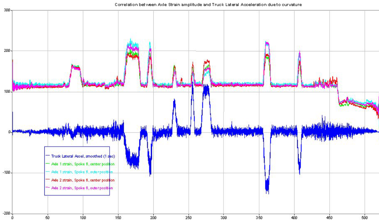
Figure 3.52. Comparison of Truck Frame Lateral Accelerations and Axle Strains (File 061805_03.AB3)–June 18, 2005
