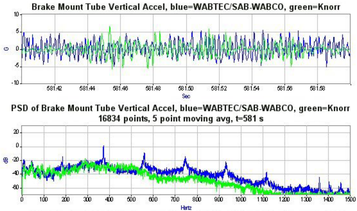
Figure 3.57. Time History and PSD of Brake Mounting Tube Vertical Accelerations During Sustained Oscillations While Braking (File 061805_24.AB3)—June 18, 2005
