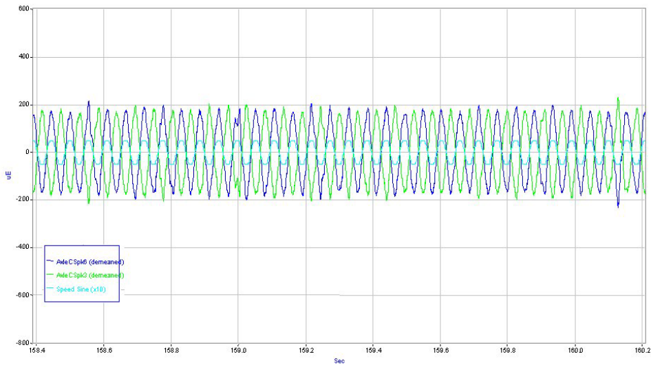
Figure 3.38. Typical Axle Bending Strains Recorded Over Tangent Track (File 052605_18.AB2)–May 26, 2005
