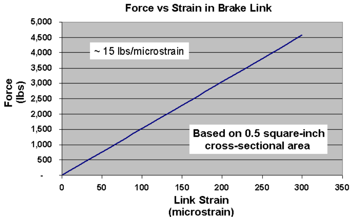
Figure 3.62. Brake Link Strain Level–Force Relationship
