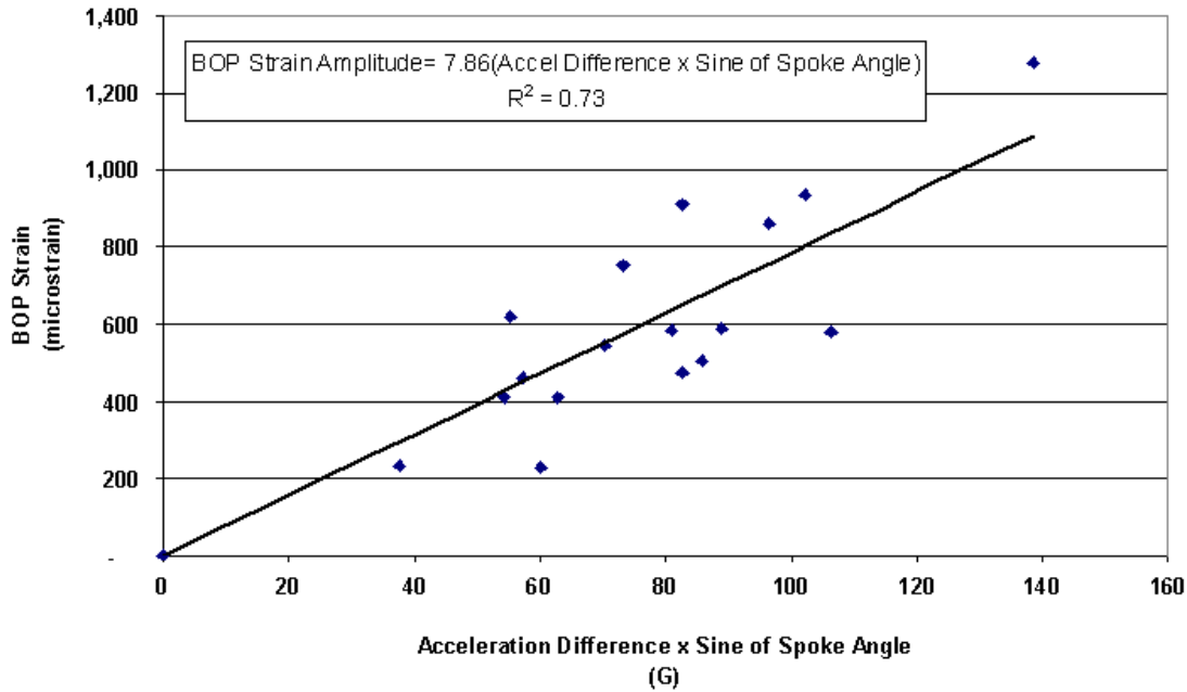
Figure 3.34. Correlation of BOP Strain Amplitudes and Acceleration Differences Based on Measurements Collected on May 26, 2005
