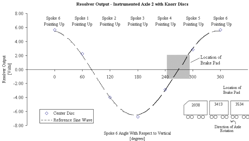
Figure 2.24. Instrumented Spoke Phase Based on Wheel Angular Position, Knorr Disc
