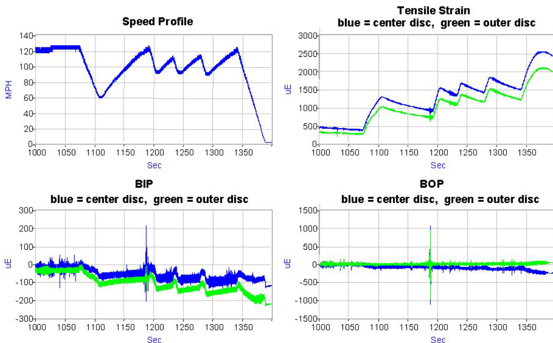
Figure 3.8. Strains on Spoke 6 of Center and Outer WABTEC/SAB-WABCO Supplied Brake Discs During Brake Applications (File 051605_09.ABT)–May 16, 2005
