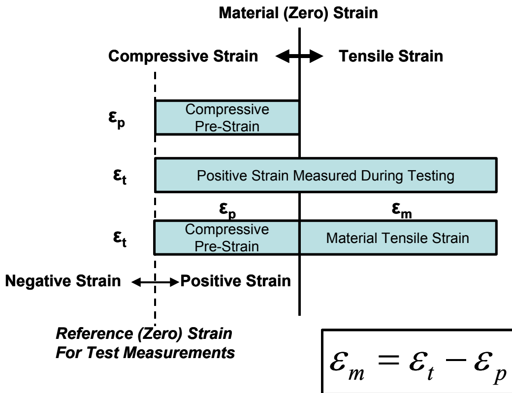
Figure 2.27. Illustration of Concept of Compressive Pre-Strain
