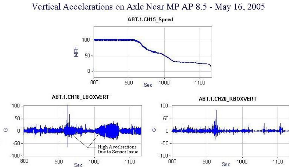
Figure 3.3. Vertical Accelerations Measured on Instrumented Axle 1 Near MP AP 8.5 (File 051605_08.ABT)–May 16, 2005
