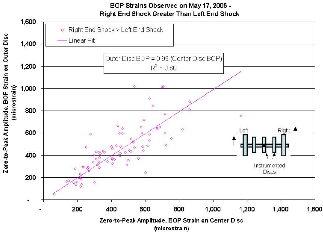
Figure 3.10b. Comparison of BOP Amplitudes of WABTEC/SAB-WABCO Supplied Center and Outer Discs Measured During Vertical Impacts, Right End Shock Greater Than Left End Shock—May 17, 2005
