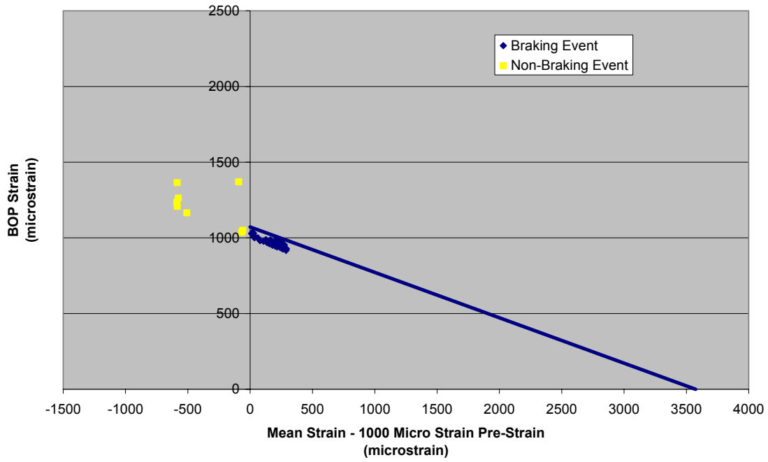
Mean Strain vs. Alternating Strain, Outer WABTEC/SAB-WABCO Disc, Spoke 6 - May 17, 2005
