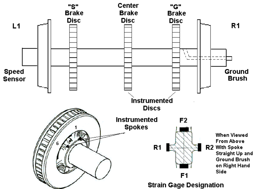
Figure 2.3. Location of Strain Gages on WABTEC/SAB-WABCO Supplied Discs During Phase 1 of Study
