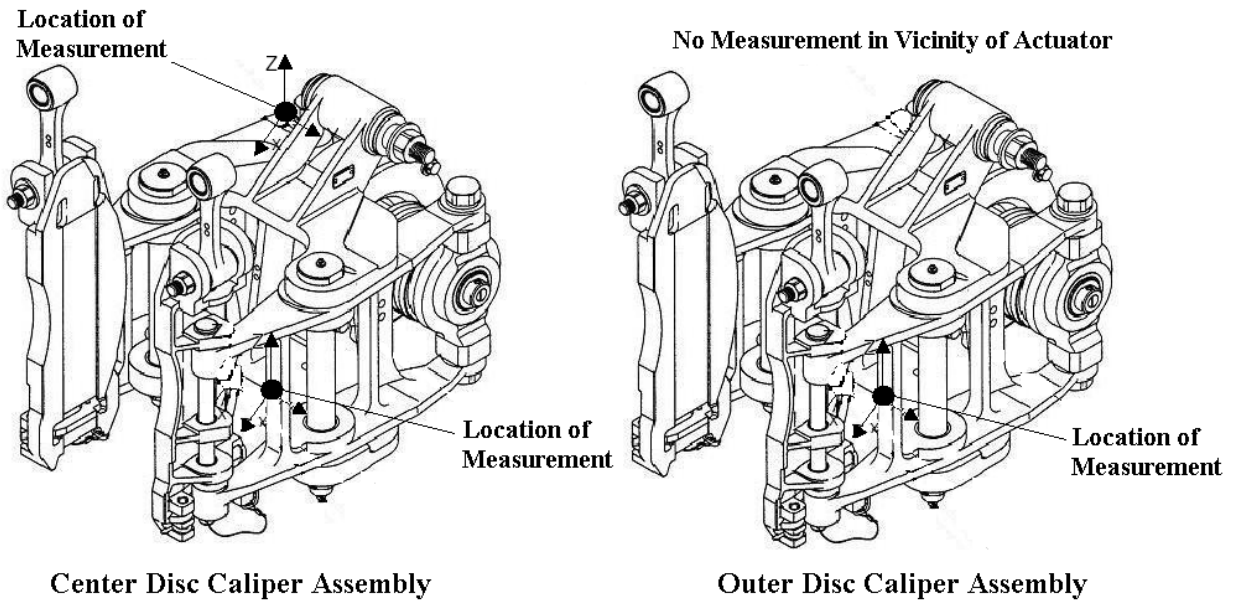
Figure 2.13. Acceleration Measurement Locations on the Caliper Assemblies
