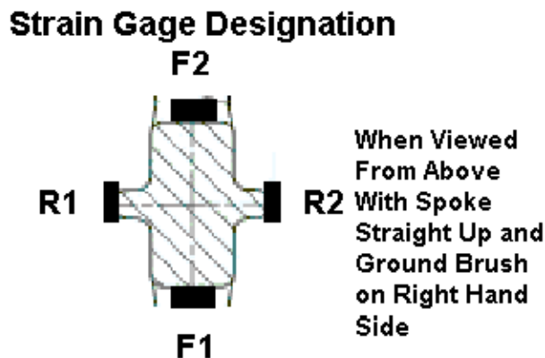
Figure 3.7. Designation of Strain Gages Used on Spoke 6 of Center and Outer Instrumented WABTEC/SAB-WABCO Supplied Discs During Phase 1 Testing
