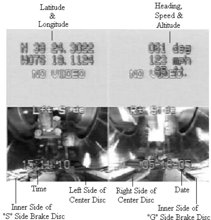
Figure 2.26. Example of Video Collected Over WABTEC/SAB-WABCO Test Axle
