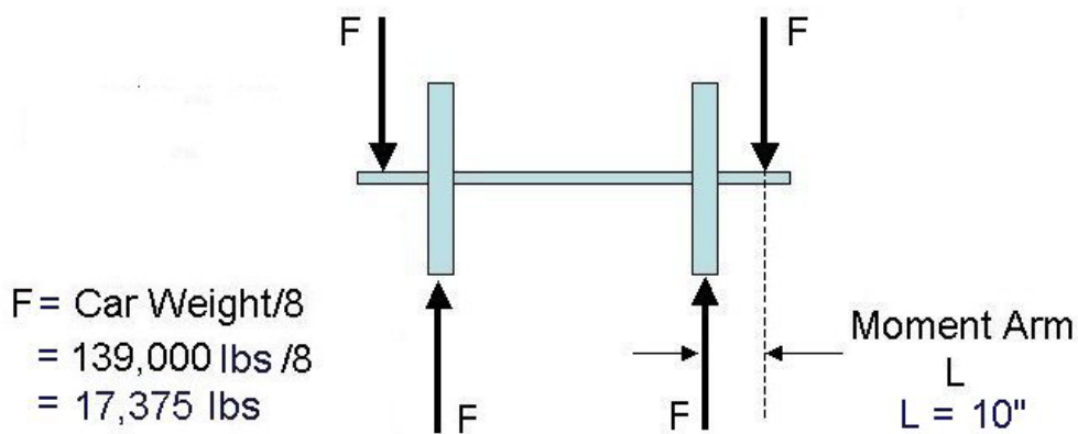
Figure 3.36. Bending Moments in Generic Wheelset
