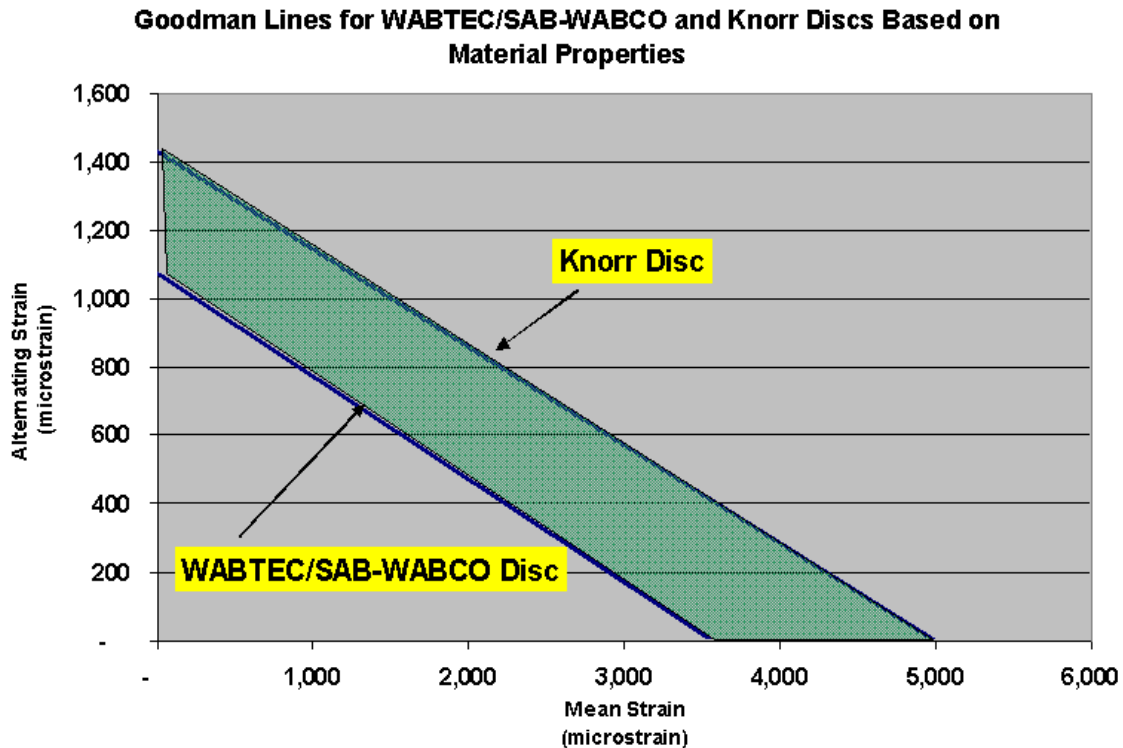
Figure 3.74. Comparison of Goodman Lines for WABTEC/SAB-WABCO Supplied and Knorr Brake Discs
