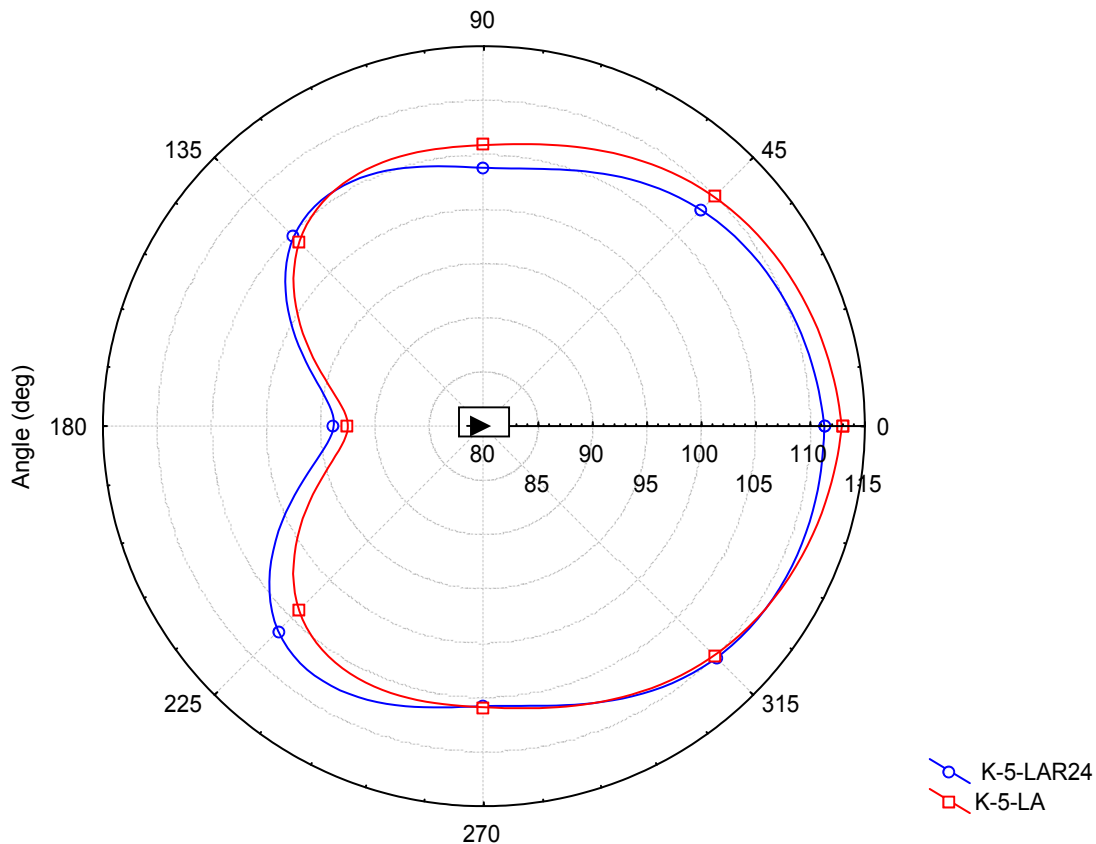
Figure 12. Directivity of Directional vs Bi-Directional Horn
