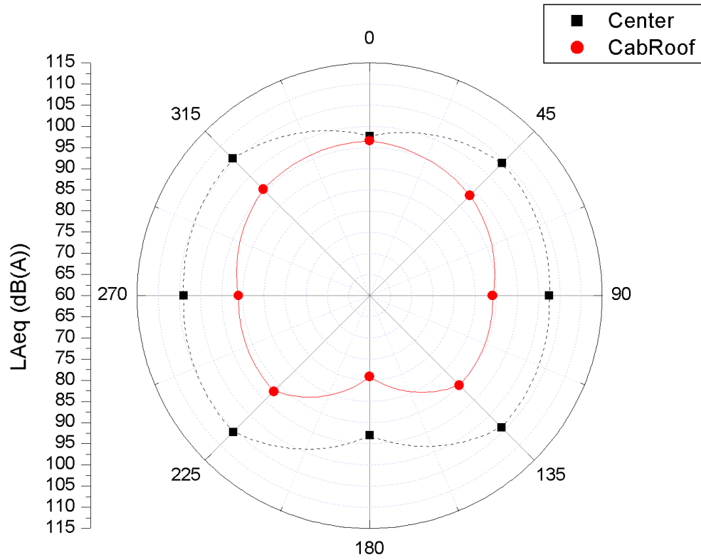
Figure C -9 Acoustic Data Measured 100 ft from horn Airchime K-5-LAR24, GP-40 Locomotive 96 dB(A) 100 ft forward of the locomotive
