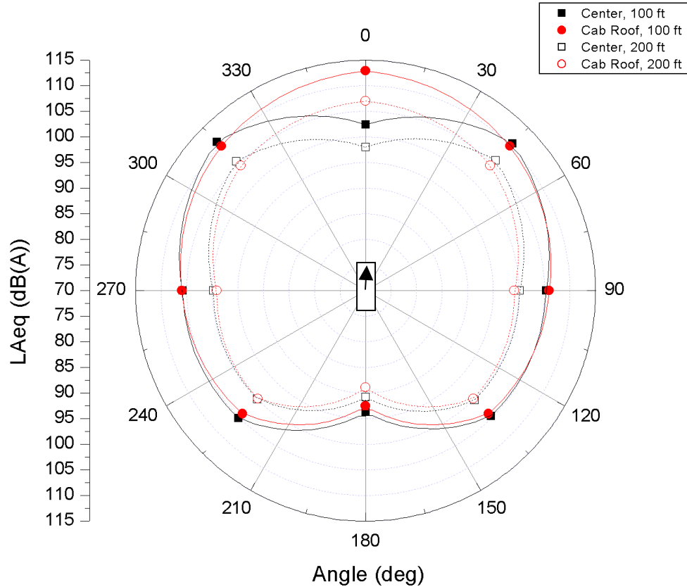
Figure 11. Center-Installed vs. Cab Roof Installed Sound Levels
