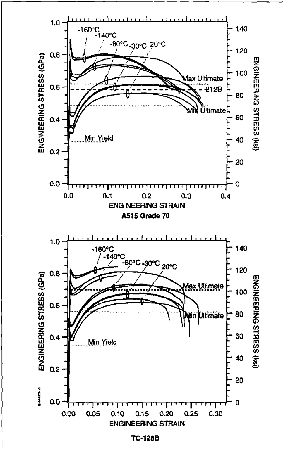
Figure 14. Engineering Stress-Strain Curves from Smooth Round Bar Laboratory Results
