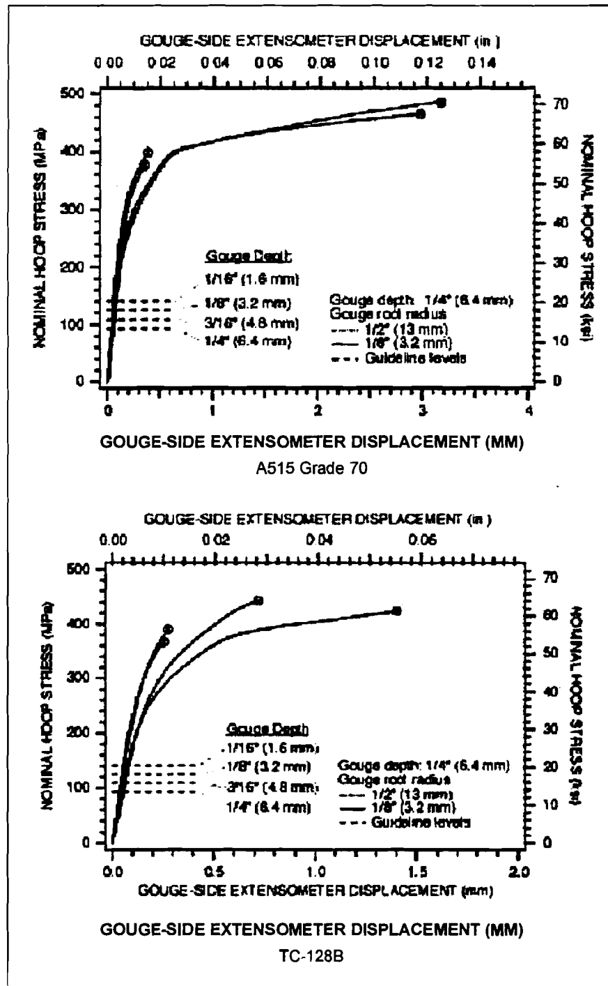
Figure 24. Results of Simulated Gouge Tests
