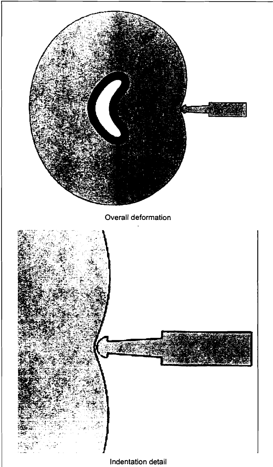
Figure 40. Unpressurized Indentation at 40 mph for an A515-70 Ring at 100° F
