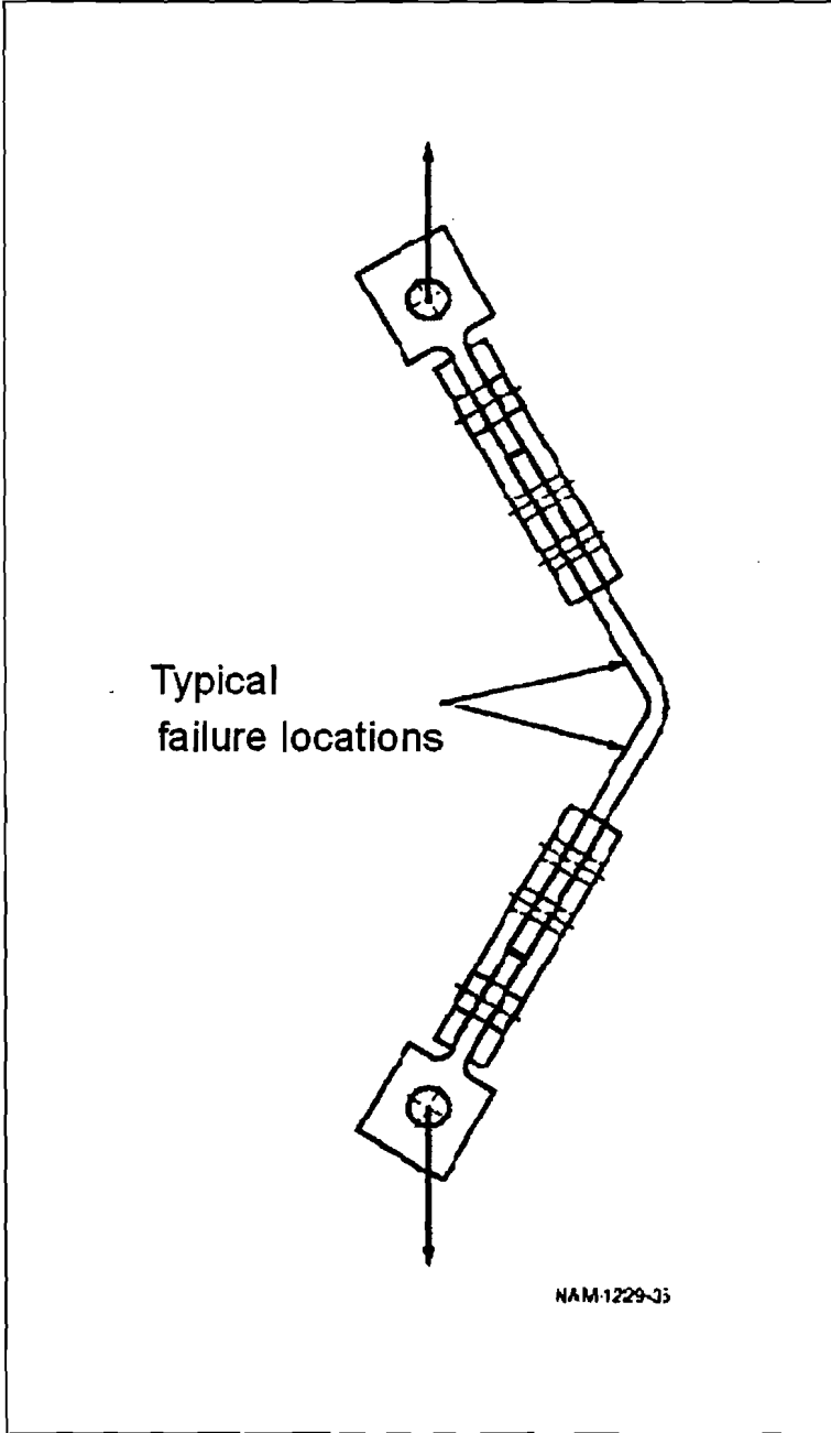
Figure 13. Configuration of Undent Tests
