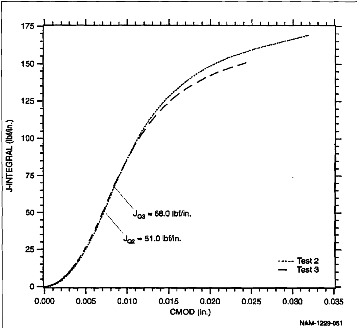
Figure 47. Results of Monotonic J_{Ic} Tests on A515-70 (A212B) at -40°F
