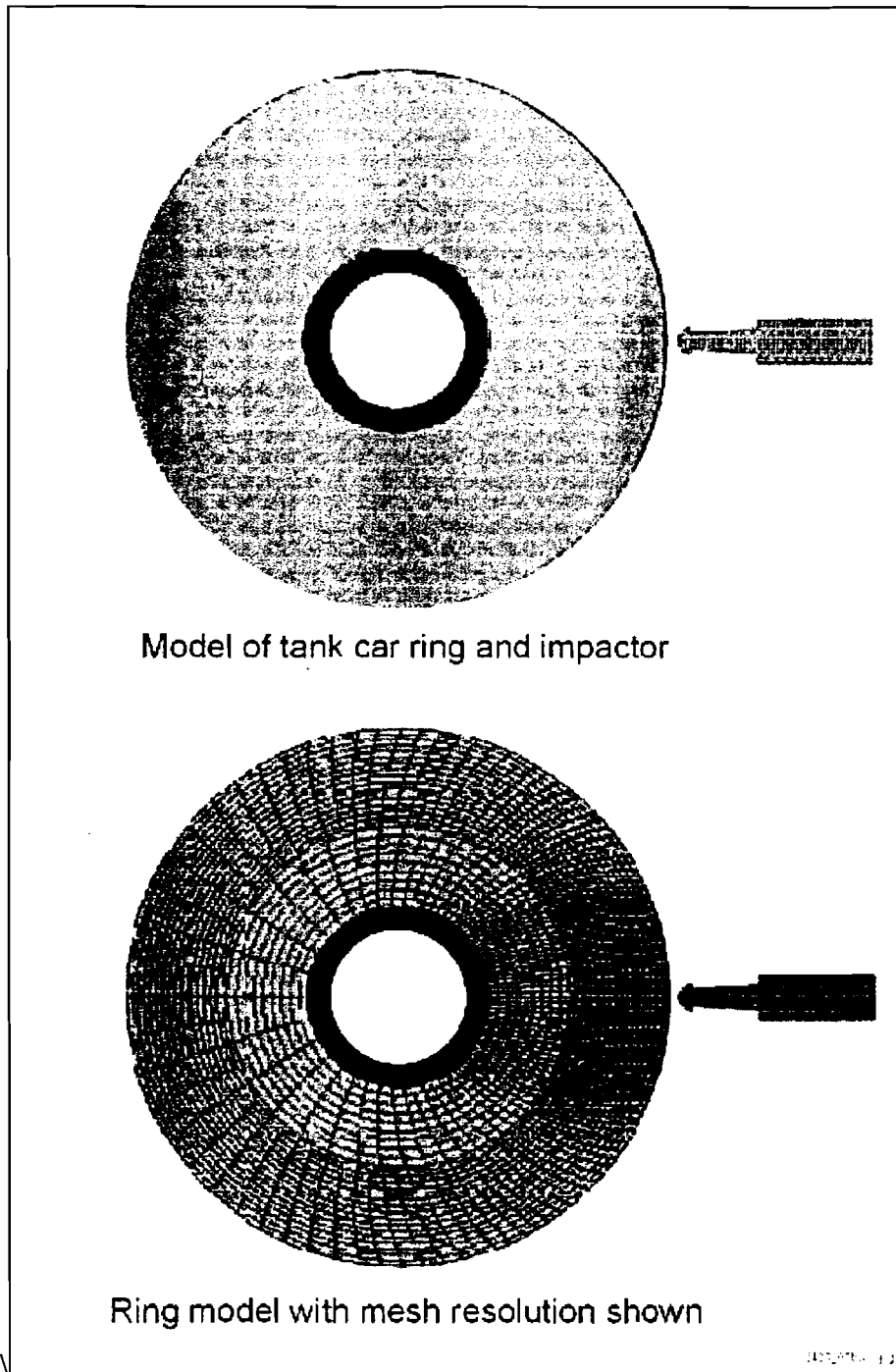
Figure 5. Finite Element Tank Car Ring Model Used to Calculate the Denting Response
