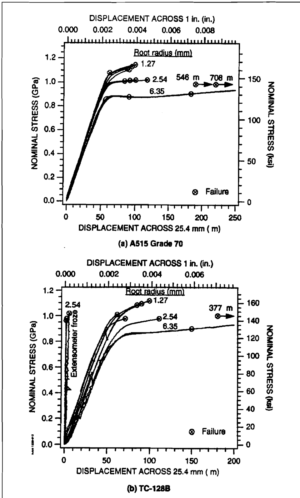
Figure 15. Tensile Stress-Displacement Curves from Notched Round Bar Laboratory Test Results
