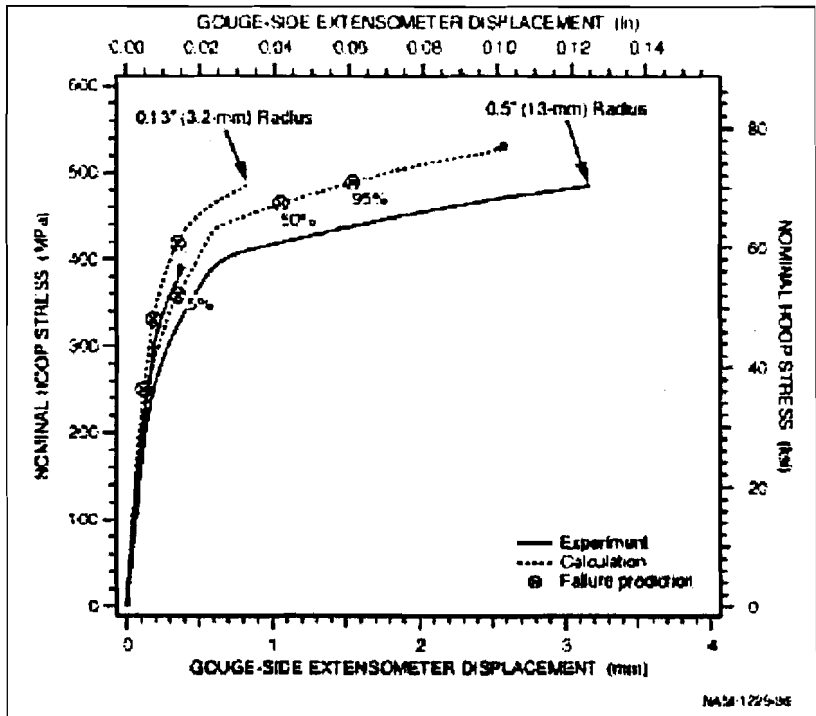
Figure 25. Summary of A515-70 Gouge Test Measurements at -238 F (-150° C) Compared to Calculated Response
