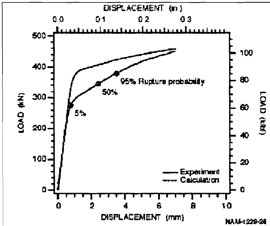
Figure 29. Comparison of Measurements and Analyses For the Engineering Bend Test with the TC-128B Tank Car Steel at -238°F (-150° C)
