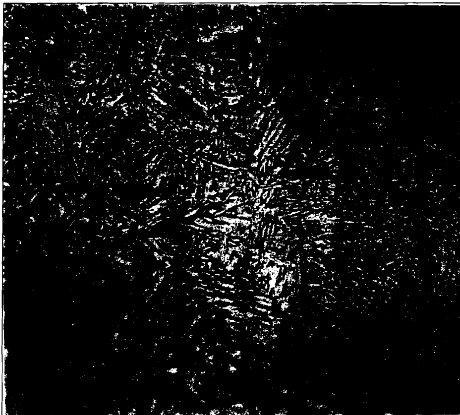
Figure B-9. Microstructure of Heat-Affected Zone, Etched with 2% Nital, X400
