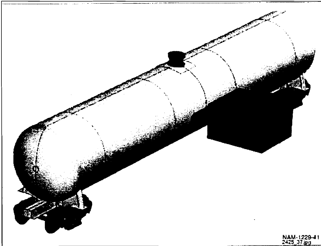
Figure 37. Model Used for Analysis of a Longitudinal Dent Response with Internal Pressure
