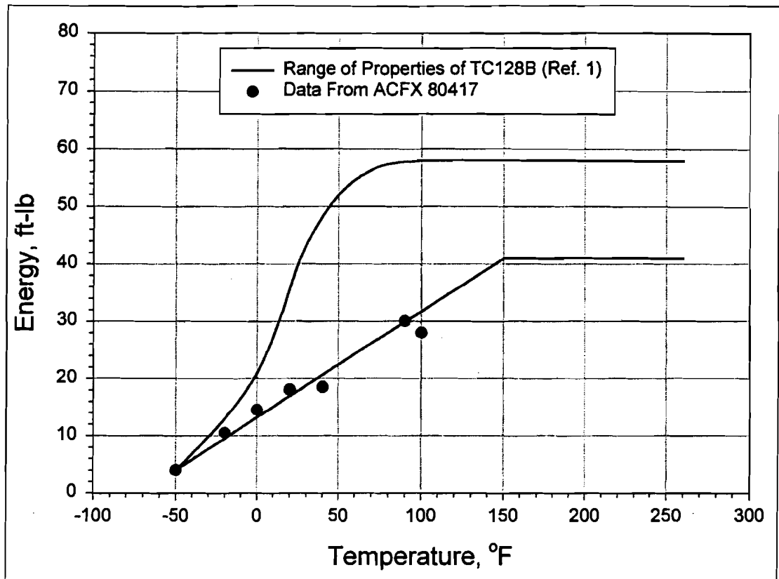
Figure B-7. Charpy V-Notch Properties in Vicinity of Crack
