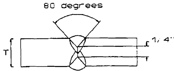
DETAIL 2
