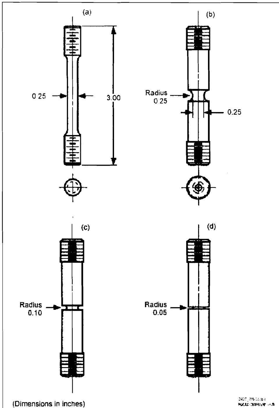
Figure 9. Round Bar Tensile Specimens: (a) Smooth, (b)-(d) Notched
