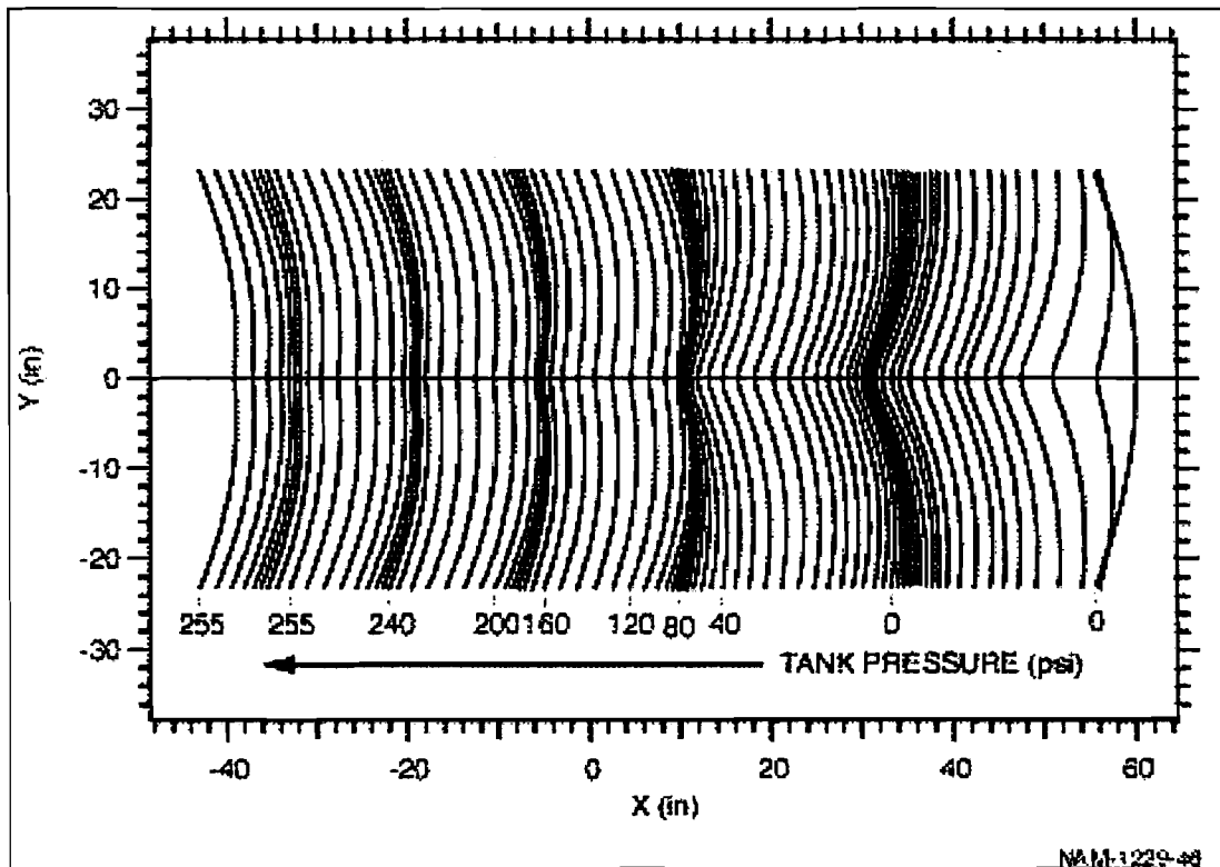
Figure 42. Progression of Dent Profile Following Impact from the Right and Subsequent Pressurization
