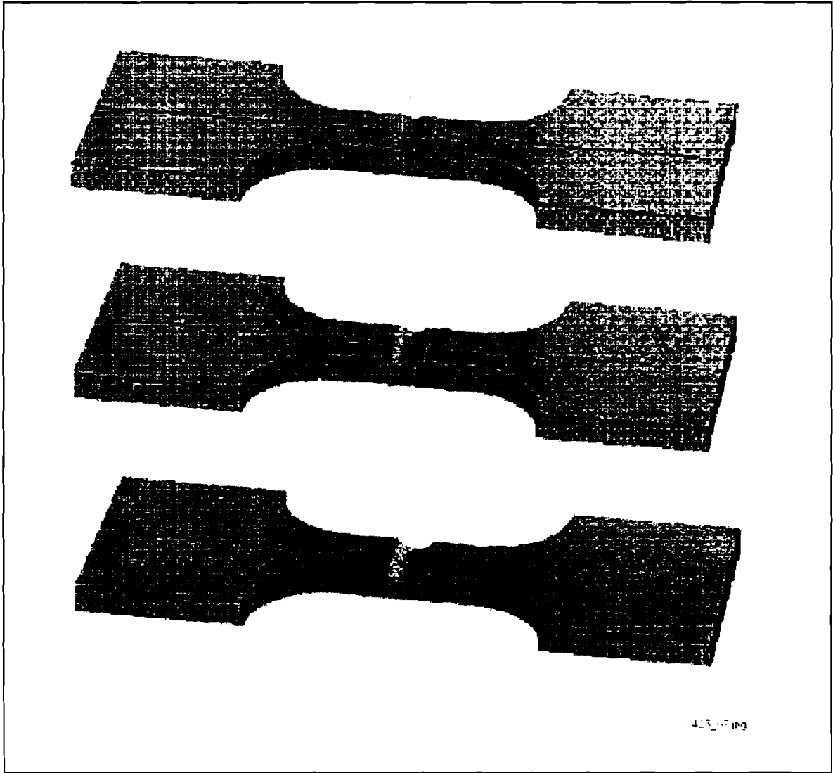
Figure 7. Example Finite Element Models for Analysis of Gouge Specimen Engineering Tests
