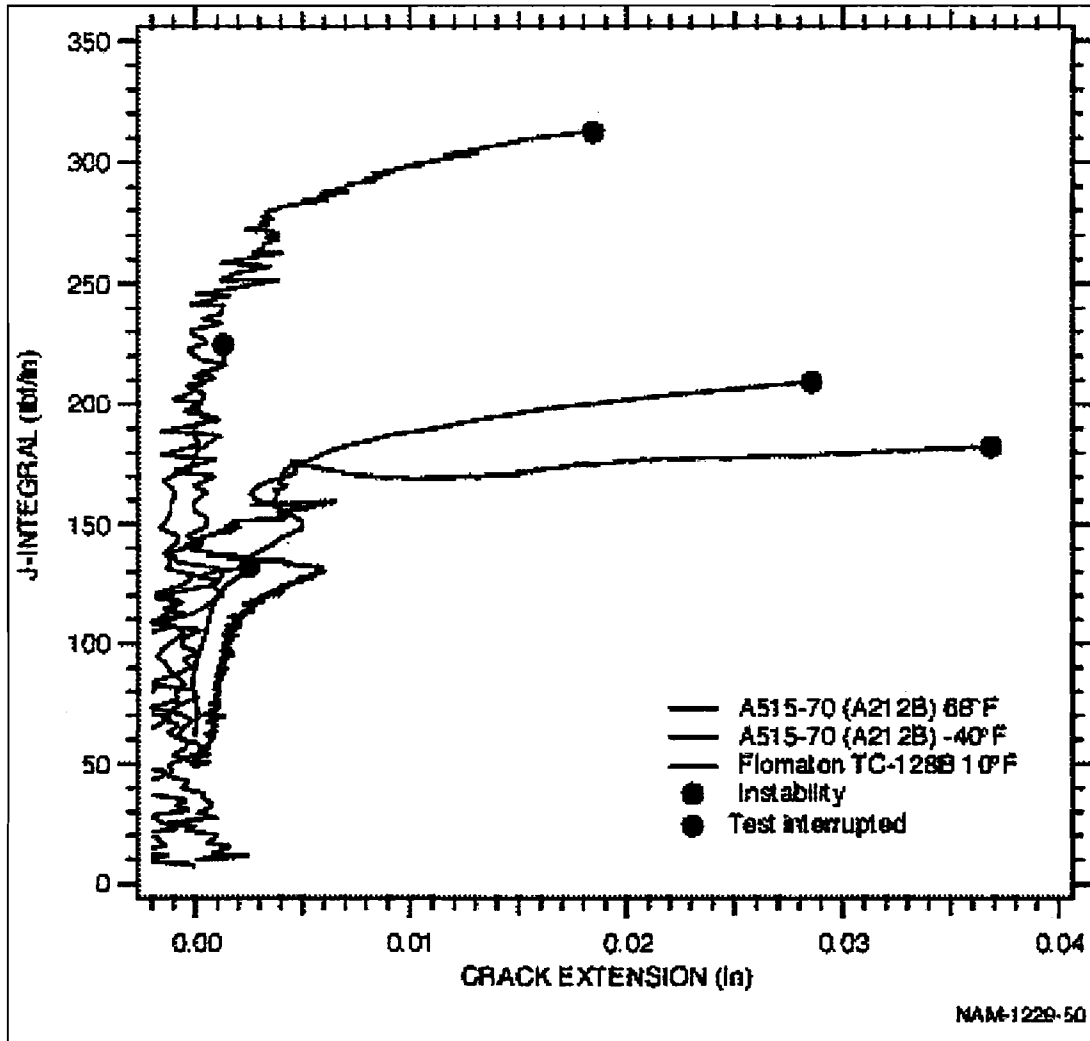
Figure 46. Results of J-R Curve Tests on Pressure Tank Car Steels
