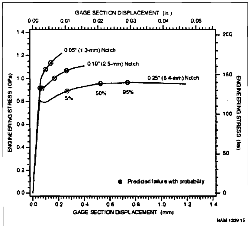
Figure 18. Calculated Notched Round Bar Stress-Displacement Curves for A515-70 with Rupture Probabilities Indicated (-238°F or -150°C)
