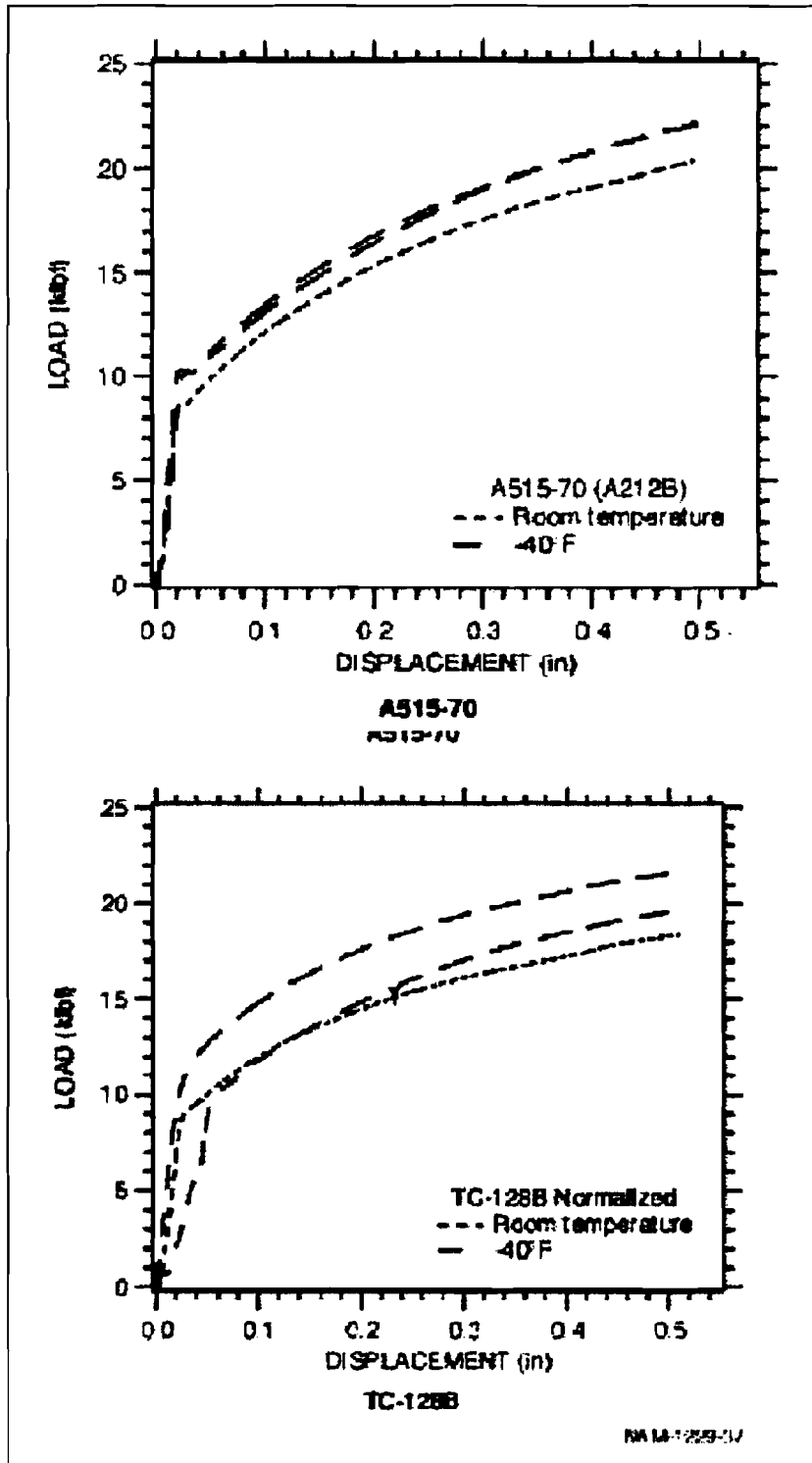
Figure 30. Results of Denting Portion of Dent/Undent Tests
