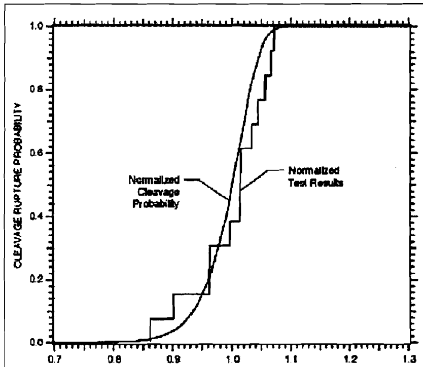
Figure 23. Summary of TC-128B Notched Round Bar Tests at -238^{\circ}\text{F} ( -150^{\circ}\text{C} ) Compared with the Normalized Cleavage Probability Curve
