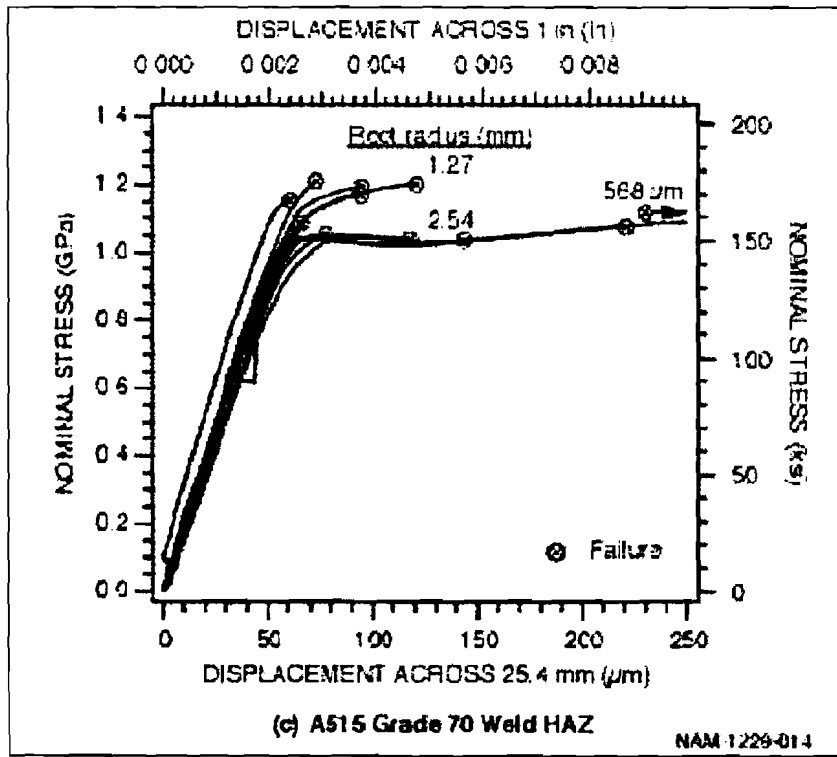
Figure 15 (continued). Tensile Stress-Displacement Curves from Notched Round Bar Laboratory Test Results
