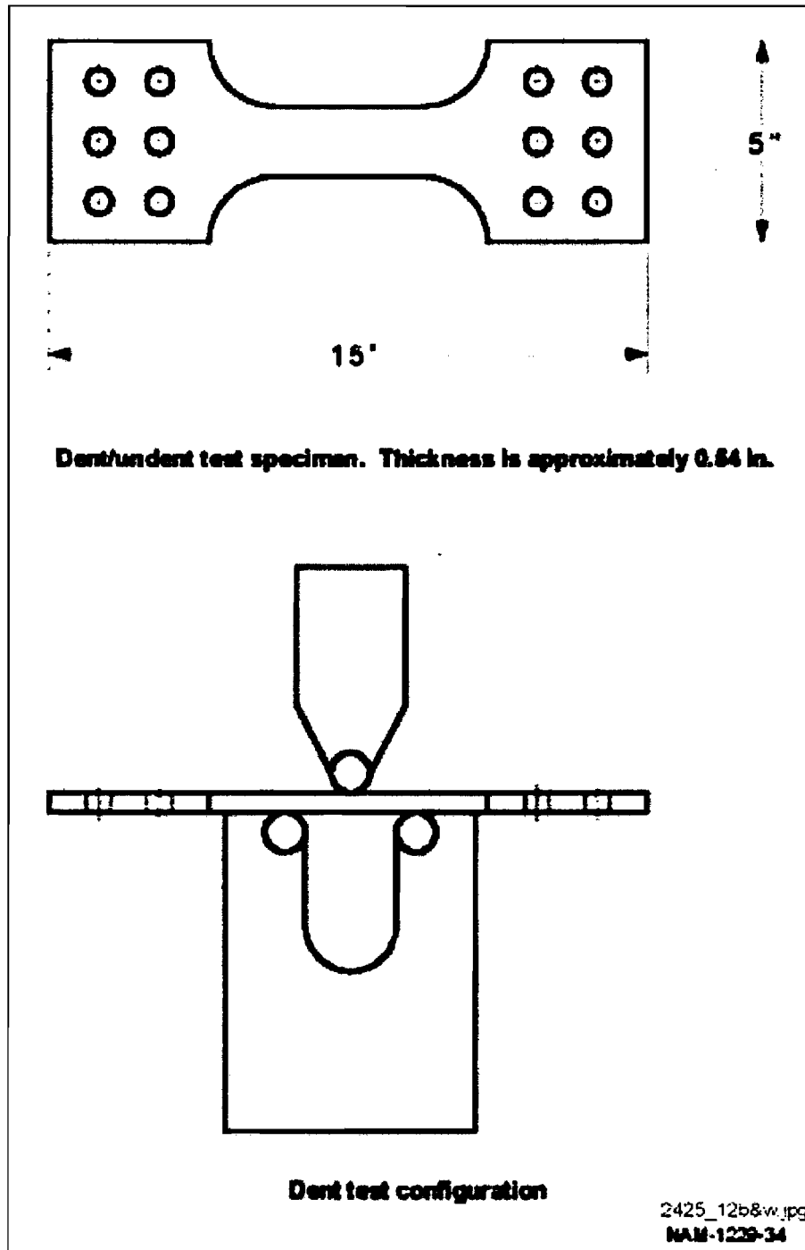
Figure 12. Specimen and Configuration for Dent/Undent Test
