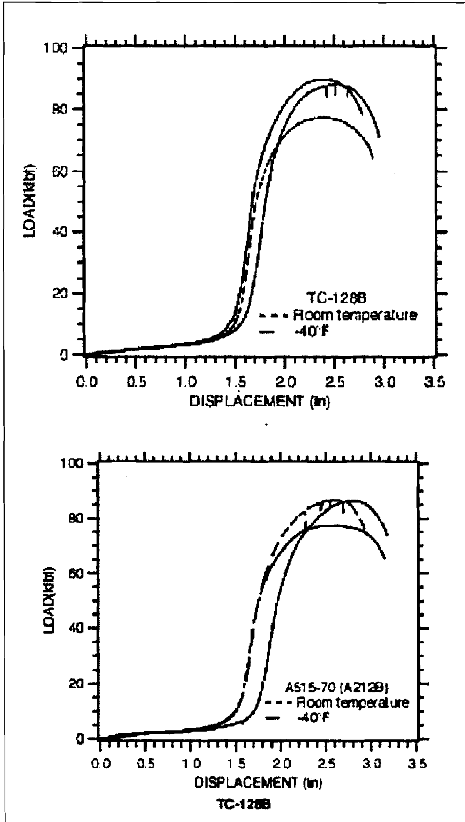
Figure 31. Results of Undenting Portion Of Dent/Undent Tests
