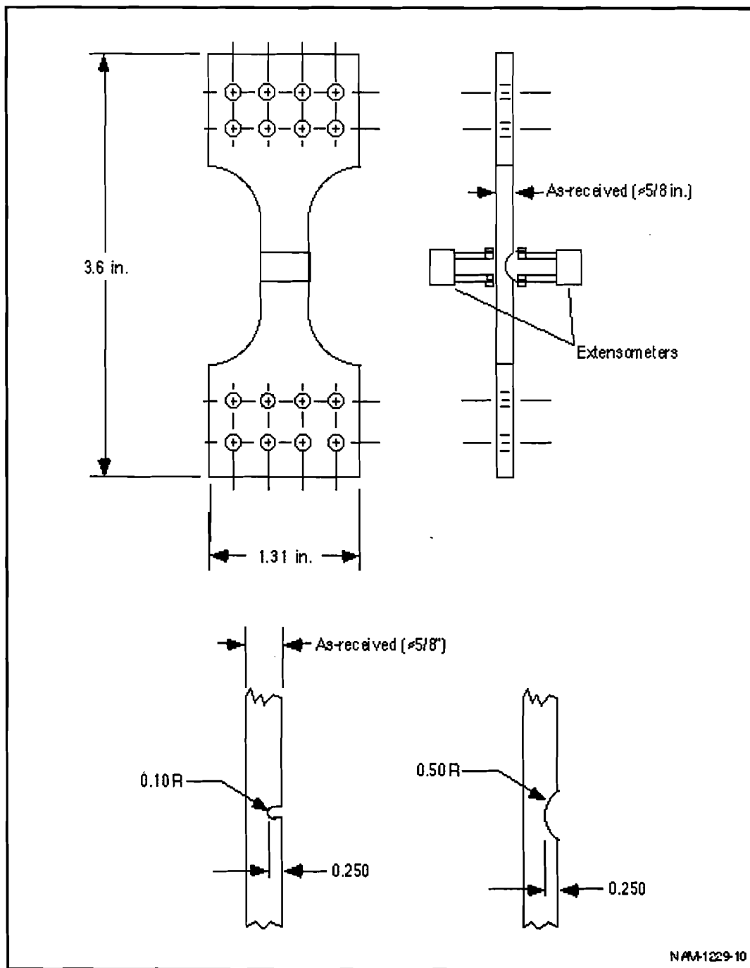
Figure 10. Simulated Gouge Specimens
