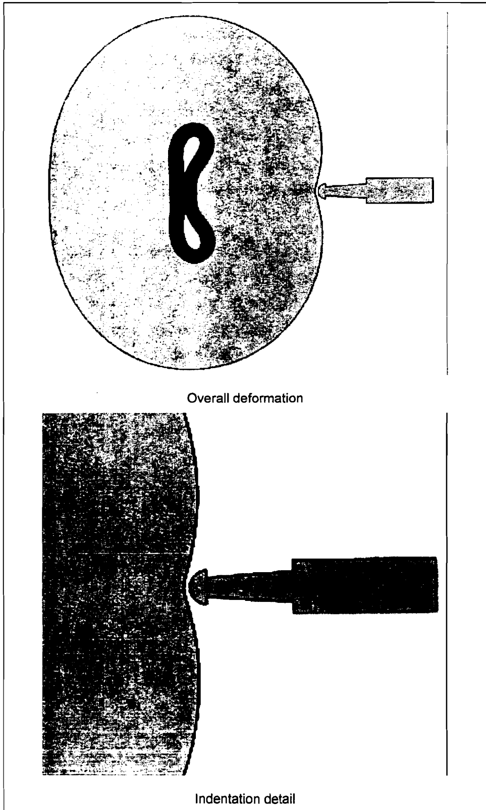
Figure 41. Unpressurized Indentation at 40 mph for an A515-70 Ring at -40° F
