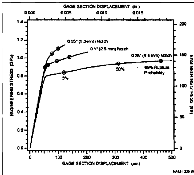
Figure 22. Calculated Notched Round Bar Stress-Displacement Curves, for TC-128B with Rupture Probabilities Indicated (-238° F or -150° C)
