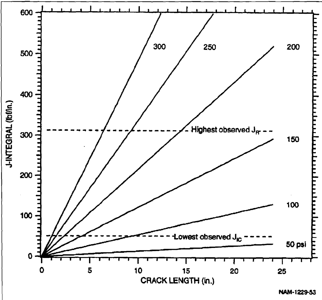
Figure 49. Applied J Versus Crack Length for Through-wall Crack
