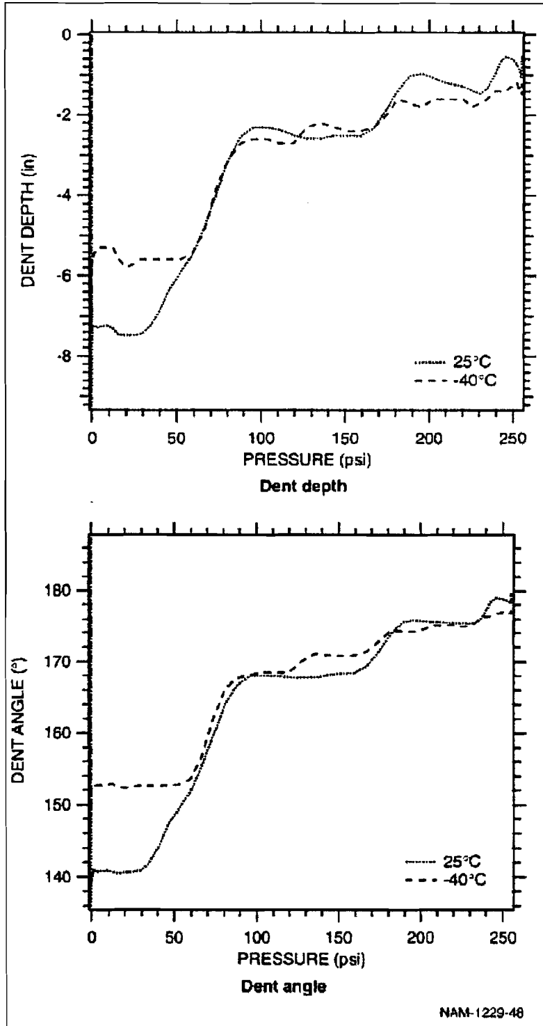
Figure 44. History of Dent Geometry with Increasing Pressure Following Impact
