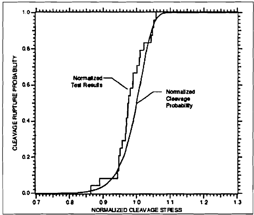
Figure 19. Summary of A515-70 Notched Round Bar Tests at -238° F (-150°) Compared with the Normalized Cleavage Probability Curve
