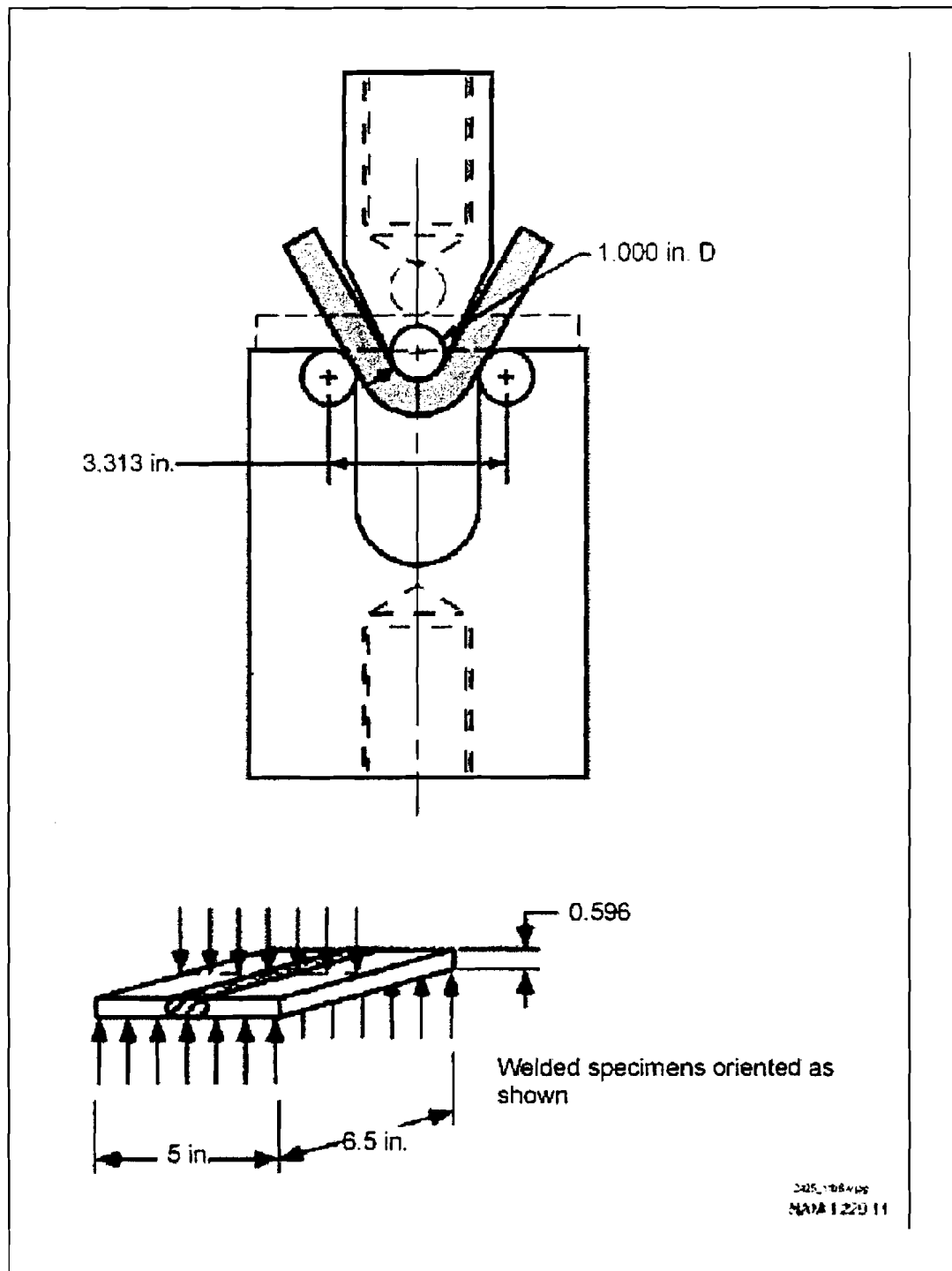
Figure 11. Bend Test Setup
