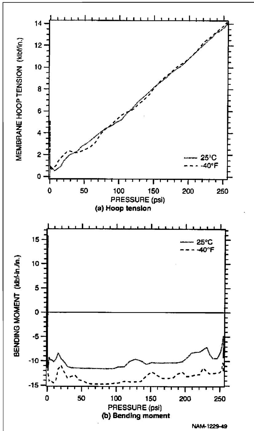
Figure 45. Dent Root Tensile Force Resultant and Bending Moment History following Impact and Subsequent Pressurization
