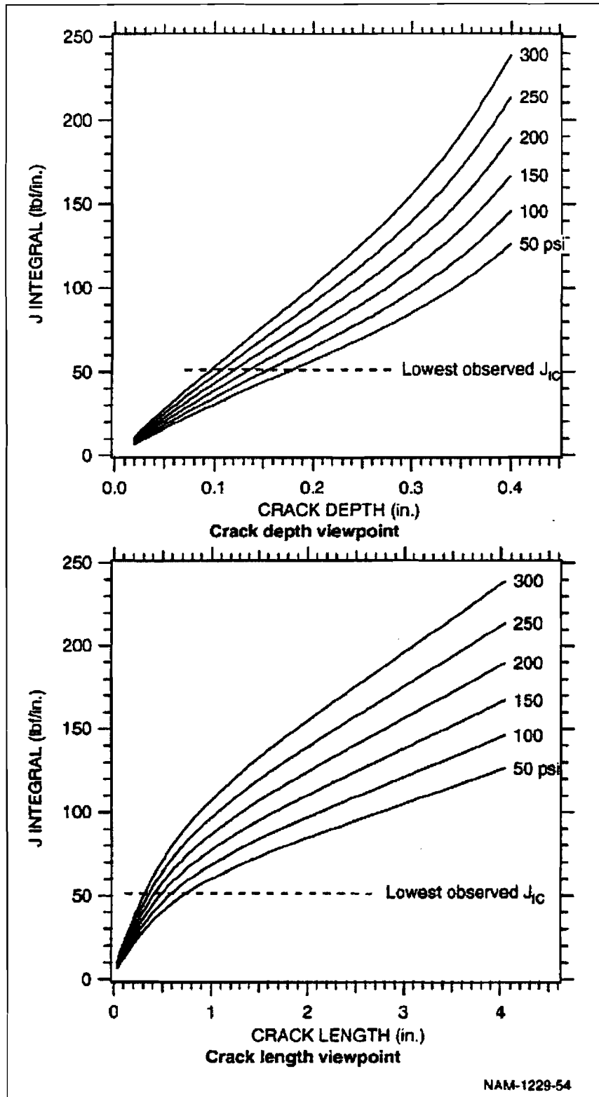
Figure 50. Applied J Versus Crack Length for Thumbnail
