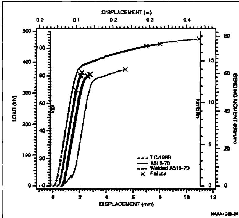
Figure 27. Results of Laboratory Cleavage Bend Tests
