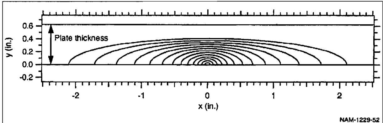
Figure 48. Profiles of Dent Root Thumbnail Cracks Growing with Constant Stress Intensity along the Crack Front for the Case of 285 psi Pressure and 15 klbf-in./in. Bending Moment
