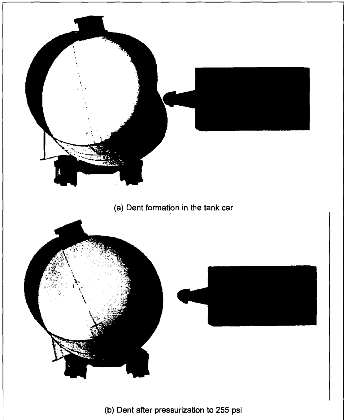
Figure 38. Analysis of a Longitudinal Dent Response with Internal Pressure
