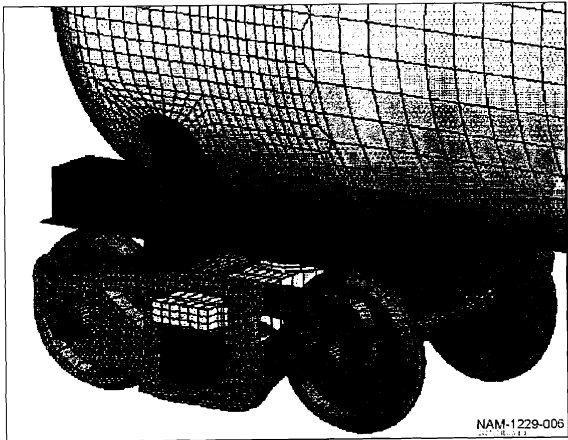
Figure 4. Detail of the Wheelset, Stub Sill, and Suspension for the Model Showing Mesh Resolution
