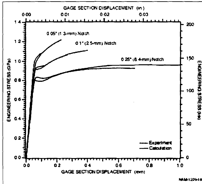
Figure 17. Calculated and Measured Notched Round Bar Stress-Displacement Curves for A515-70 (-238° F or -150° C)
