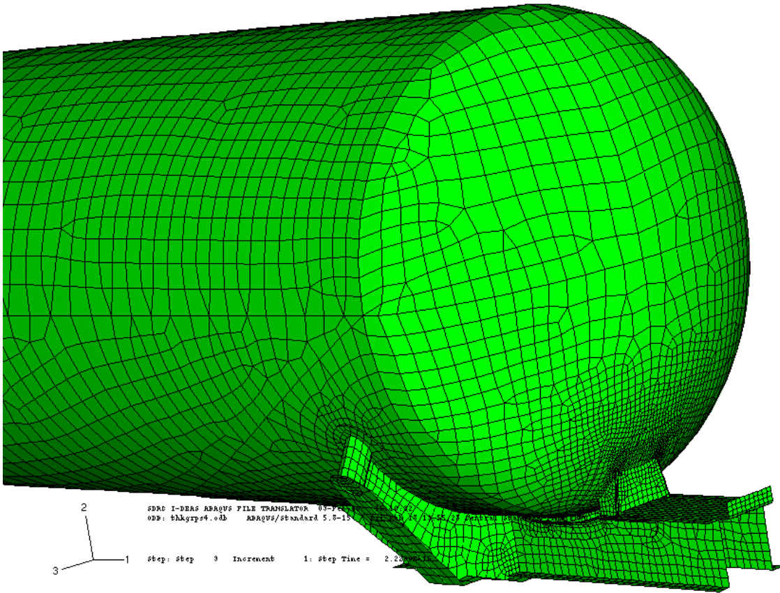
Figure 33. Static finite element model of test tank car
