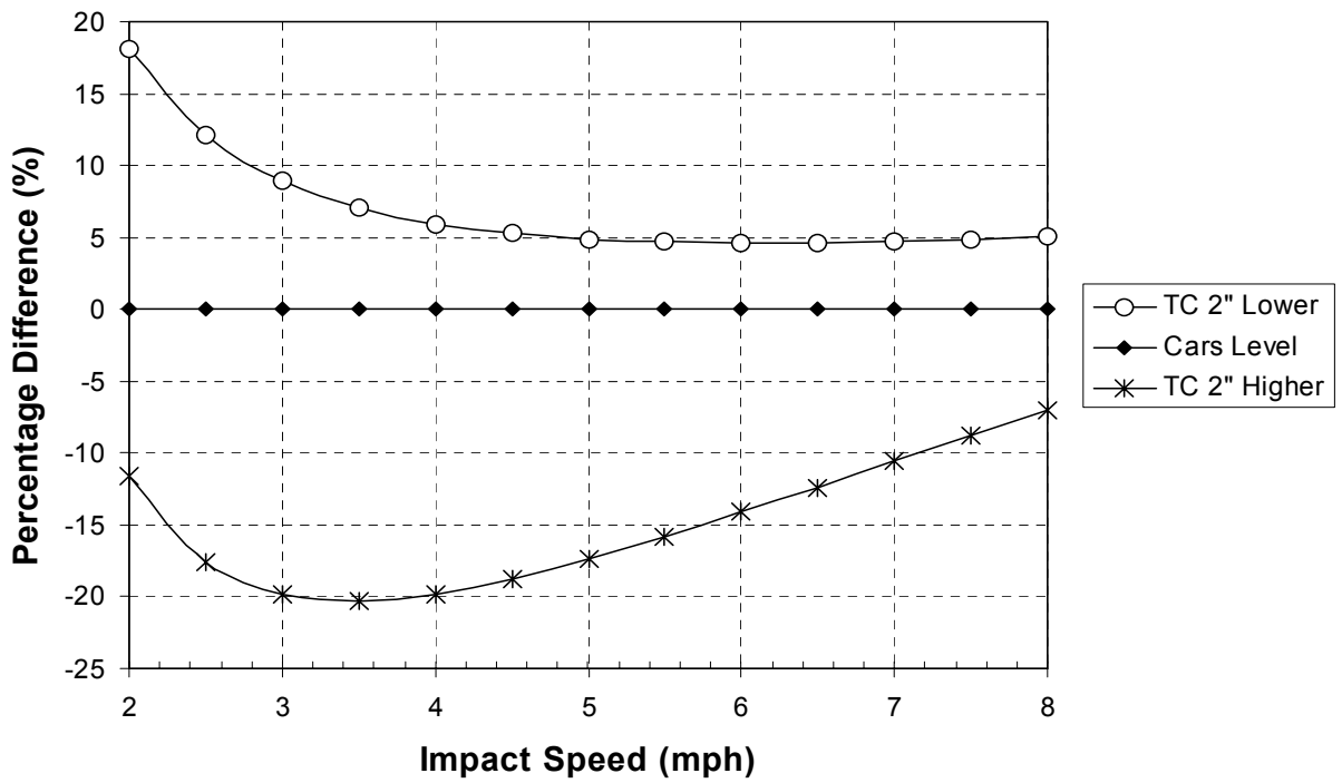
Figure 21. Variation in head pad extension (B) stresses
