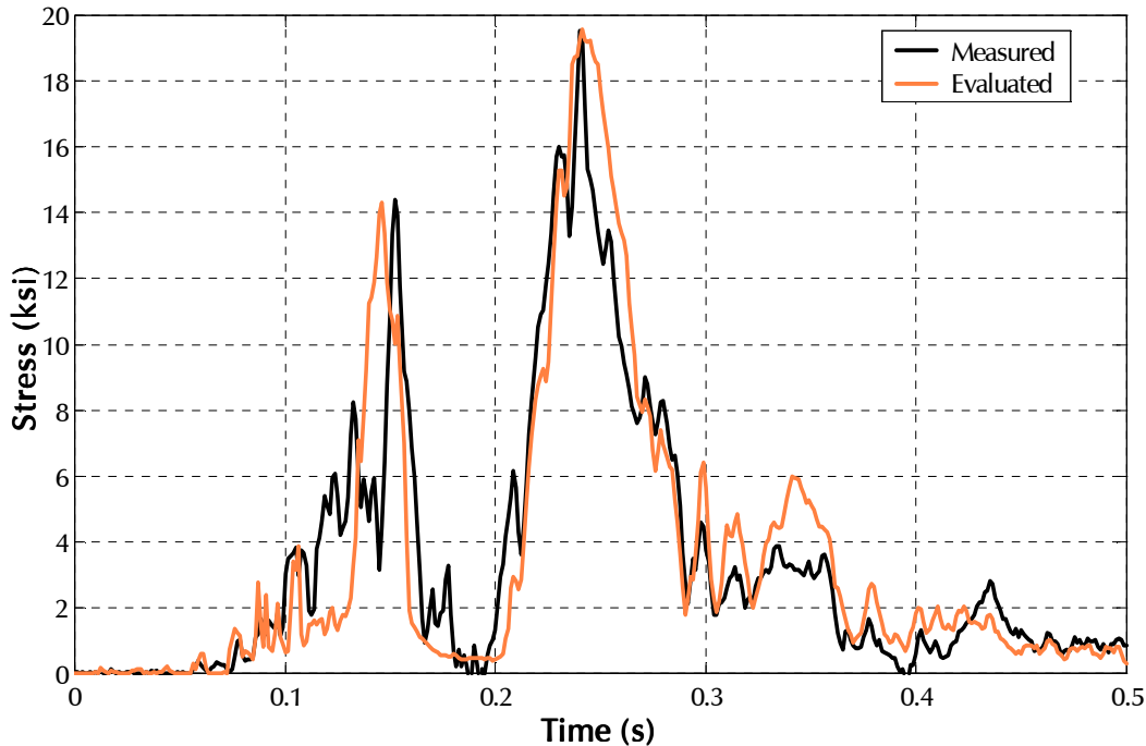
Figure 29. Comparison of stress time histories - Cars level - 8 mph impact
