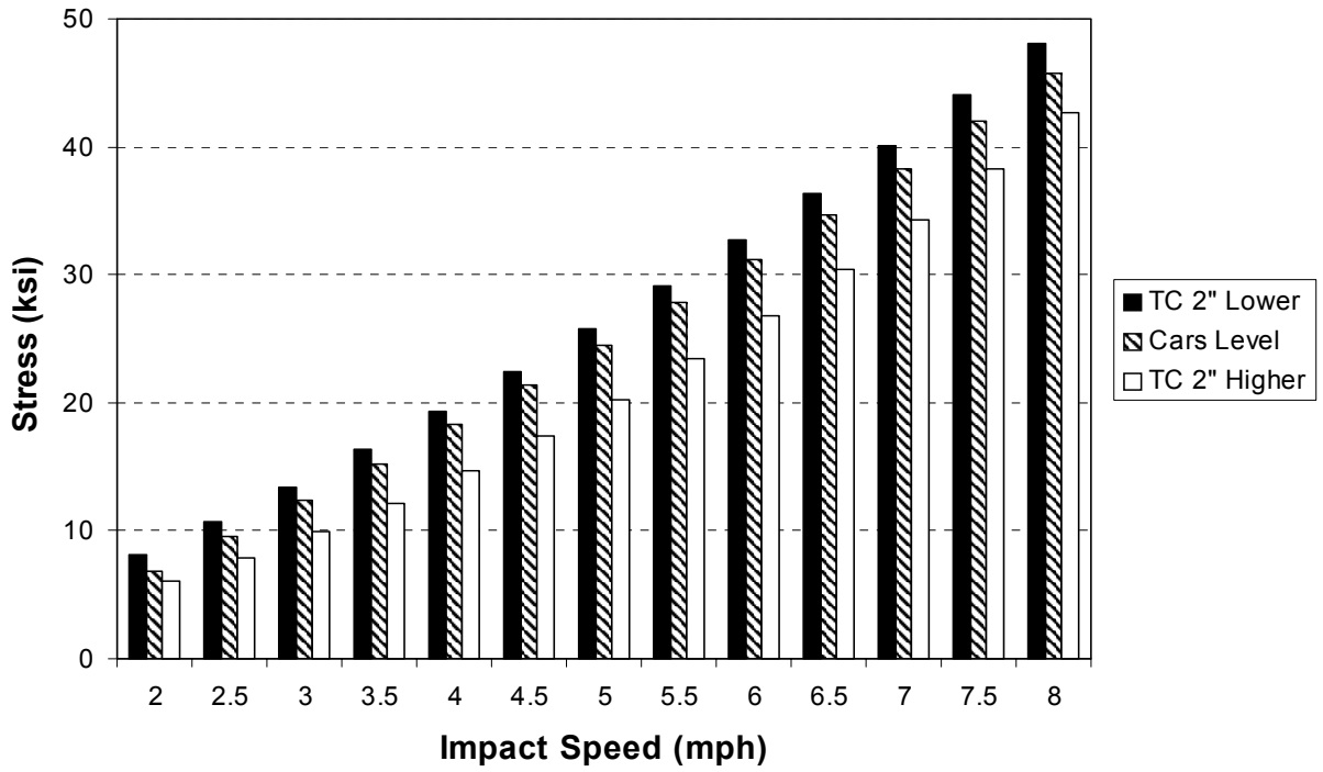
Figure 20. Principal stresses at the head pad extension (B) - Averaged
