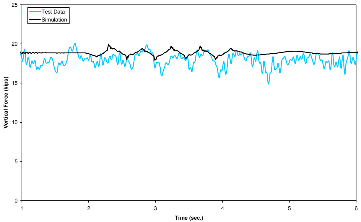
Figure B-24(c). Yaw and sway - vertical force time history, 60 mph (trailing left wheel)
