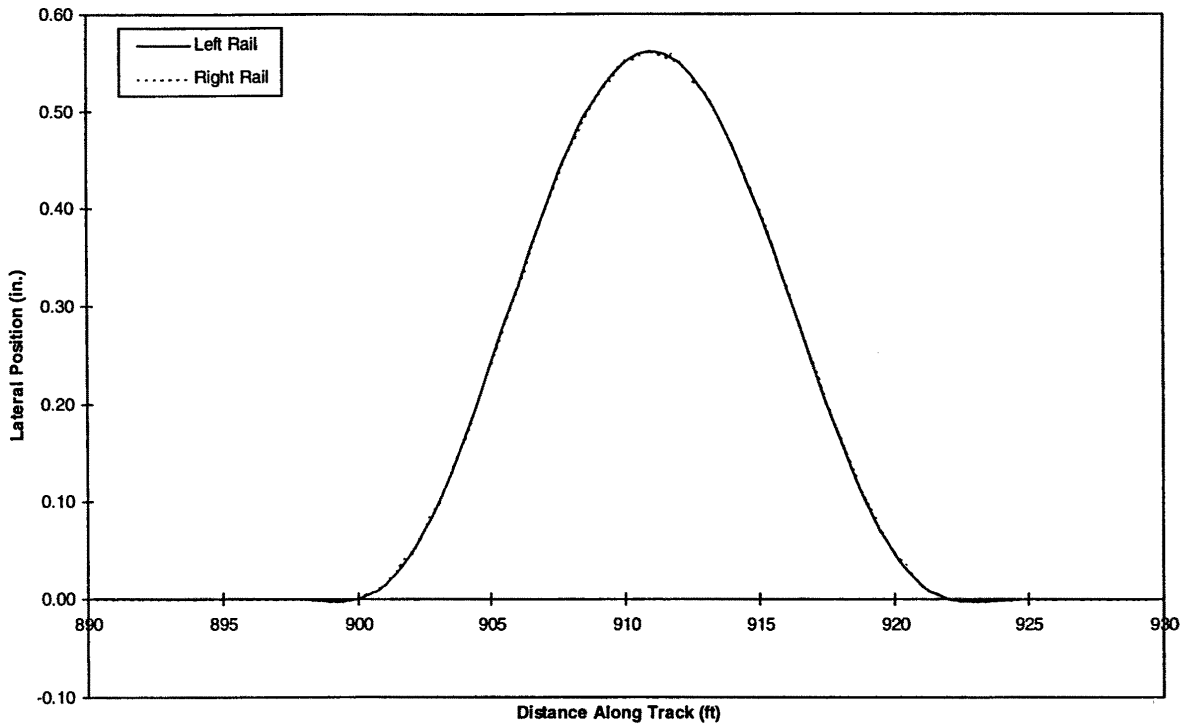
Figure 16. Lateral perturbation for hunting test
