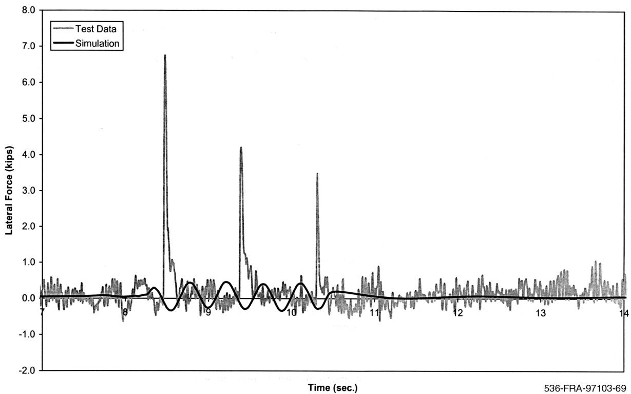
Figure A-22(a). Yaw and sway - lateral force time history, 60 mph (lead left wheel)
