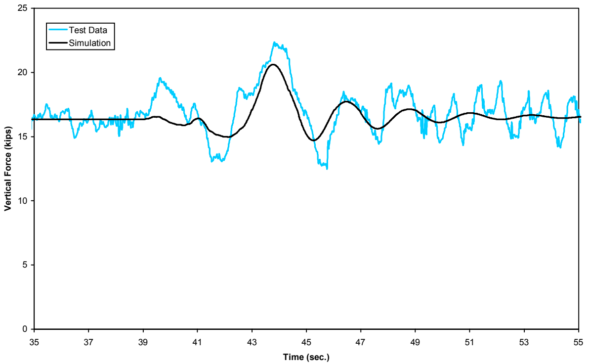
Figure B-3(c). Vertical bump test - vertical force time history, 15 mph (trailing outer wheel)
