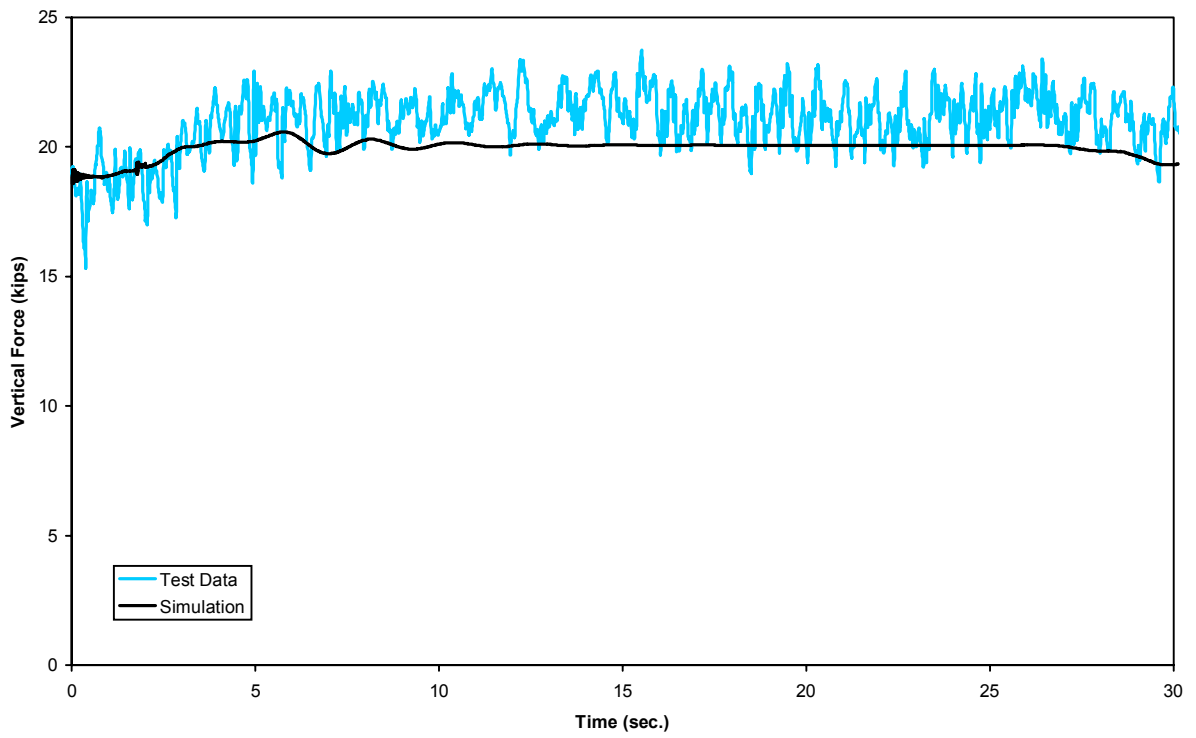
Figure B-9(c). Constant curving - vertical force time history, 32 mph (trailing outer wheel)
