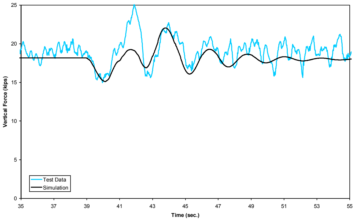
Figure B-3(a). Vertical bump test - vertical force time history, 15 mph (lead outer wheel)
