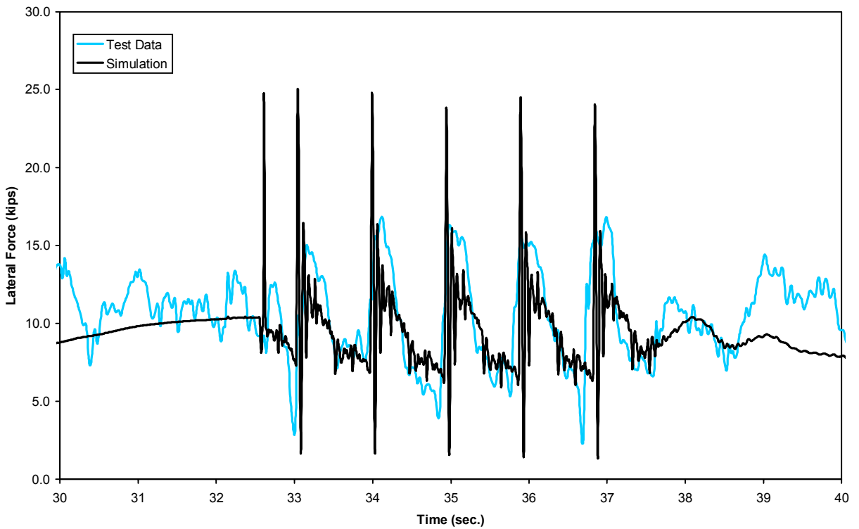
Figure B-18(a). Dynamic curving - lateral force time history, 28 mph (lead outer wheel)
