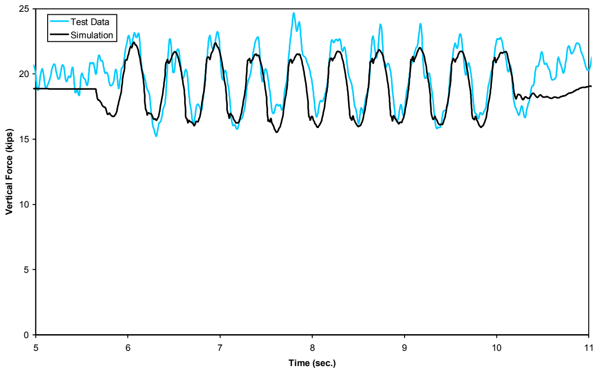
Figure B-31(a). Twist and roll - vertical force time history, 60 mph (lead left wheel)
