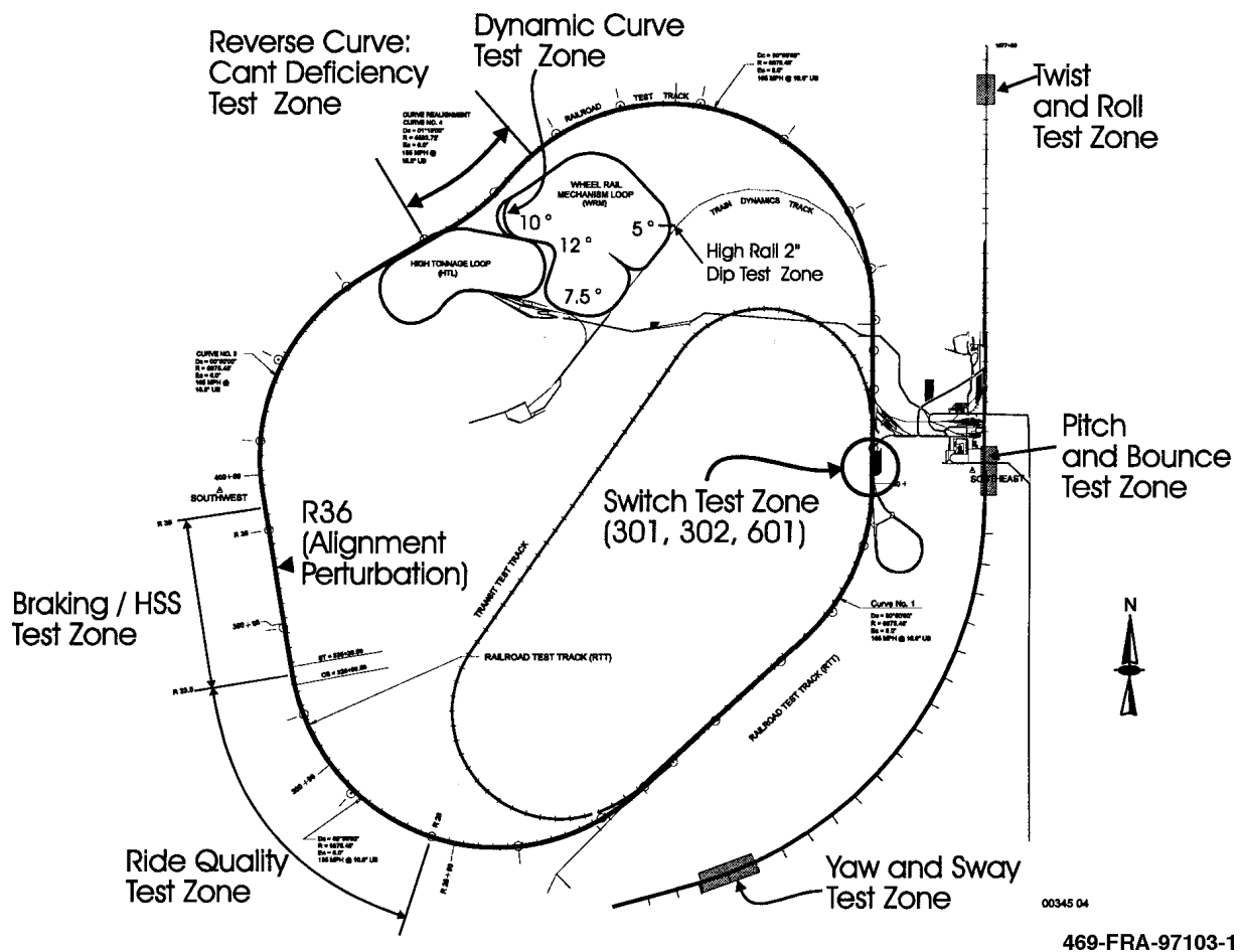
Figure 9. TTC test tracks
