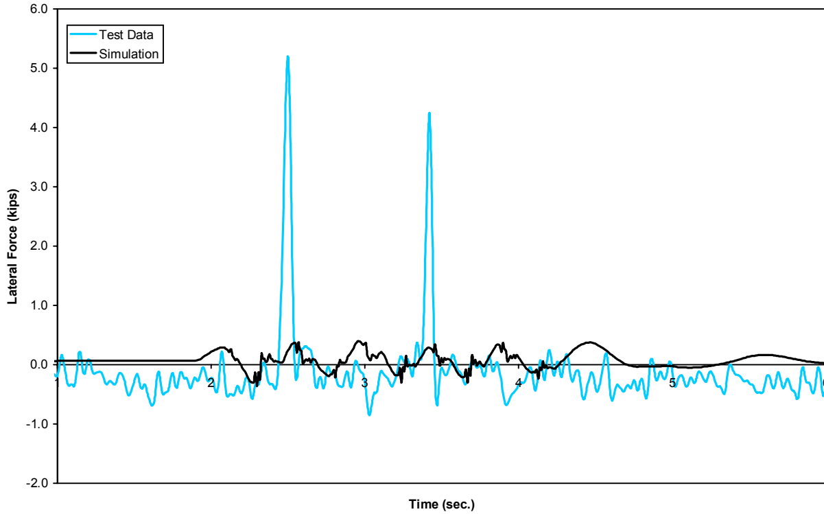
Figure B-25(b). Yaw and sway - lateral force time history, 60 mph (lead right wheel)
