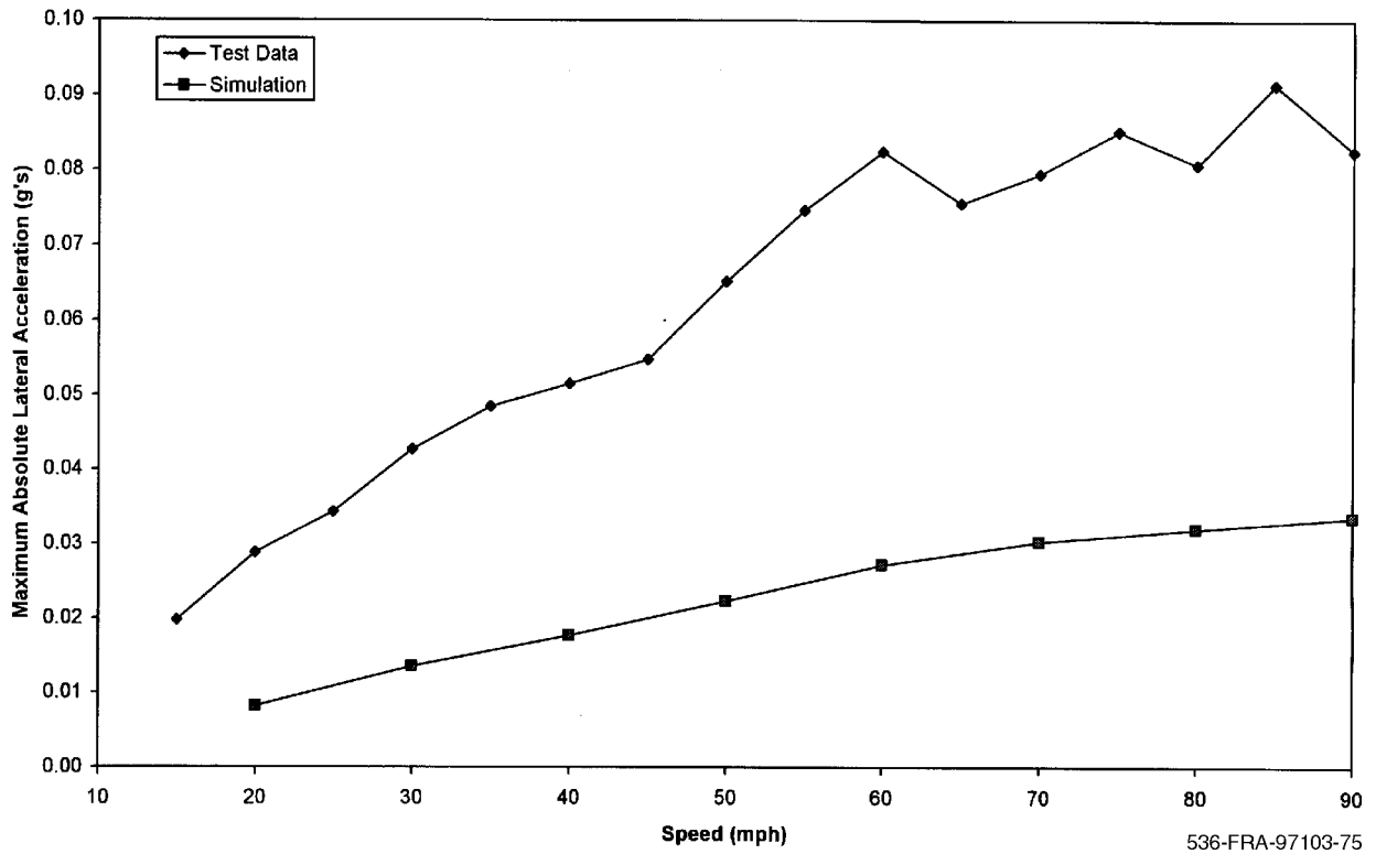
Figure A-25. Yaw and sway - maximum absolute lateral car body acceleration ("B" end)
