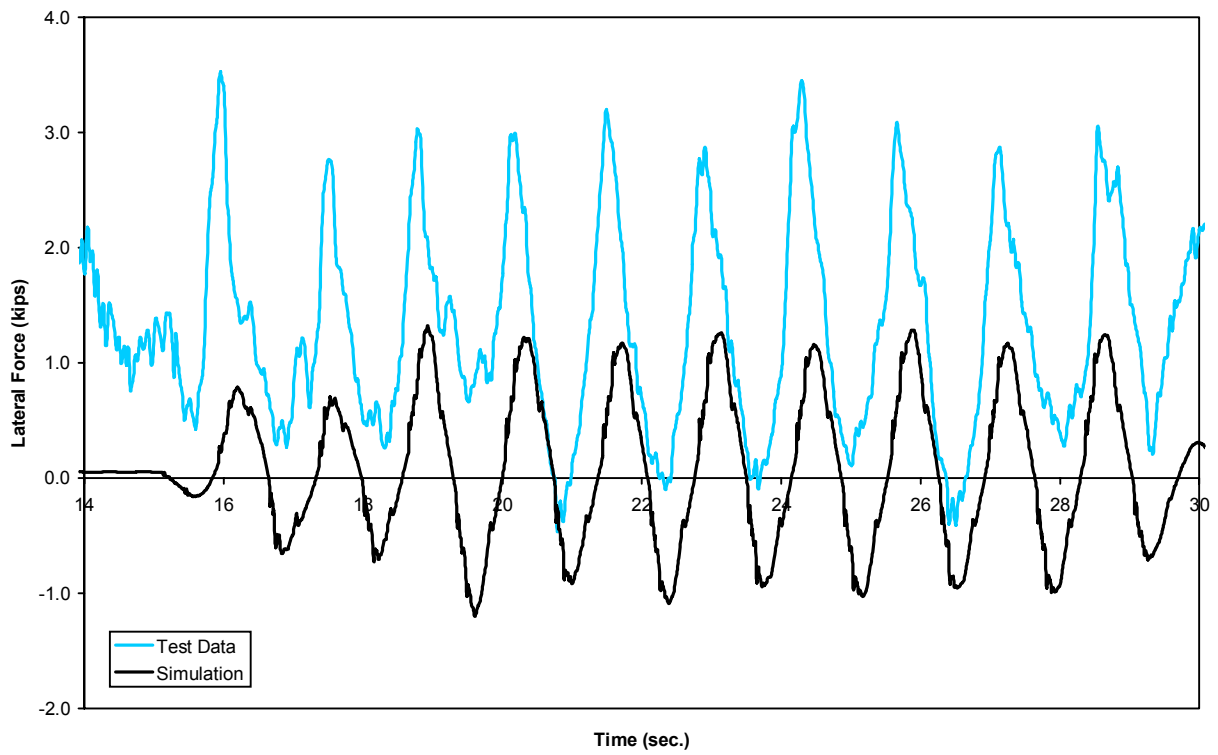
Figure B-30(a). Twist and roll - lateral force time history, 19.2 mph (lead left wheel)
