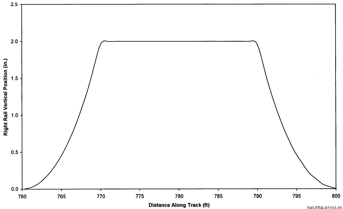
Figure 17. Vertical bump in the 7.5 deg curve
