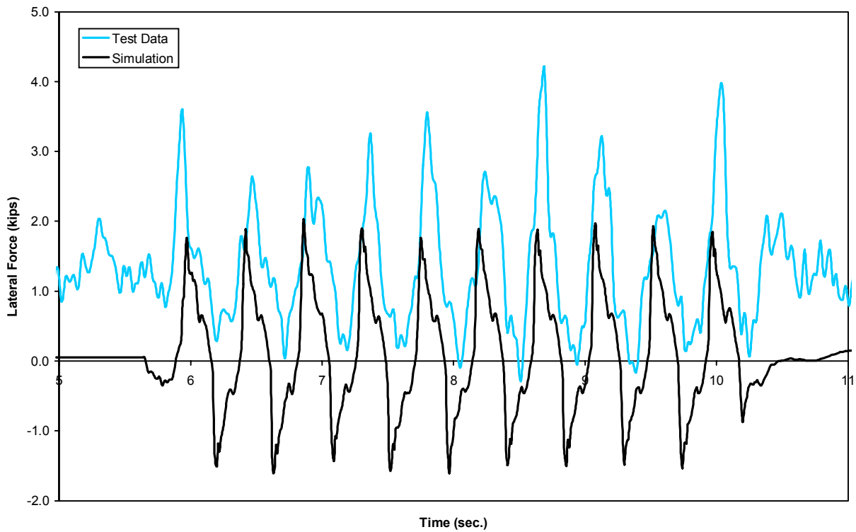
Figure B-32(a). Twist and roll - lateral force time history, 60 mph (lead left wheel)
