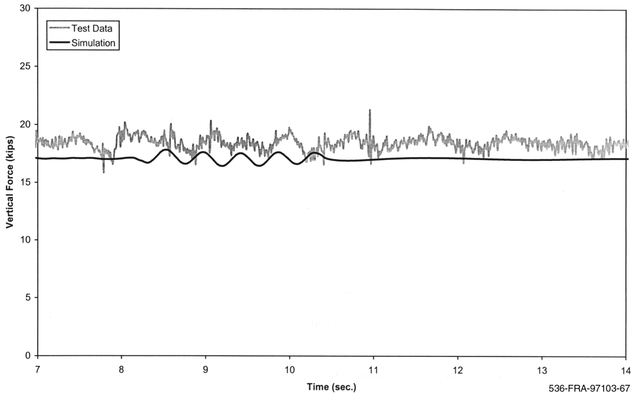
Figure A-21(c). Yaw and sway - vertical force time history, 60 mph (trailing left wheel)
