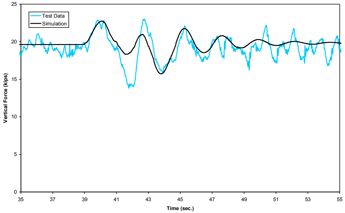
Figure B-3(b). Vertical bump test - vertical force time history, 15 mph (lead inner wheel)
