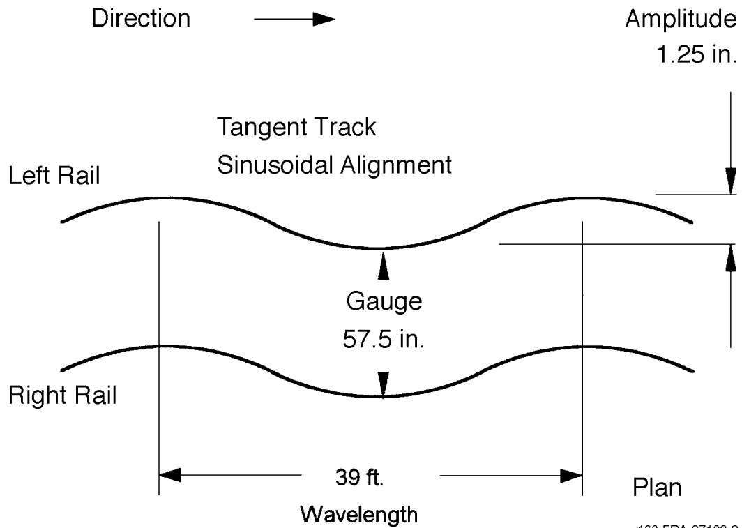
Figure 13. Track alignment variation for yaw and sway
