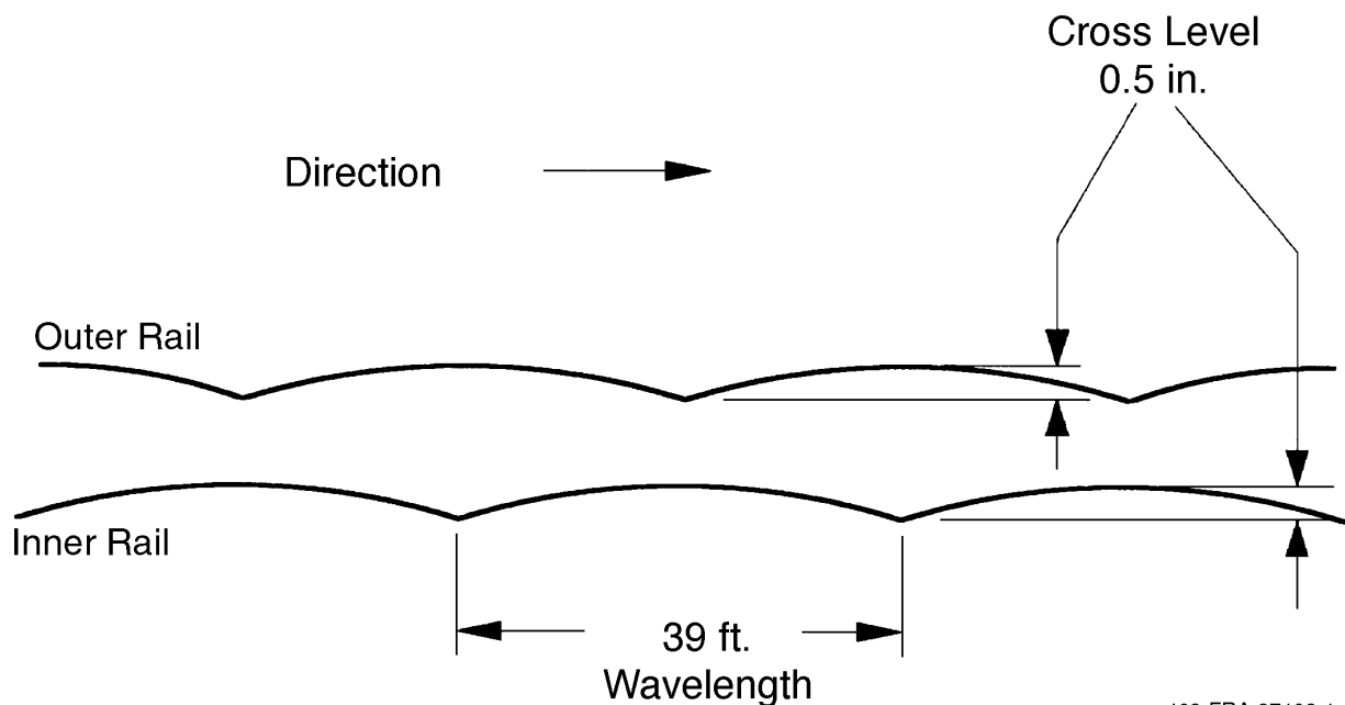
Figure 11. Crosslevel variation for dynamic curving
