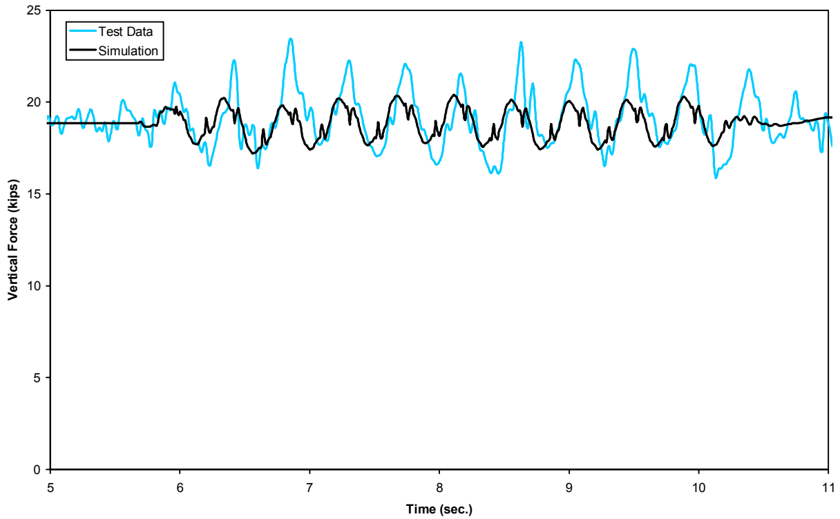
Figure B-31(d). Twist and roll - vertical force time history, 60 mph (trailing right wheel)
