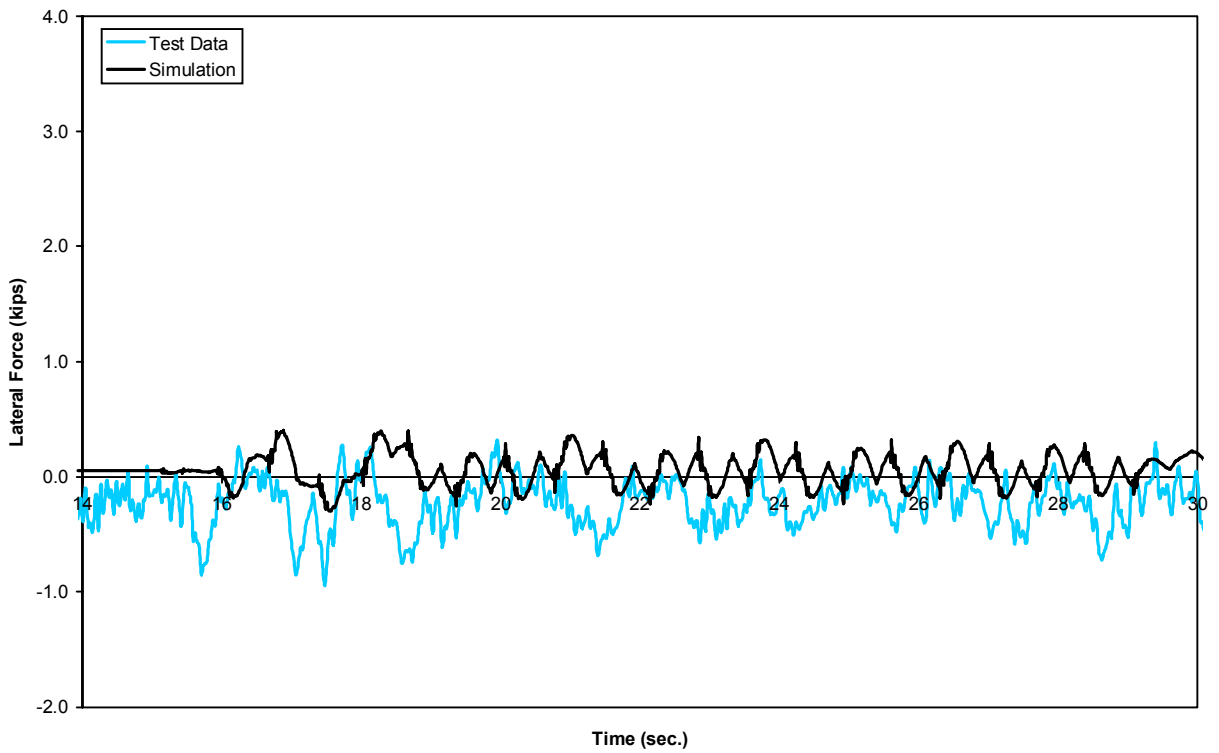
Figure B-30(c). Twist and roll - lateral force time history, 19.2 mph (trailing left wheel)
