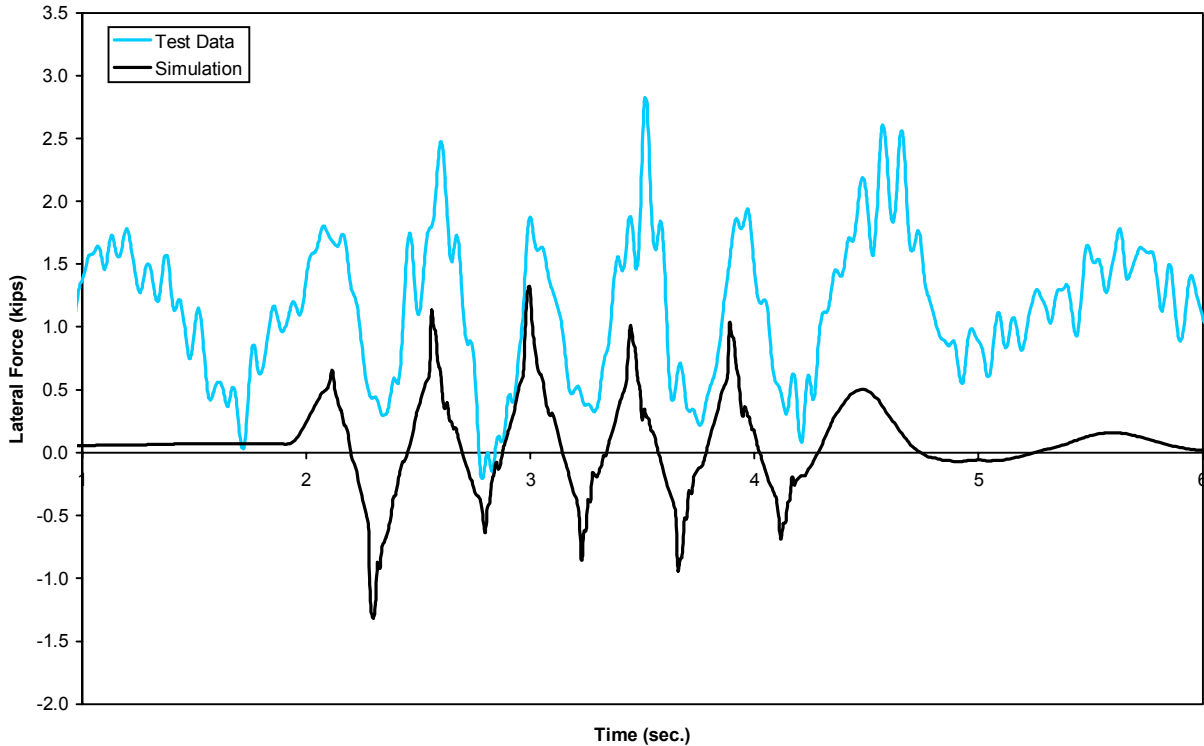
Figure B-25(d). Yaw and sway - lateral force time history, 60 mph (trailing right wheel)
