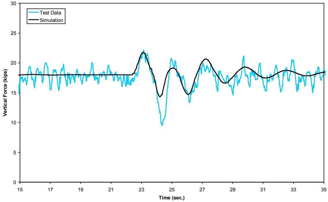
Figure B-1(b). Vertical bump test - vertical force time history, 24 mph (lead inner wheel)
