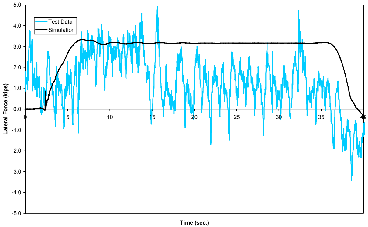
Figure B-8(a). Constant curving - net axle lateral force time history, 24 mph (lead axle)
