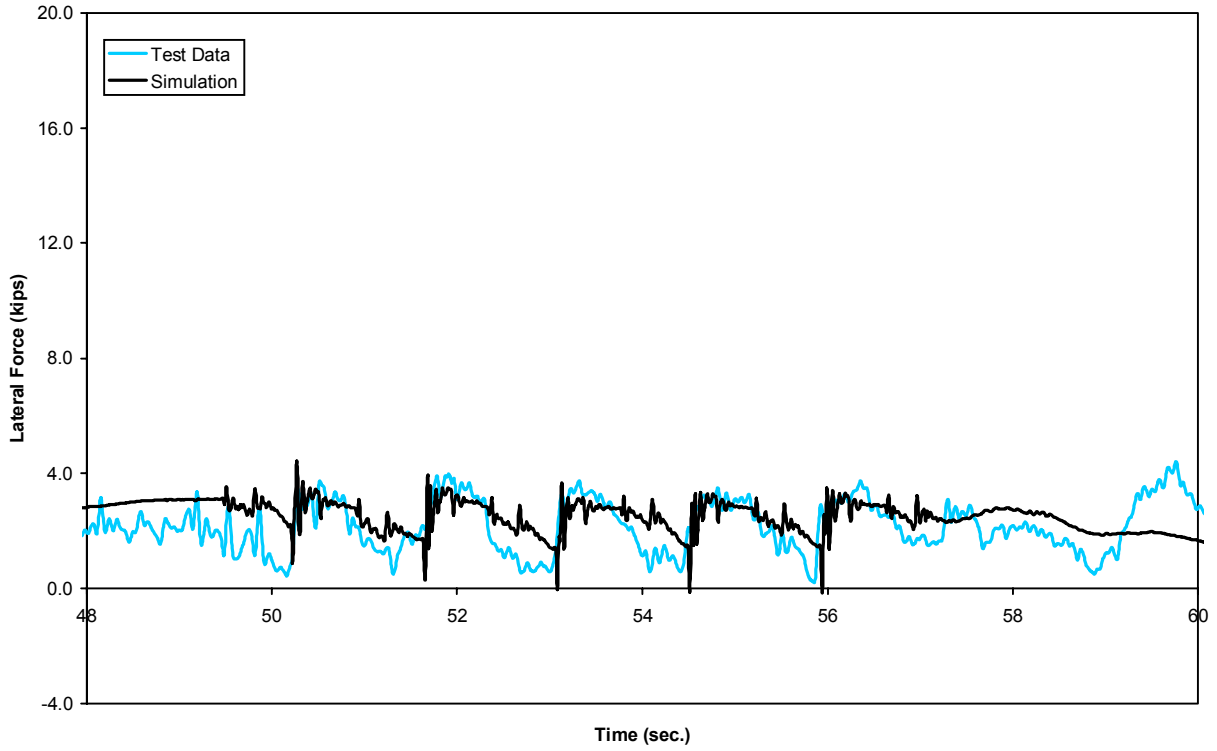
Figure B-16(d). Dynamic curving - lateral force time history, 18.6 mph (trailing inner wheel)
