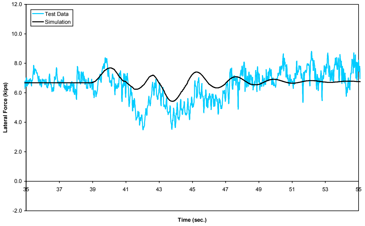
Figure B-4(b). Vertical bump test - lateral force time history, 15 mph (lead inner wheel)
