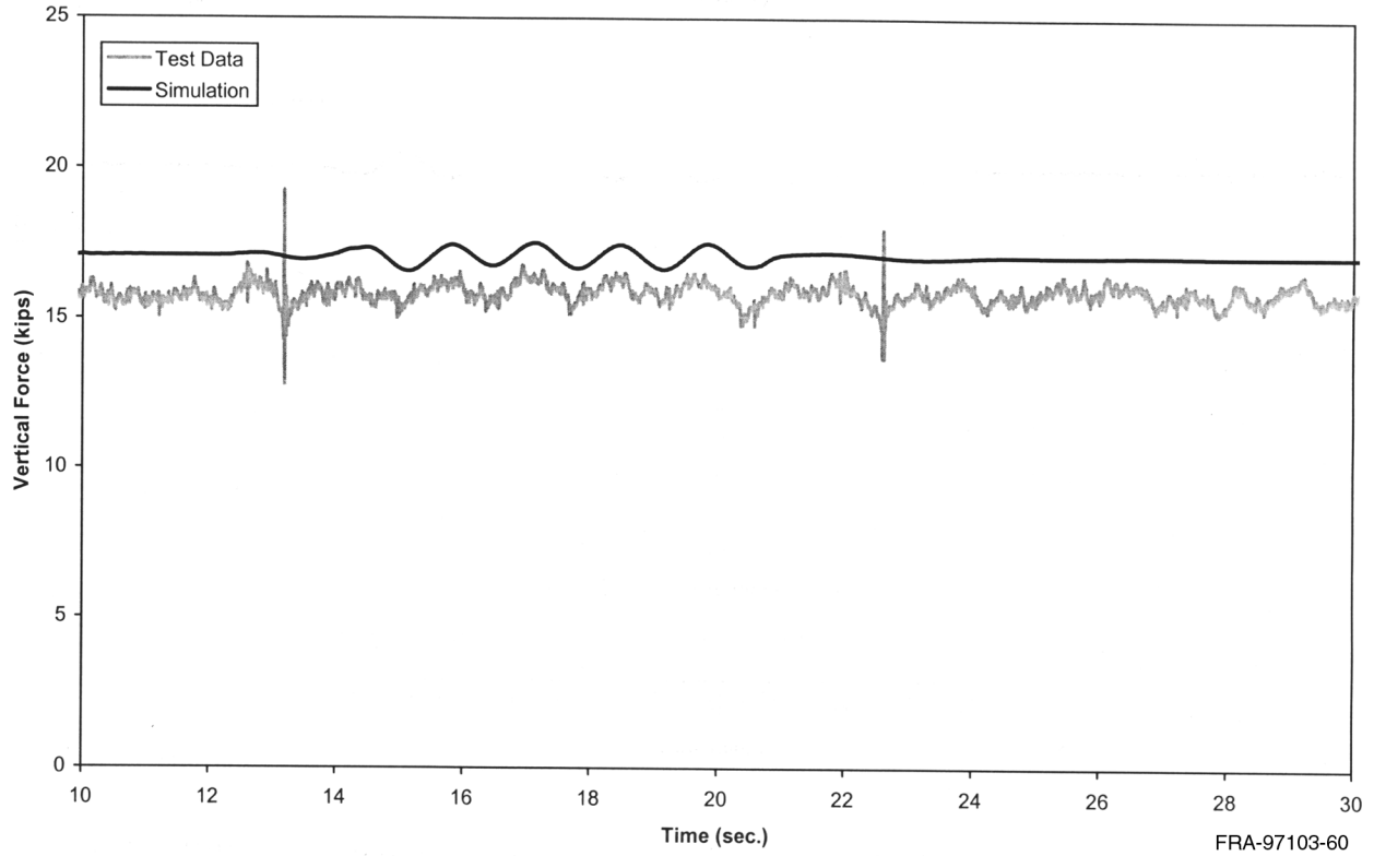
Figure A-19(d). Yaw and sway - vertical force time history, 20 mph (trailing right wheel)
