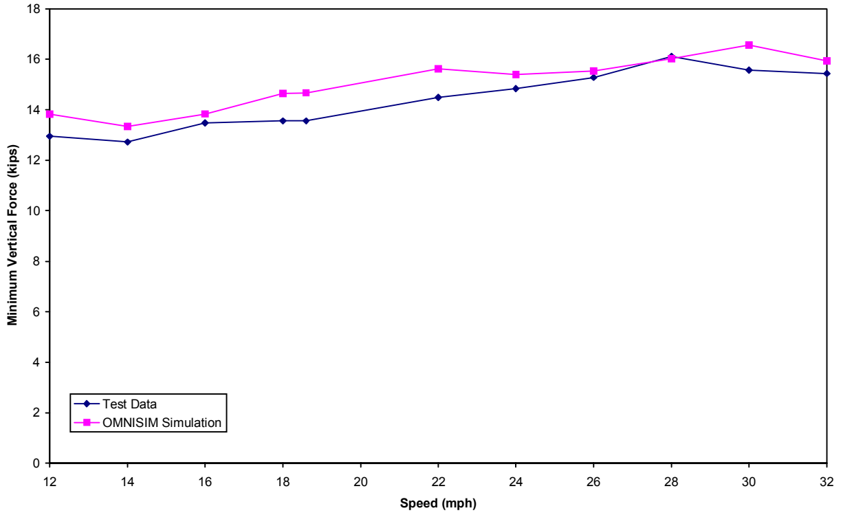
Figure B-19. Dynamic curving - minimum vertical force
