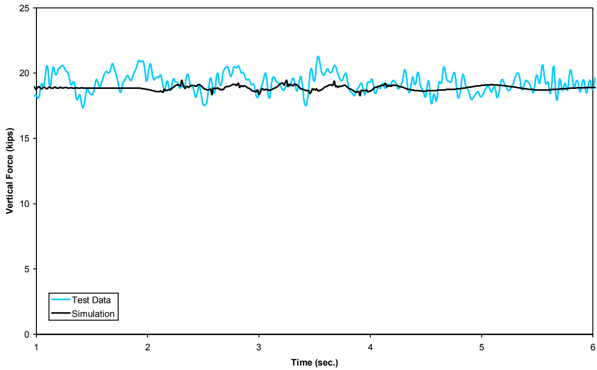
Figure B-24(a). Yaw and sway - vertical force time history, 60 mph (lead left wheel)
