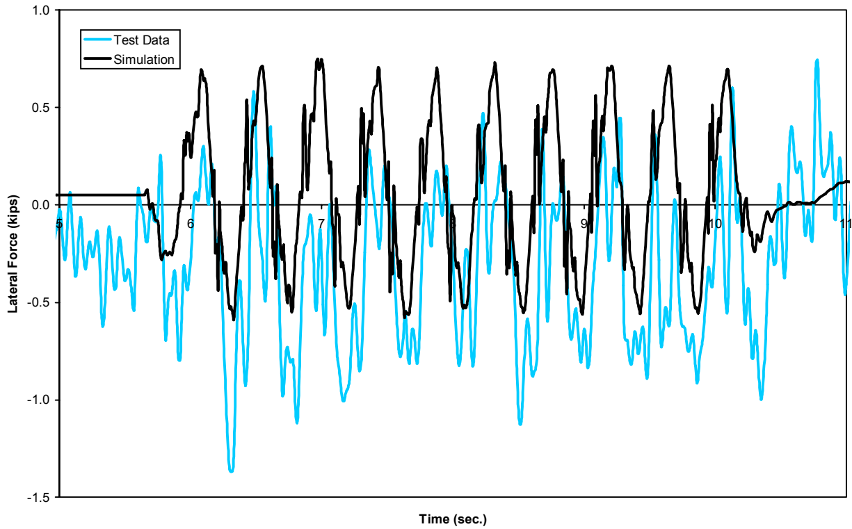
Figure B-32(c). Twist and roll - lateral force time history, 60 mph (trailing left wheel)
