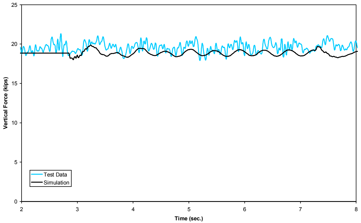
Figure B-37(a). Pitch and bounce - vertical force time history, 60 mph (lead left wheel)
