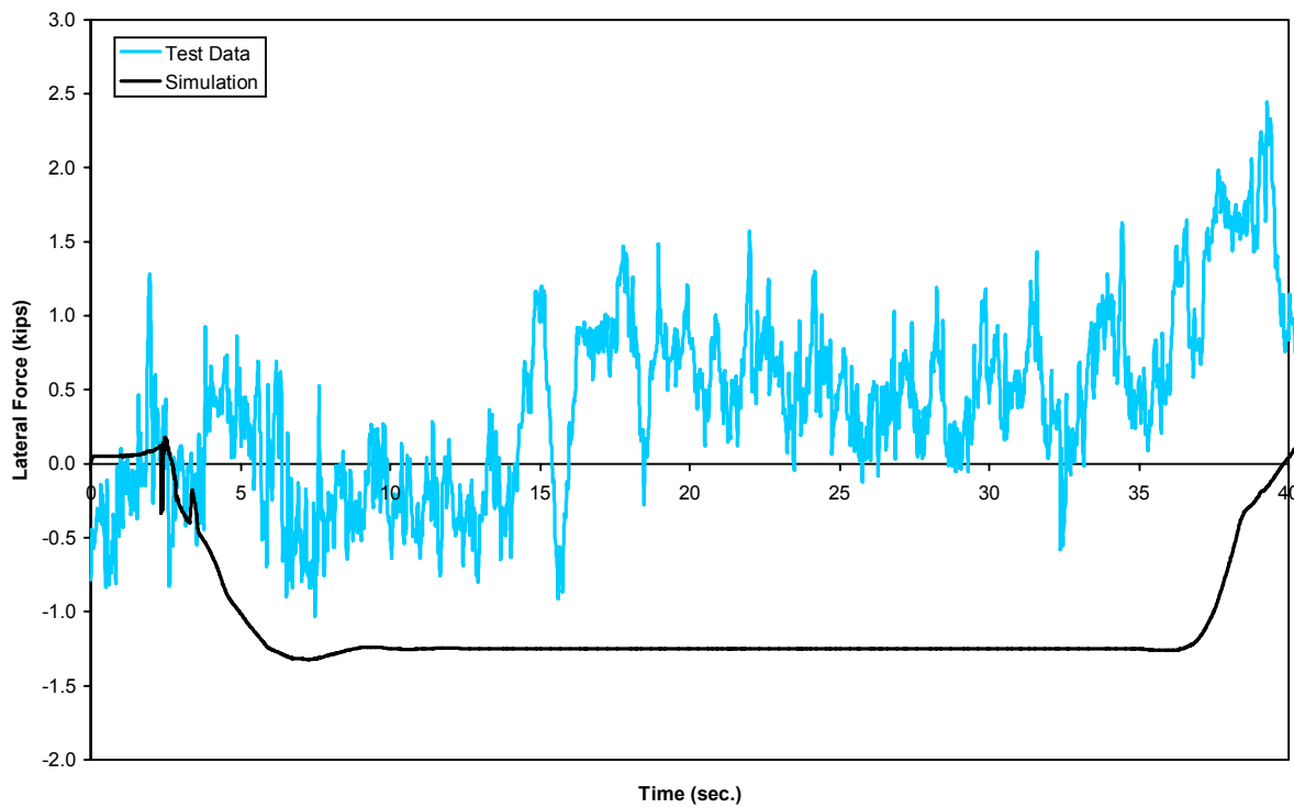
Figure B-7(c). Constant curving - lateral force time history, 24 mph (trailing outer wheel)
