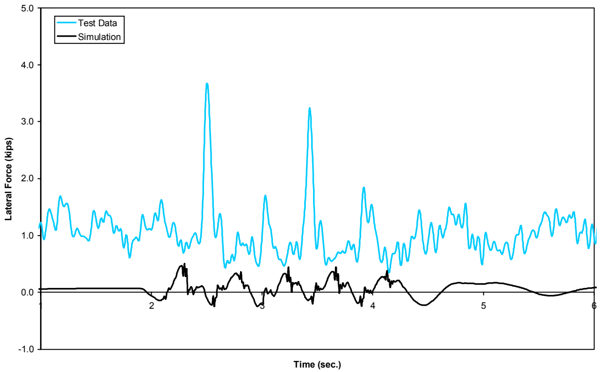
Figure B-25(a). Yaw and sway - lateral force time history, 60 mph (lead left wheel)
