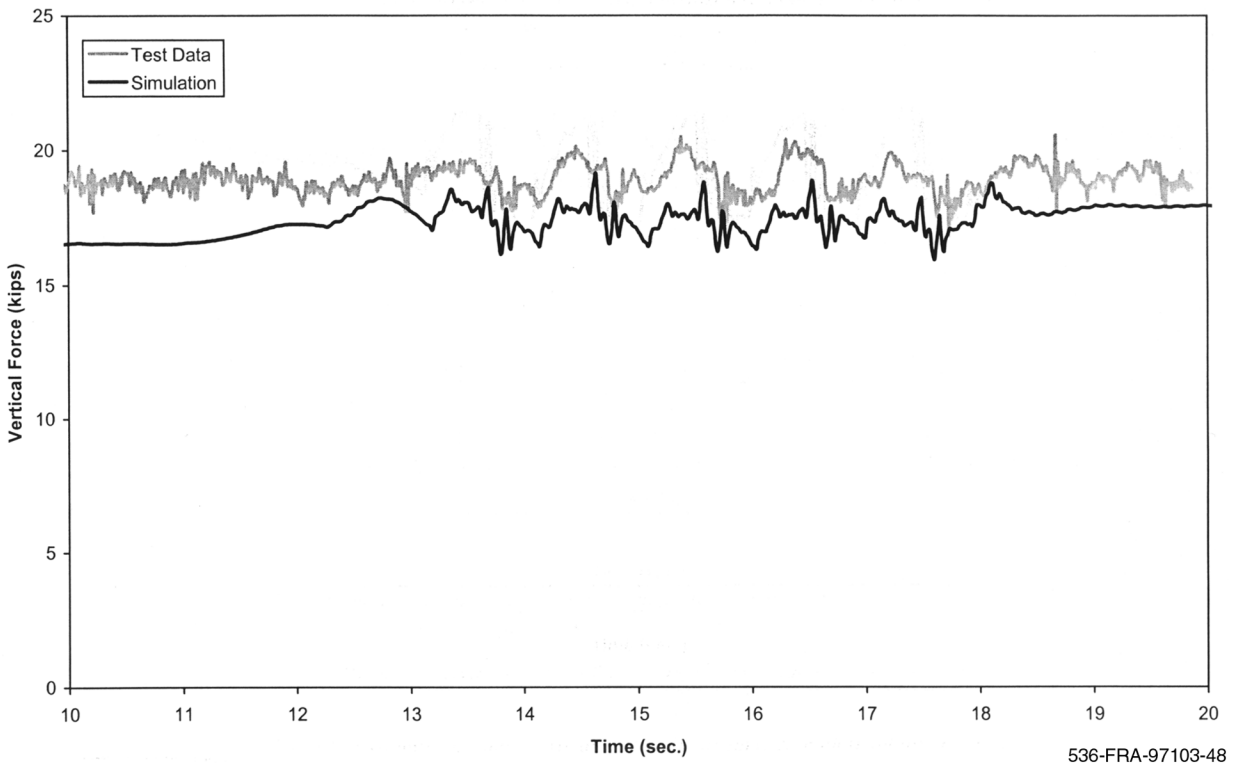
Figure A-14(c). Dynamic curving - vertical force time history, 28 mph (trailing outer wheel)
