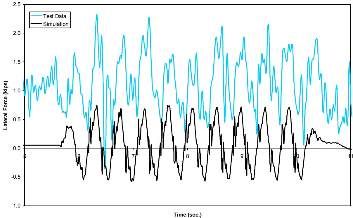
Figure B-32(d). Twist and roll - lateral force time history, 60 mph (trailing right wheel)
