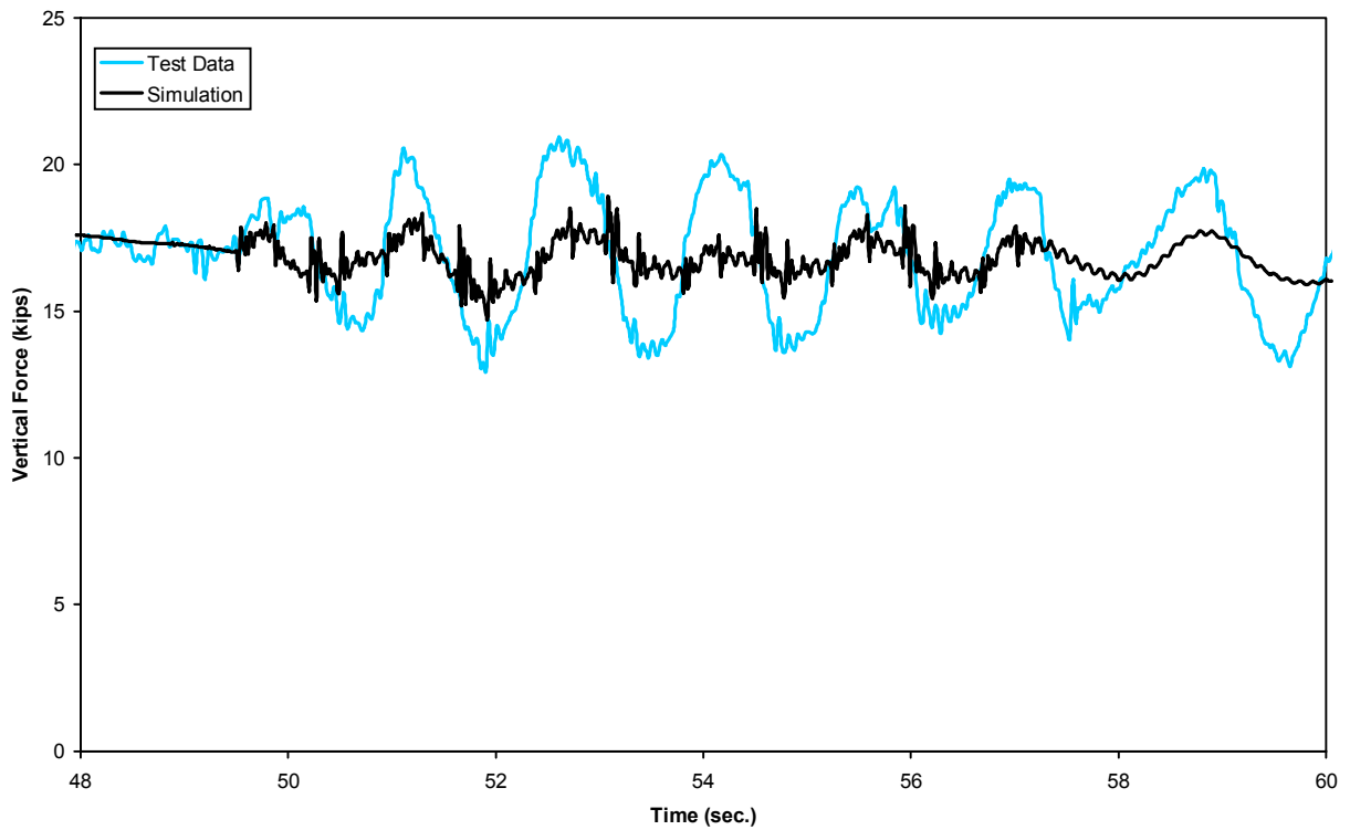
Figure B-15(c). Dynamic curving - vertical force time history, 18.6 mph (trailing outer wheel)
