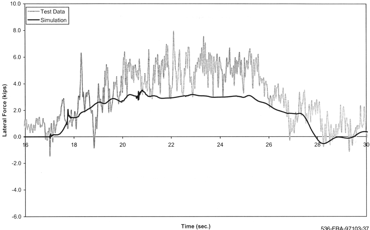
Figure A-11(b). Steady curving - net axle lateral force time history, 124 mph (trailing axle)
