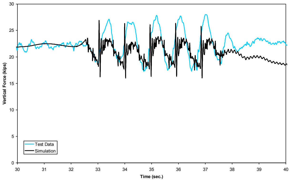
Figure B-17(a). Dynamic curving - vertical force time history, 28 mph (lead outer wheel)
