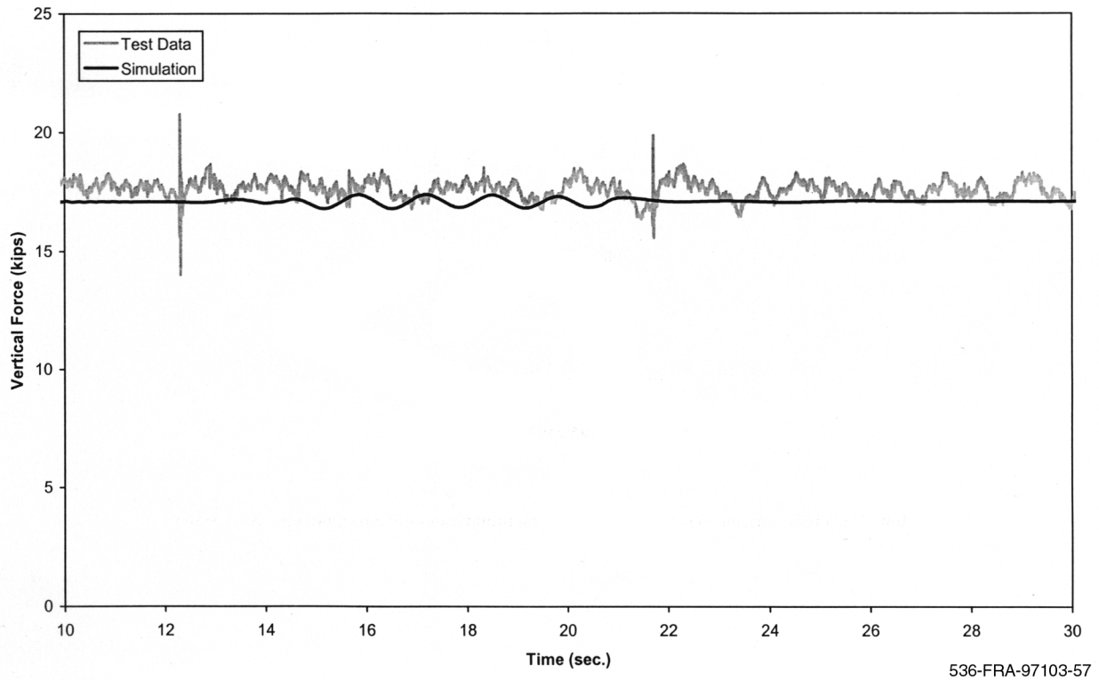
Figure A-19(a). Yaw and sway - vertical force time history, 20 mph (lead left wheel)
