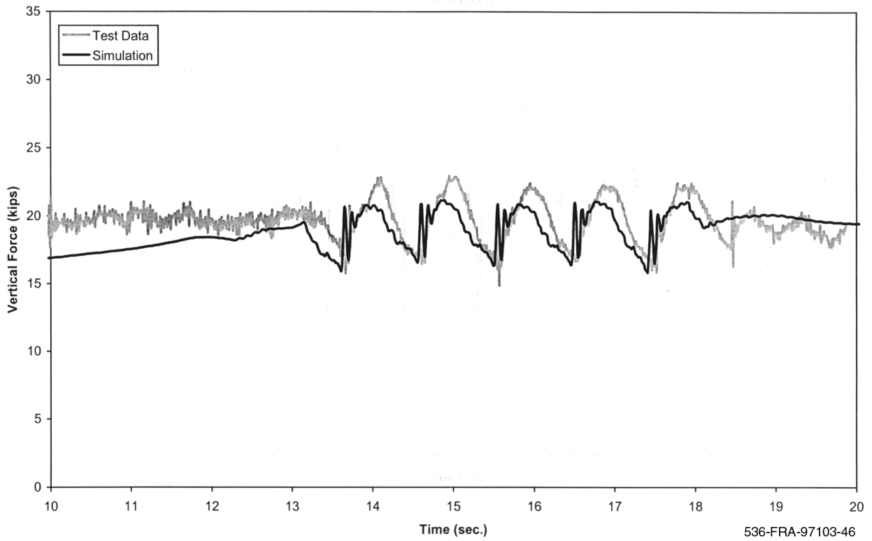
Figure A-14(a). Dynamic curving - vertical force time history, 28 mph (lead outer wheel)
