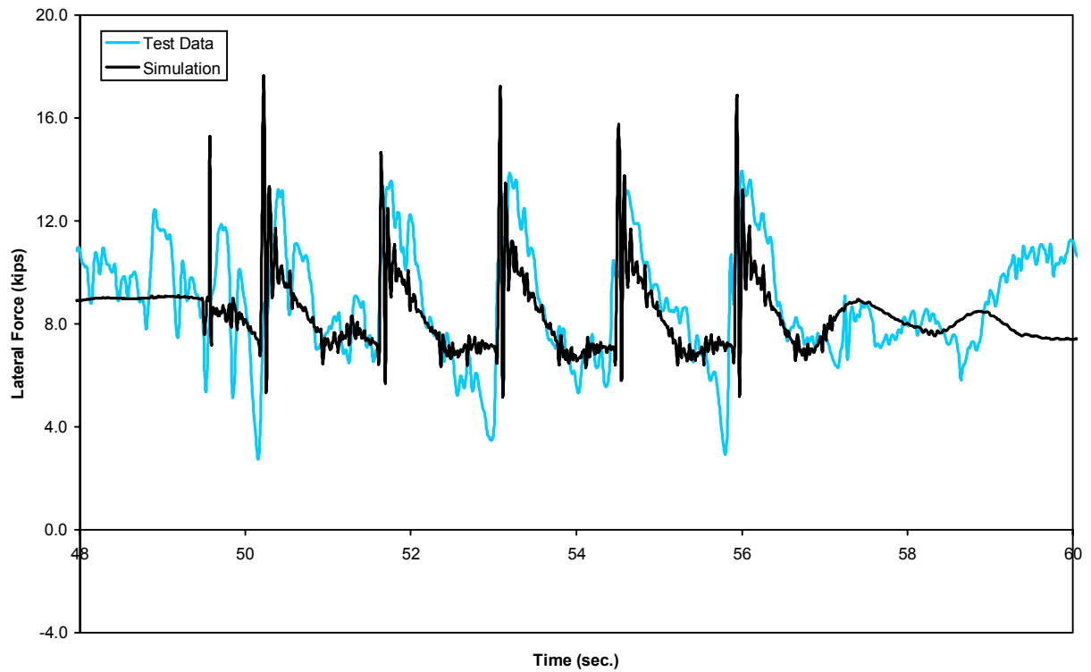
Figure B-16(a). Dynamic curving - lateral force time history, 18.6 mph (lead outer wheel)
