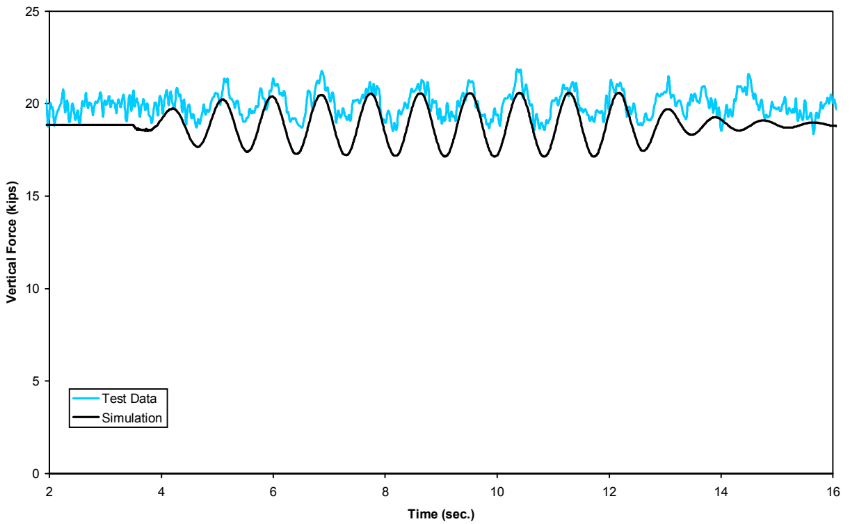
Figure B-36(a). Pitch and bounce - vertical force time history, 30 mph (lead left wheel)
