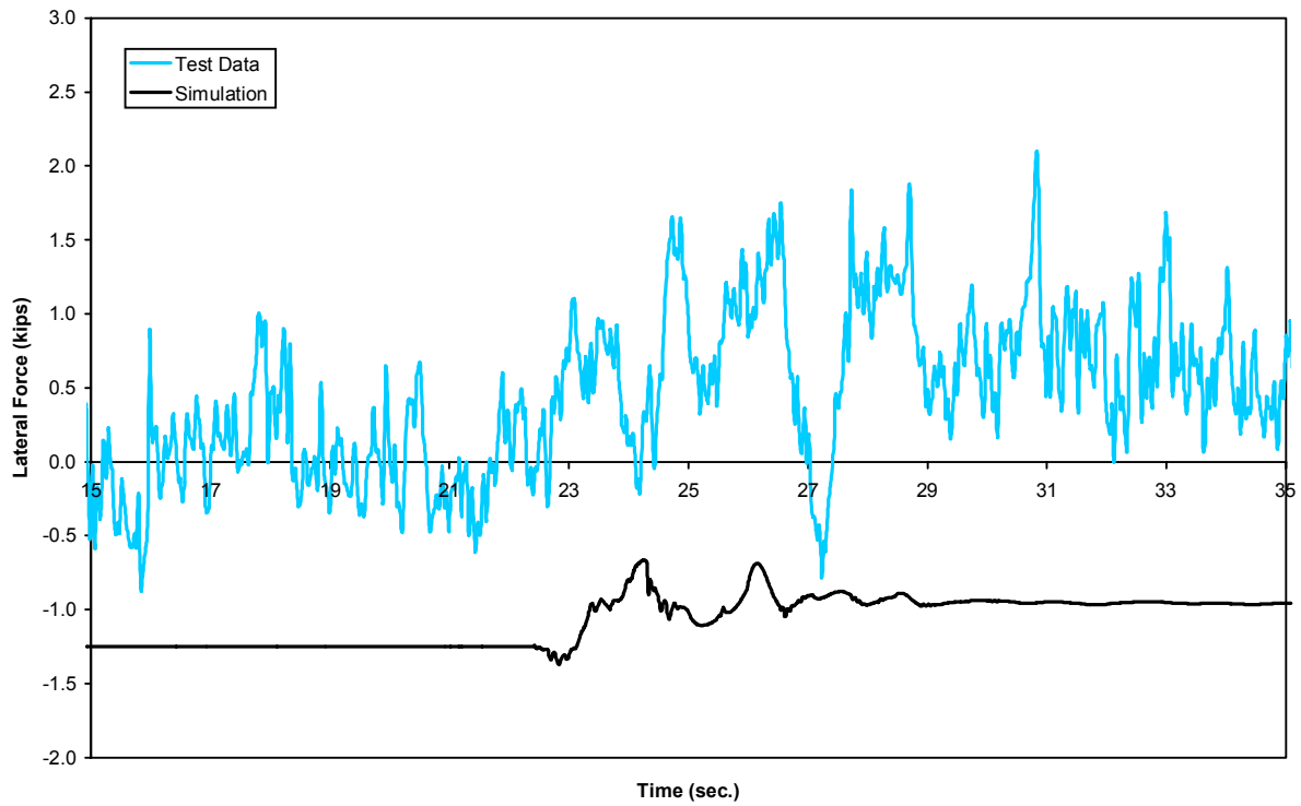
Figure B-2(c). Vertical bump test - lateral force time history, 24 mph (trailing outer wheel)
