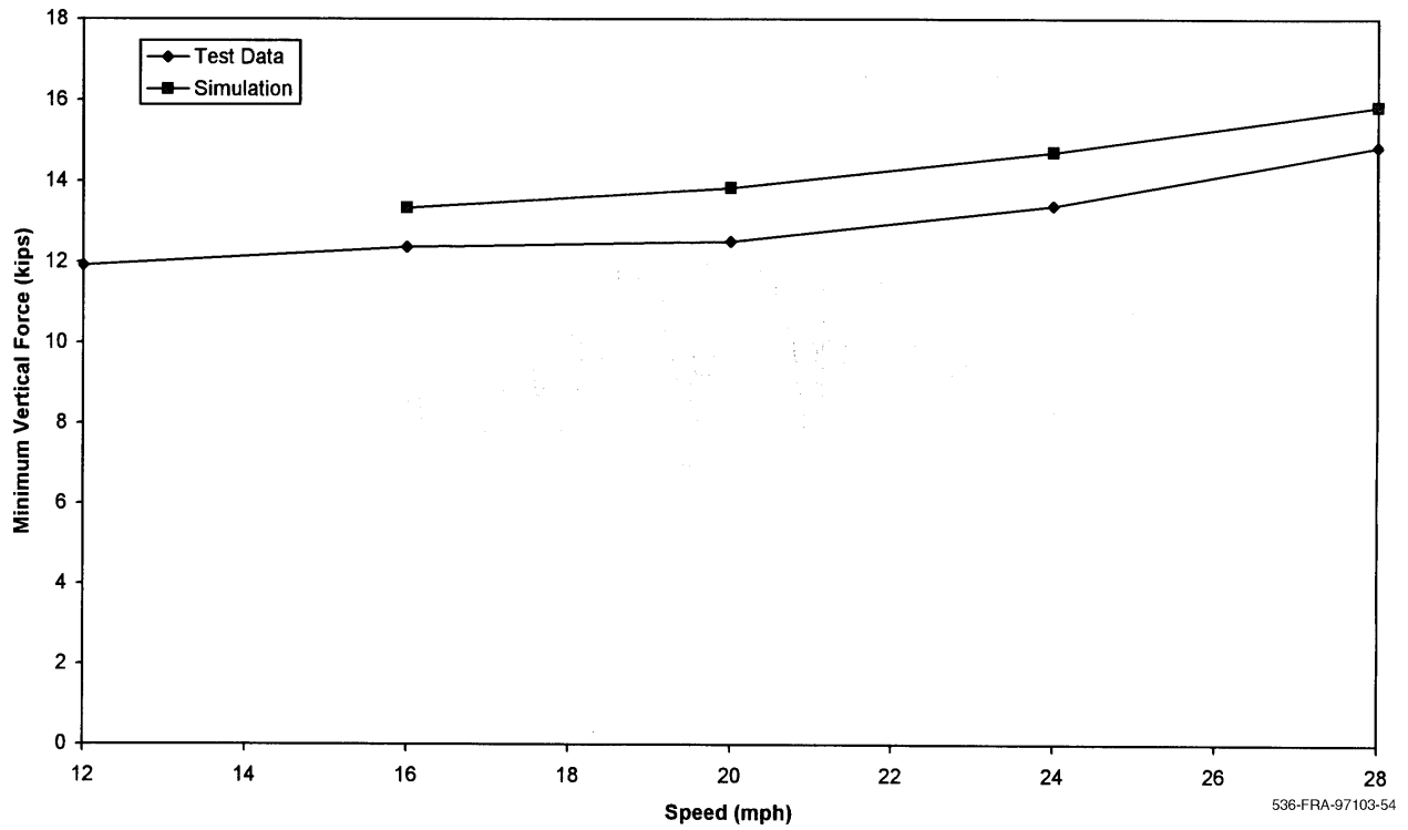
Figure A-16. Dynamic curving - minimum vertical force (lead outer wheel)
