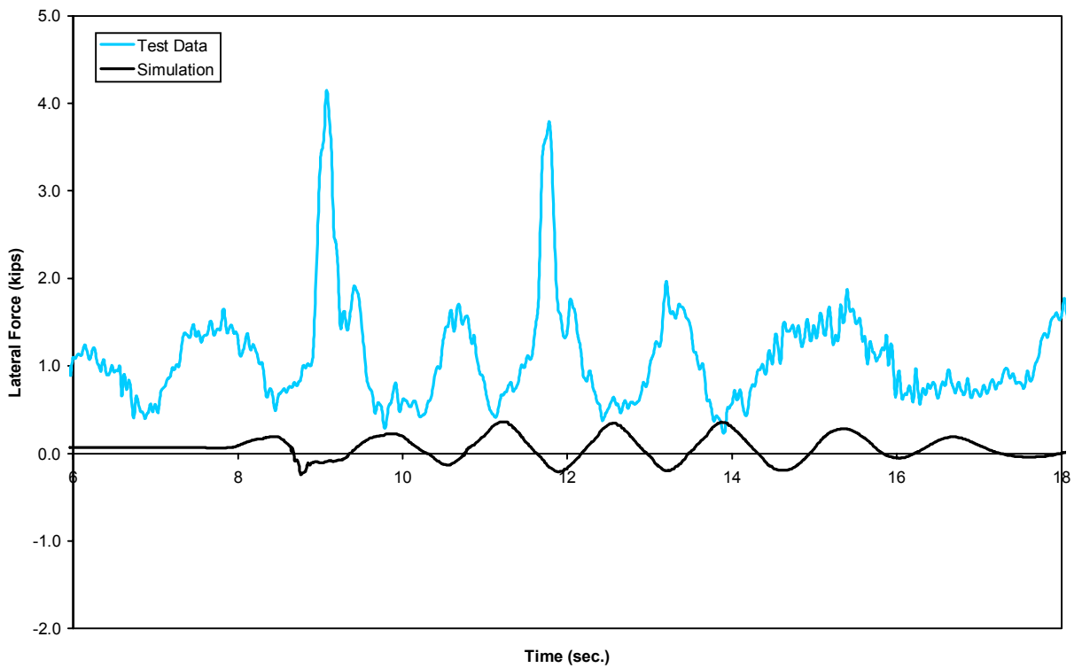
Figure B-23(a). Yaw and sway - lateral force time history, 20 mph (lead left wheel)
