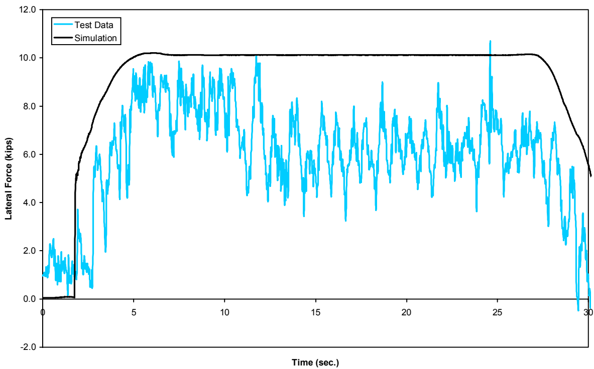
Figure B-10(a). Constant curving - lateral force time history, 32 mph (lead outer wheel)
