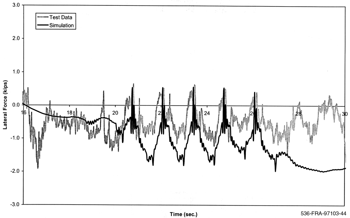
Figure A-13(c). Dynamic curving - lateral force time history, 20 mph (trailing outer wheel)
