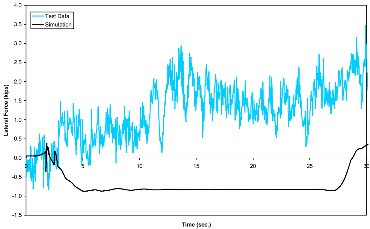
Figure B-10(c). Constant curving - lateral force time history, 32 mph (trailing outer wheel)
