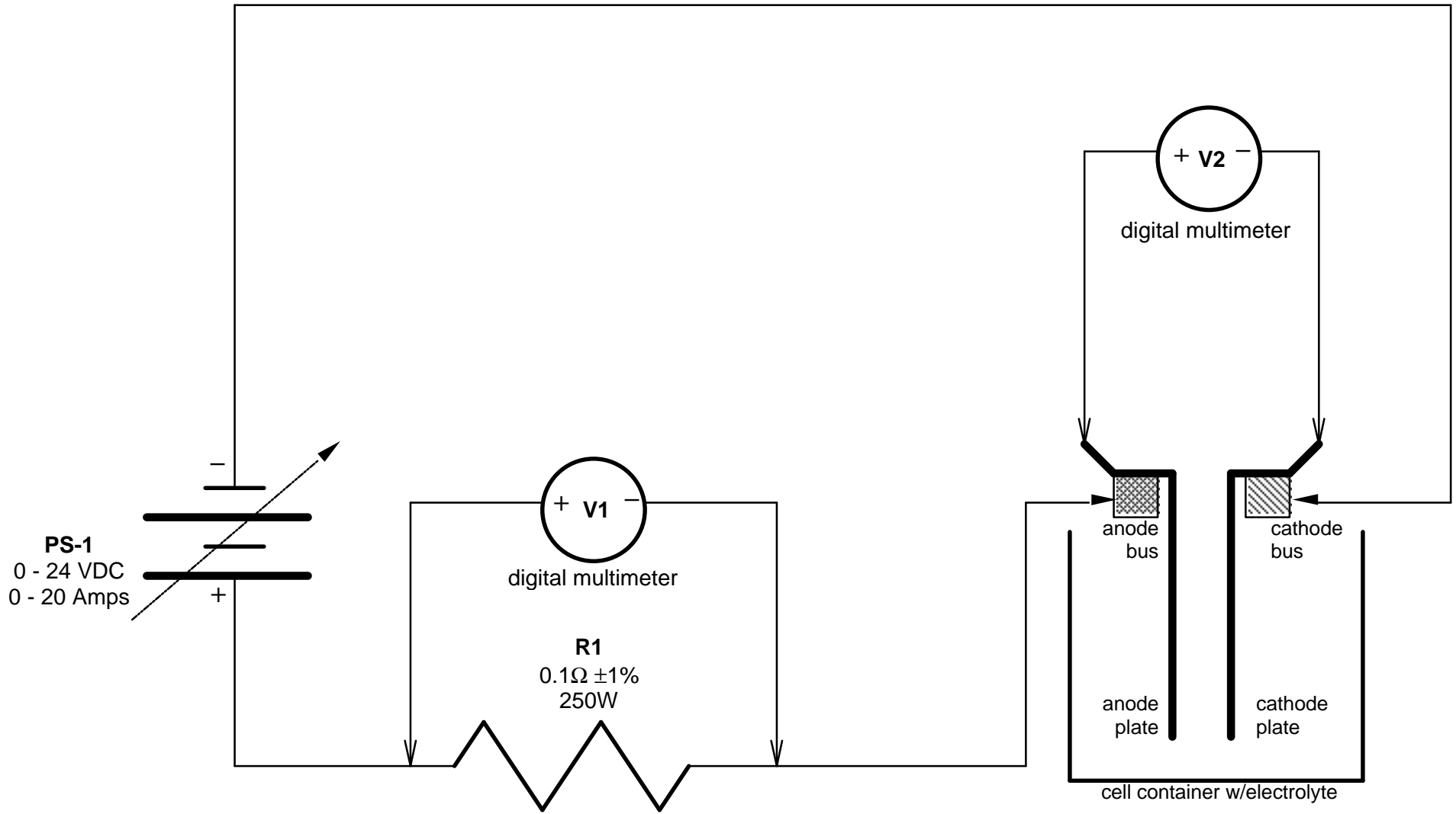
Figure-39 One-Liter Electrowinning Cell Electrical Schematic
