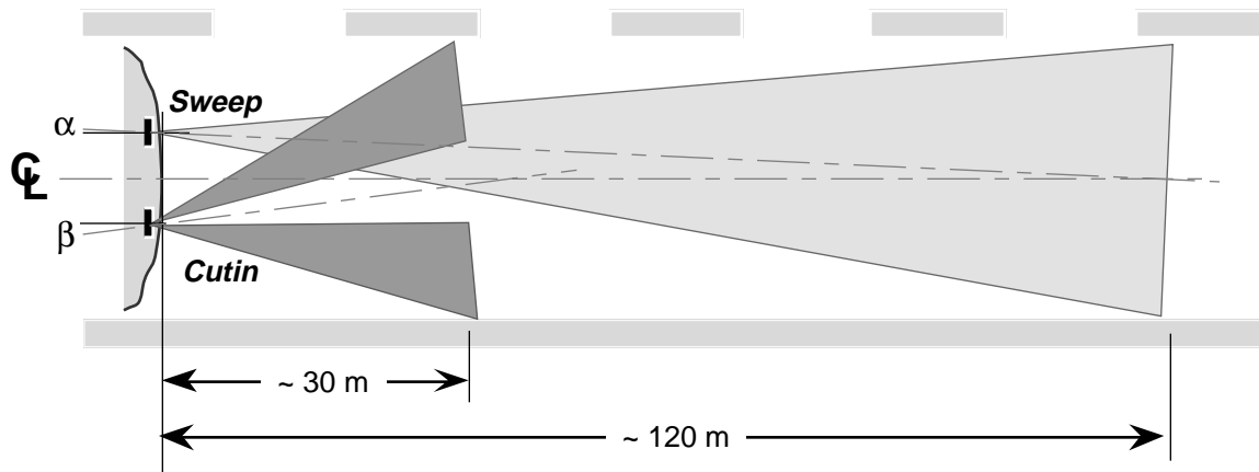
Figure 13. Top view of aligned sensor beams
