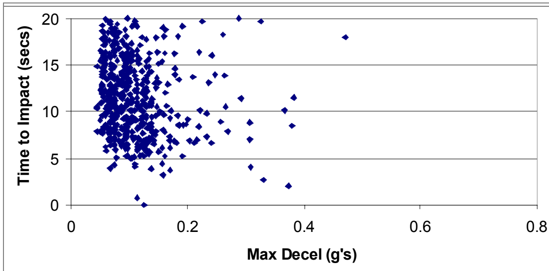
Figure 156. Time to Impact and maximum deceleration during CCC braking ( V > 55\text{mph} )
