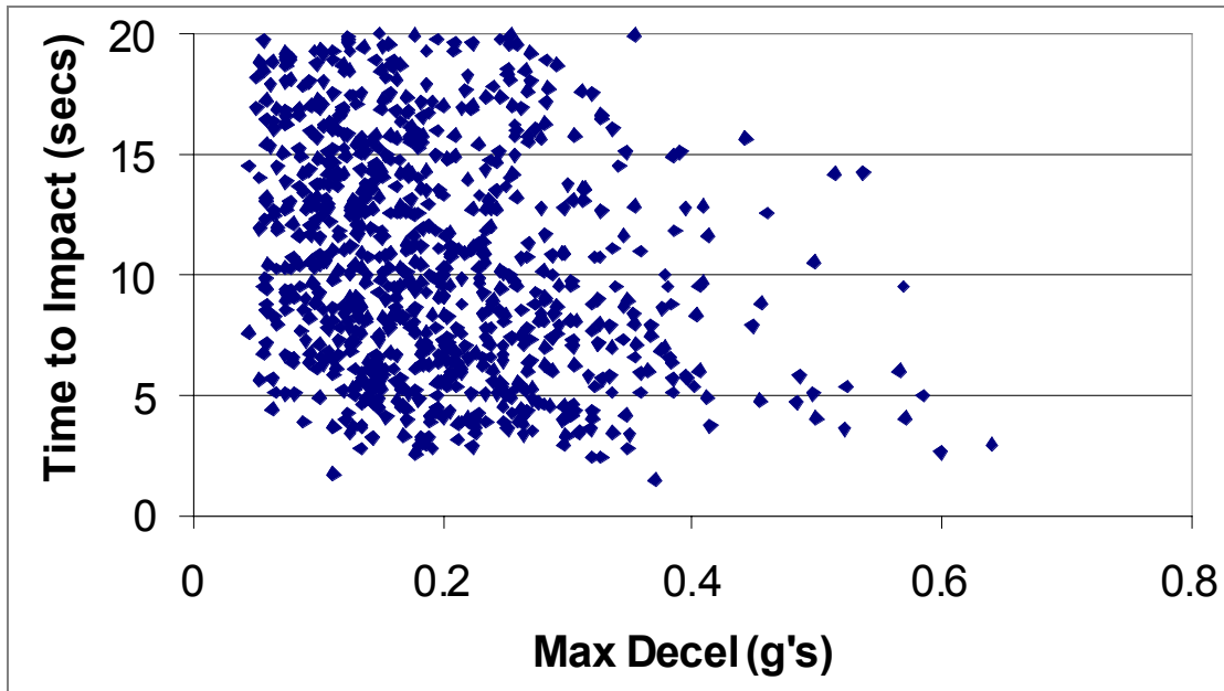
Figure 155. Time to Impact and maximum deceleration during ACC braking ( V > 55\text{mph} )
