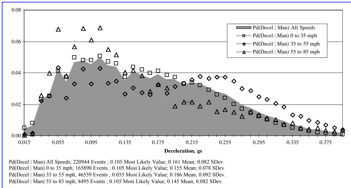
Figure 91. Maximum deceleration in manual braking events (duration > 1.0 seconds)
