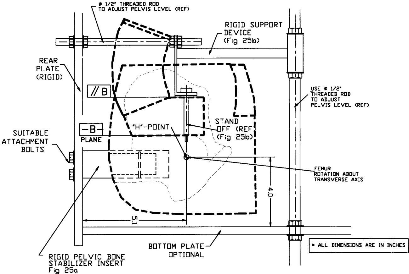
HIP-JOINT TEST FIXTURE ASSEMBLY (REF)
