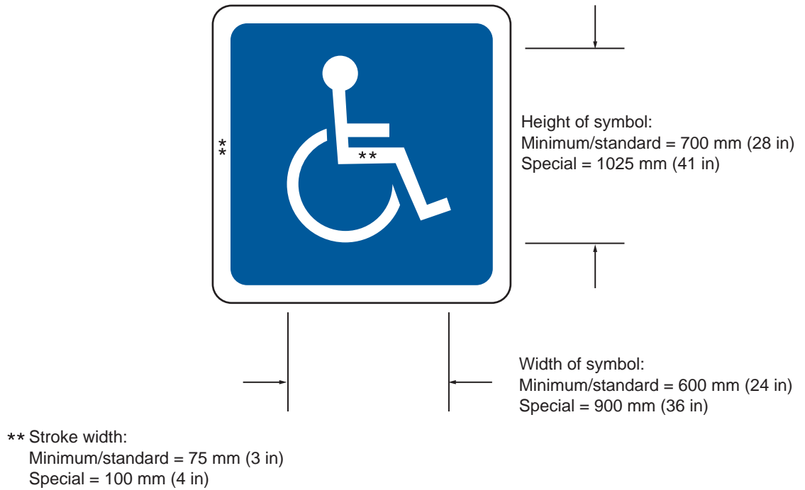
Figure 3B-18. International Symbol of Accessibility Parking Space Marking with Blue Background and White Border Options
