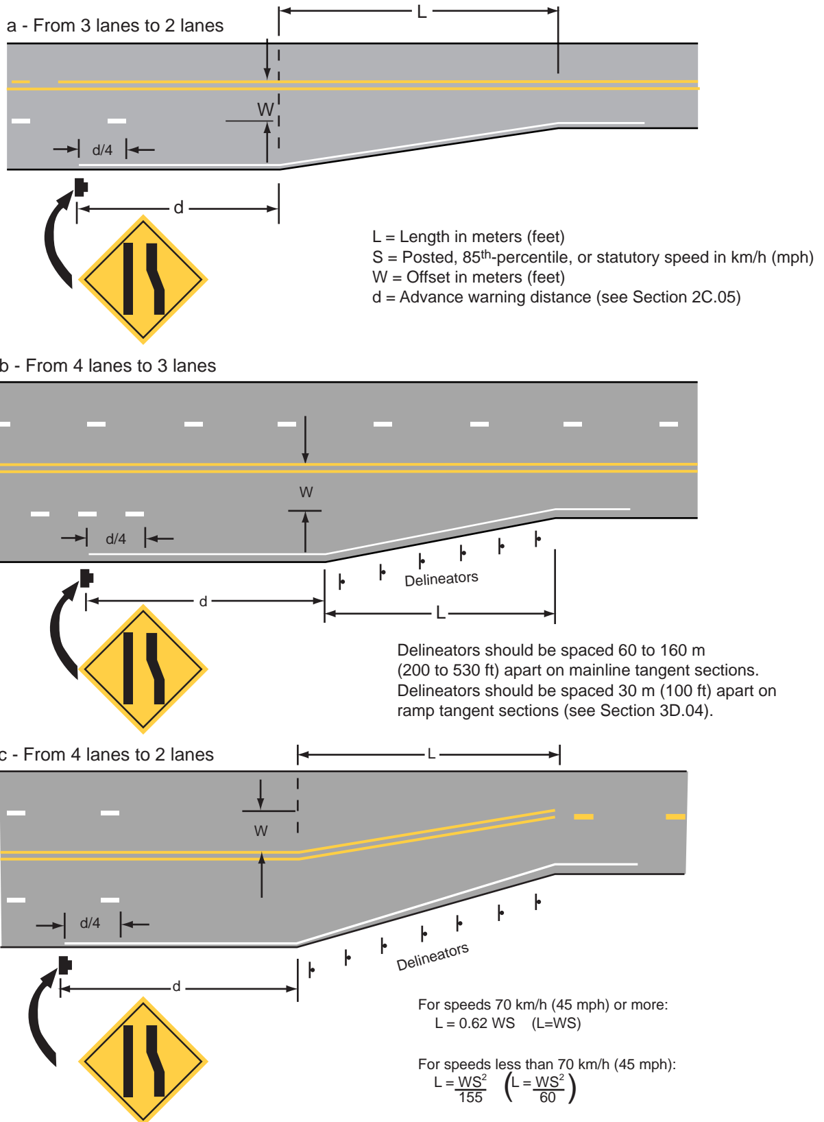
Figure 3B-12. Typical Lane Reduction Transition Markings
