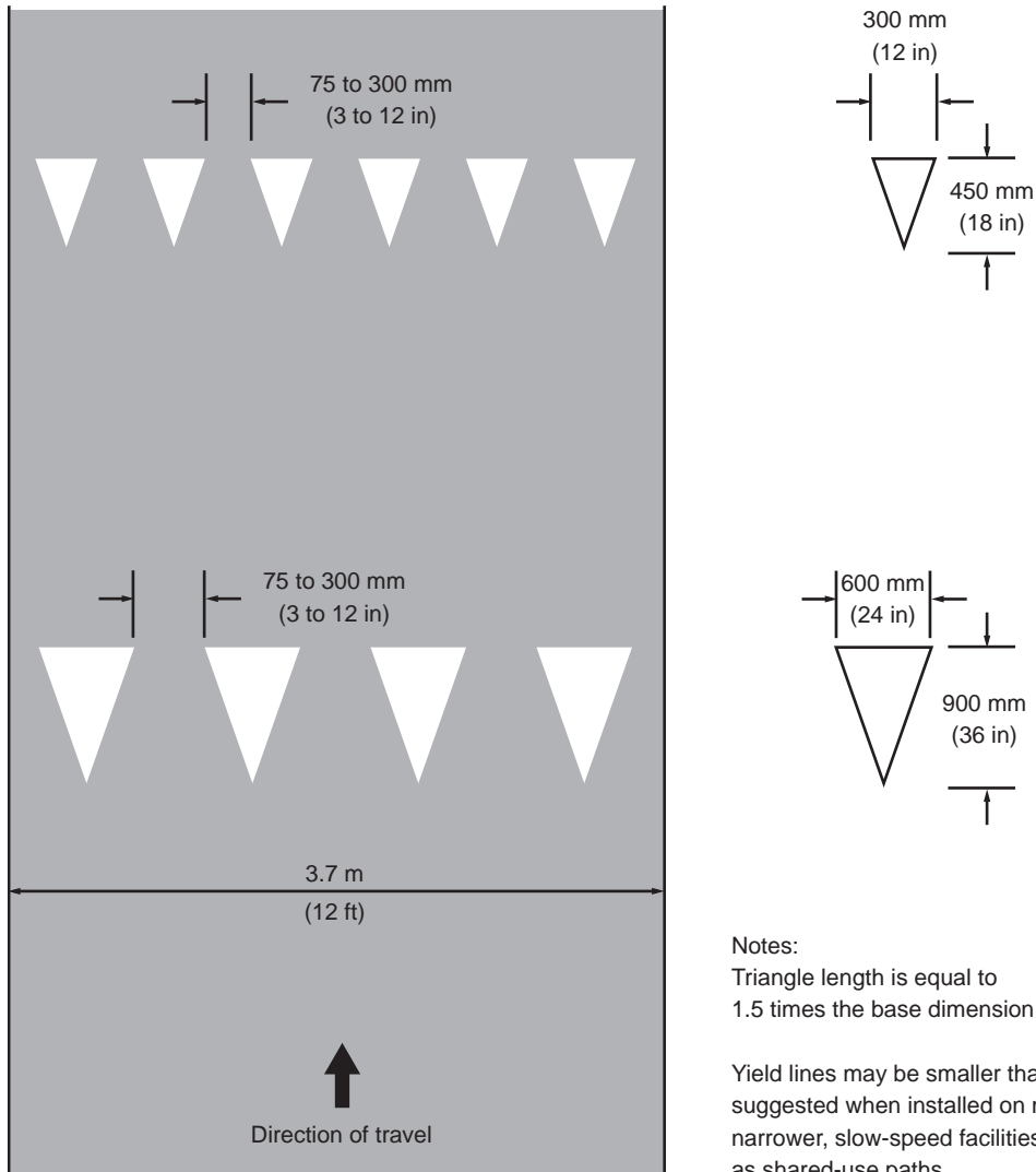
Figure 3B-14. Typical Yield Line Layout for Streets and Highways
