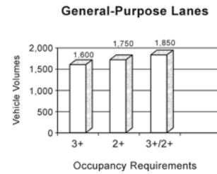
Figure 6. Changes in Morning Peak Hour Vehicle Volumes (2)
