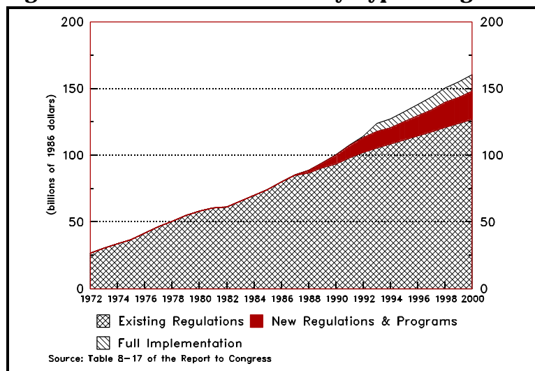
Fig. 2-1: Total Annualized Costs by Type of Regulation
