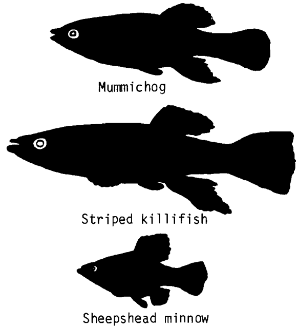
Figure 3. Silhouettes of the three most common killifishes on the Mid-Atlantic coast of the United States (from Rosen 1973).
