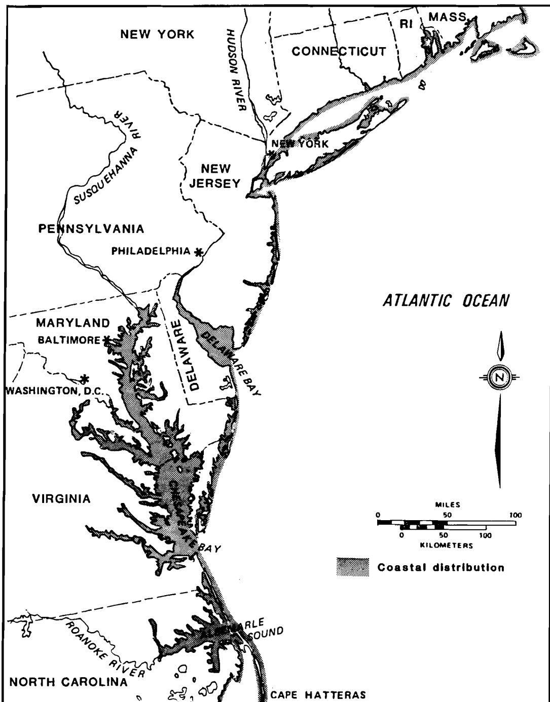
Figure 2. Mid-Atlantic coast distribution of mummichog and striped killifish. Both are found the entire length of the Mid-Atlantic region close to shore (within 110 m for mummichogs: Armstrong and Child 1965) and in bays, estuaries and tidal creeks (Hardy 1978). Striped killifish penetrate tidal rivers only as far as the mean boundary between fresh and brackish water; mummichogs penetrate as far as 75 km beyond this boundary (Massman 1954).
