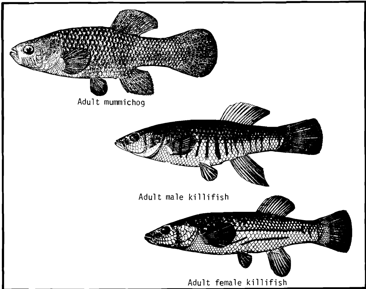
Figure 1. Mummichog and striped killifish.
