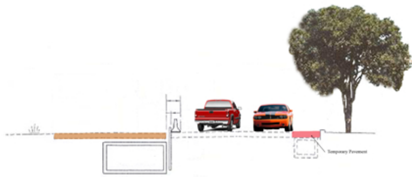
Centerline Road @ Long Bay Road - Phase I Roadway Reconstruction Typical (View North)
