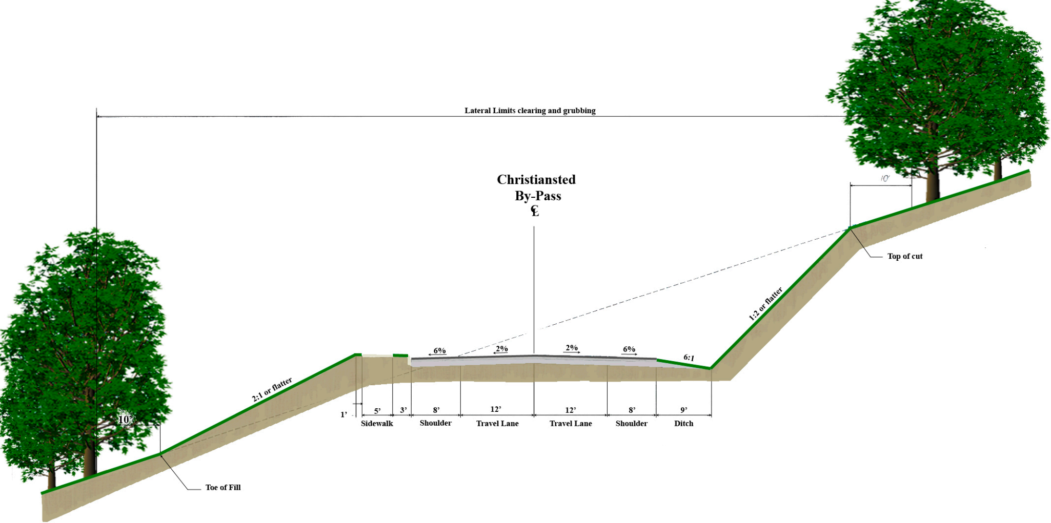
TYPICAL SECTION - 2 LANES CHRISTIANSTED BY - PASS Christiansted, St. Croix, U.S. Virgin Island August, 2006
