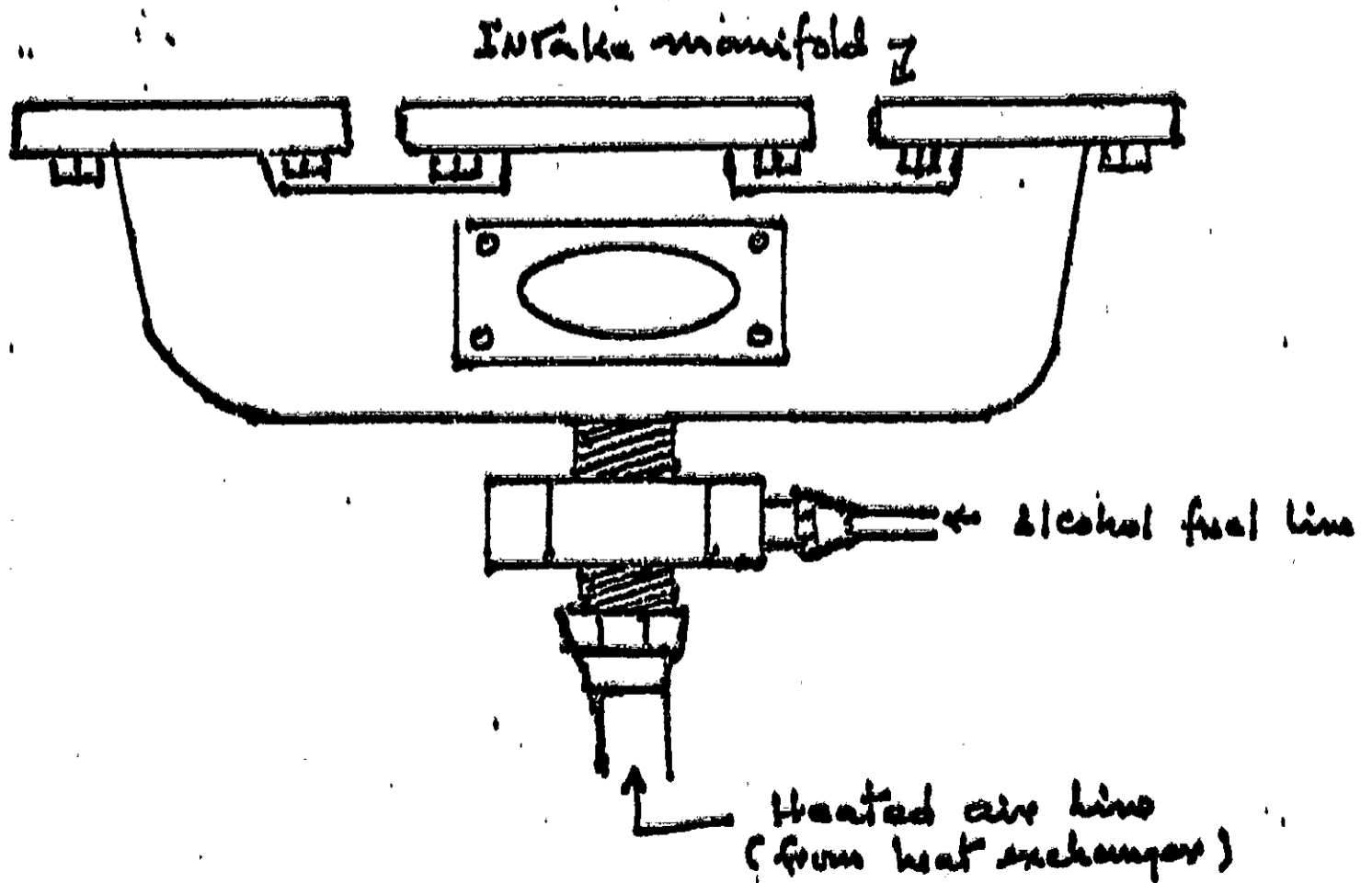
Figure 4 Vaporization Chamber
