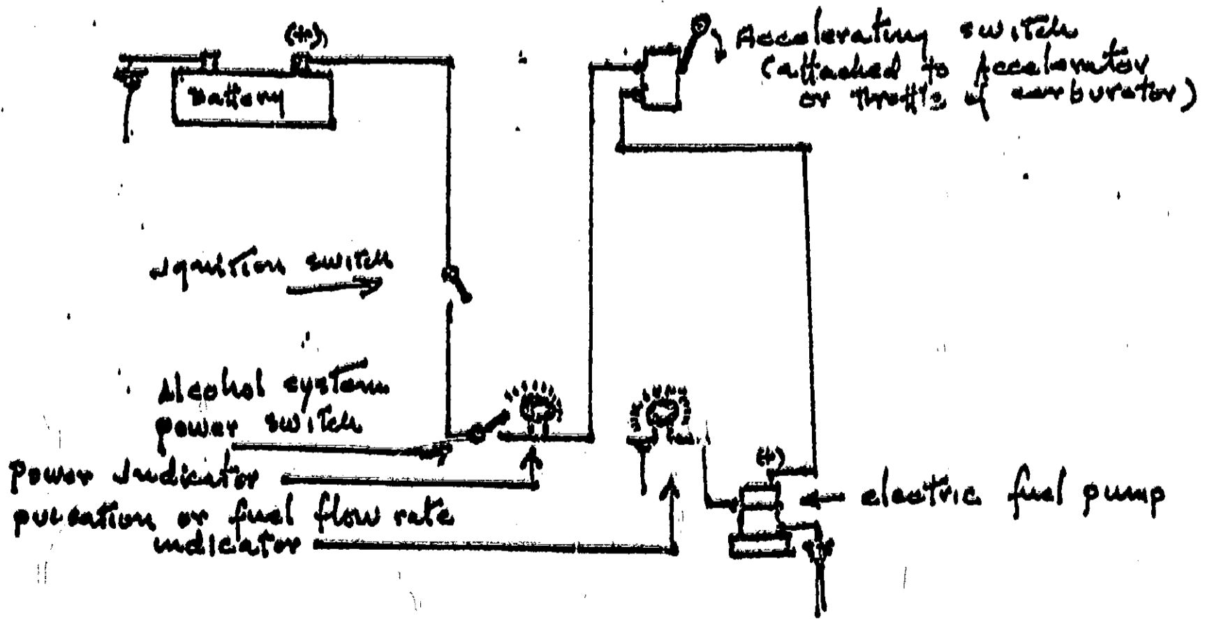
Figure 6 Wiring Diagram for Dynamix
