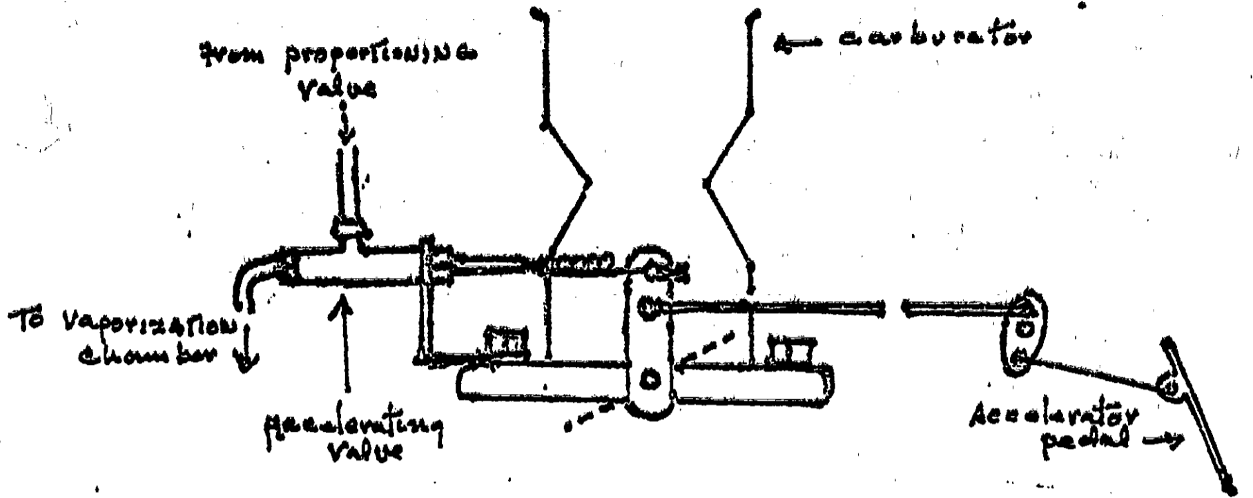
Figure 3 Accelerator Valve and Linkage
