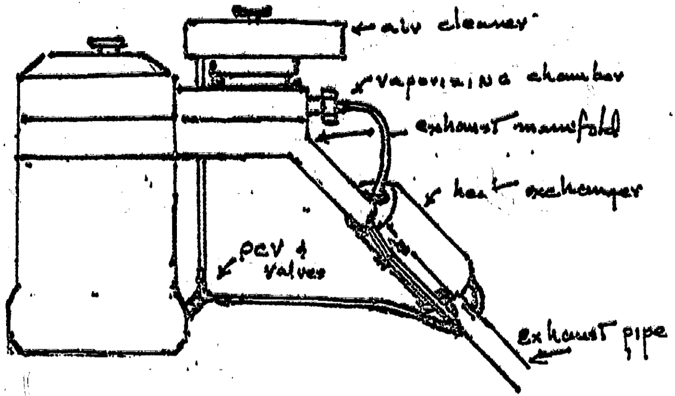
Figure 5 Heat Exchanger and Heated Air System
