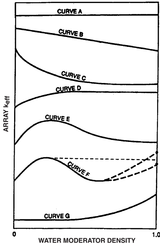
FIG. VII.1. Typical plots of array k_{eff} versus interspersed water moderator density.
