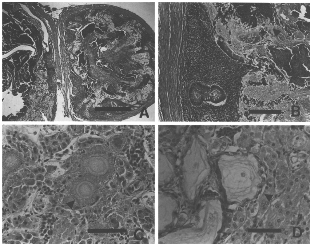
Fig. 1. (A) Small intestine and attached ceca—note diffuse necrosis of superficial mucosa on left. Bar = 1000 \mu m. (B) Lamina propria of small intestine—note diffuse lymphoplasmacytic infiltrate on left and necrosis of superficial mucosa on right. Bar = 200 \mu m. (C) Kidney—note stellate urate crystals within necrotic proximal tubules. Bar = 70 \mu m. (D) Kidney—note distal tubules distended with mucus concretions surrounded by flattened tubule cells. Bar = 50 \mu m.
