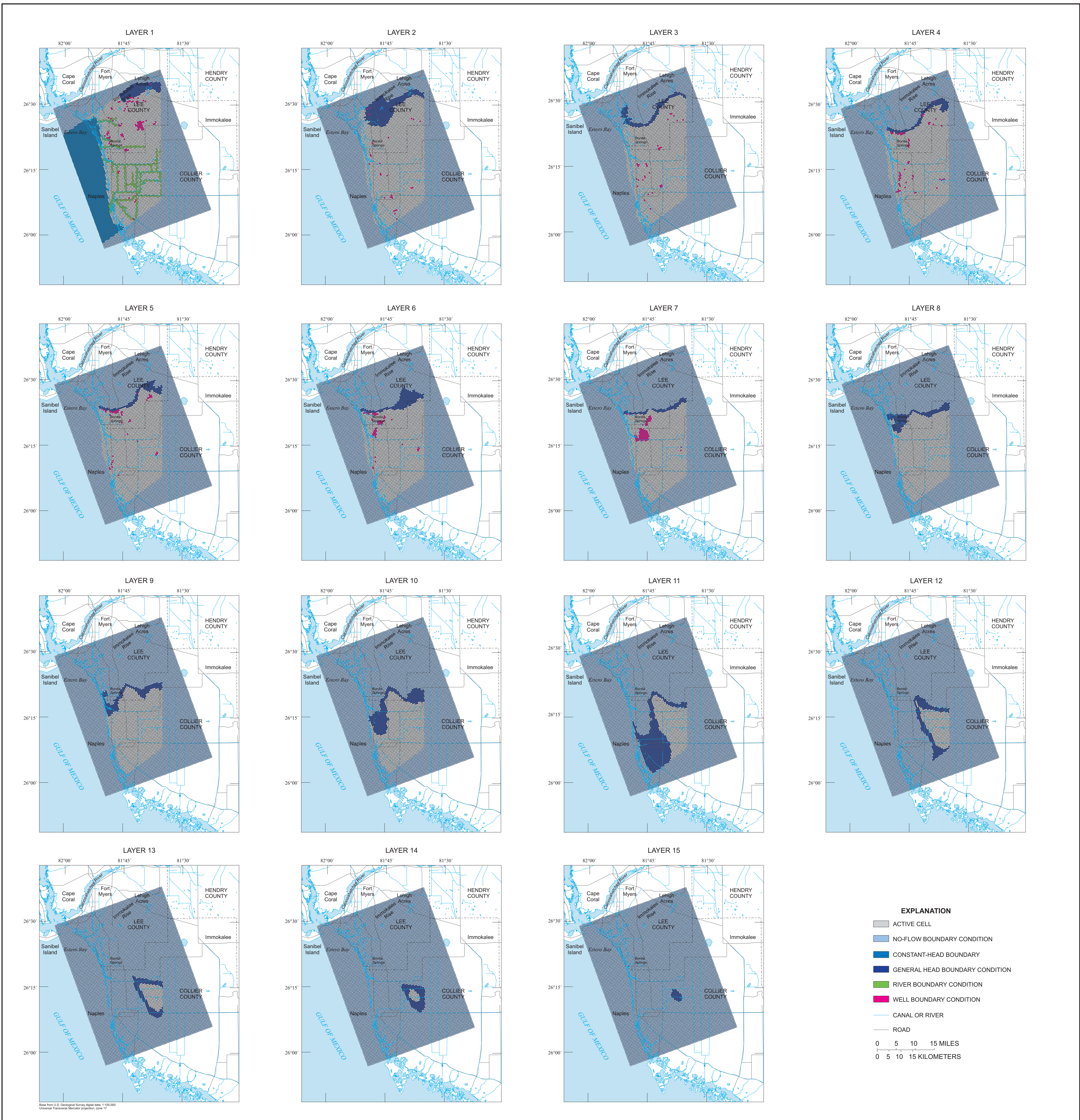
PLATE 2. BOUNDARY CONDITIONS FOR CALIBRATING THE MODEL TO MARCH AND SEPTEMBER 1996 CONDITIONS AND MOVING THE PREDEVELOPMENT DISTRIBUTION OF SALTWATER TO EQUILIBRIUM
