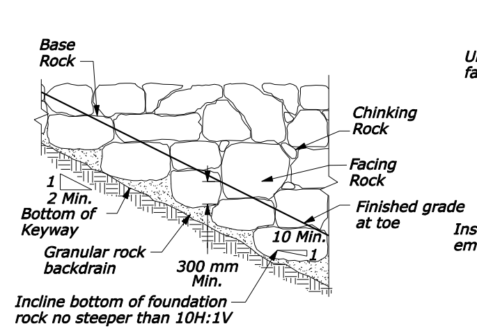
CORRECT PARTIAL TYPICAL PROFILE
