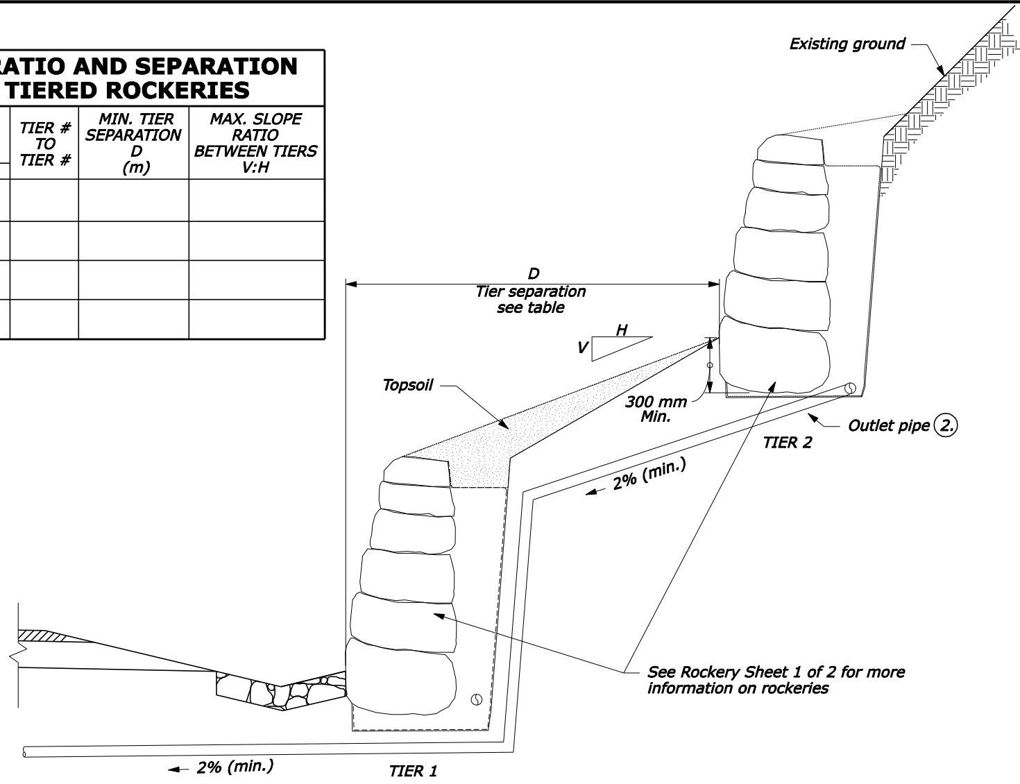
ROCKERY WITH TIERS TYPICAL SECTION
