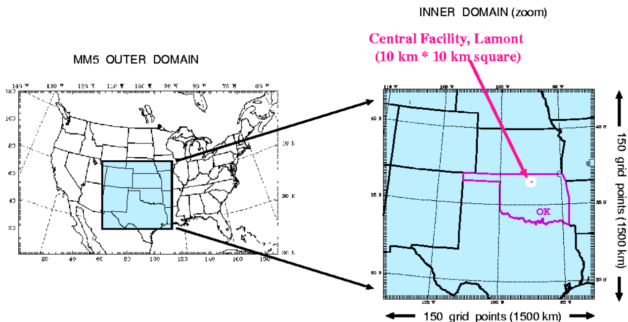
Figure 1. Domain simulated with MM5. The grid point corresponding to the central facility site is indicated by a red square (surrounded by a white disk).
