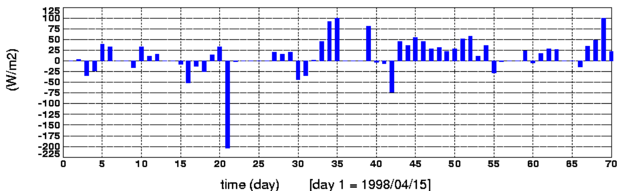
Figure 4. The daily (24-hr) mean difference between simulated and measured SW downward flux at the surface.
