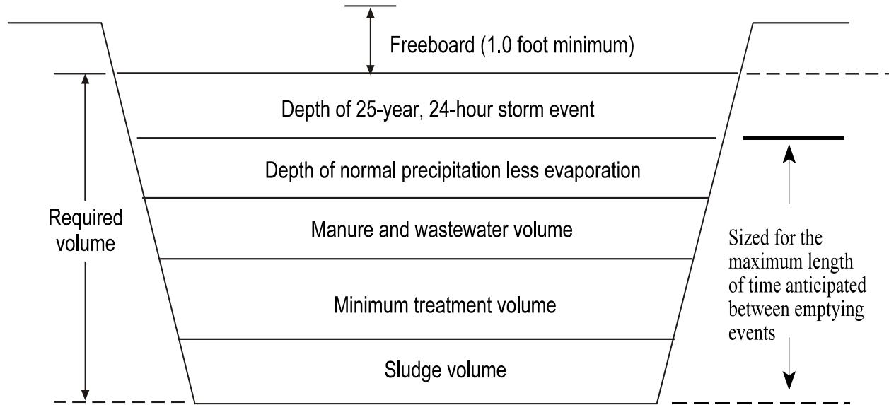
Figure 2-2. Cross Section of Properly Designed Lagoon
