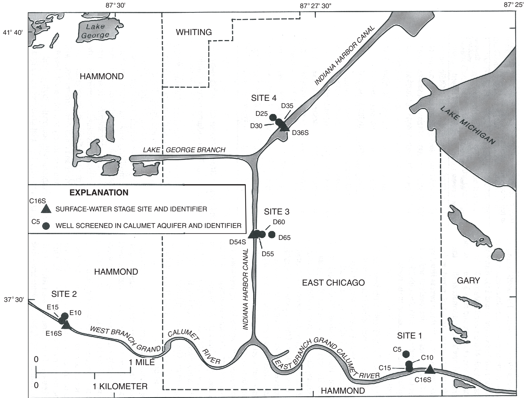
Figure 9. Locations of four transects of observation wells adjacent to the Indiana Harbor Canal and the Grand Calumet River, northwestern Indiana
