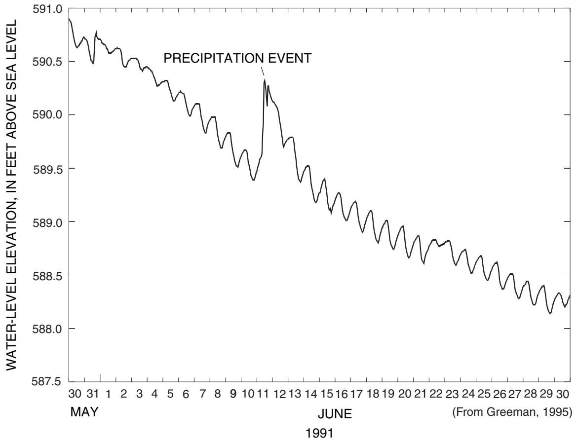
Figure 8. Ground-water hydrograph showing the daily effects of evapotranspiration, well LK-13 at Hammond, Indiana, 1991 data.
