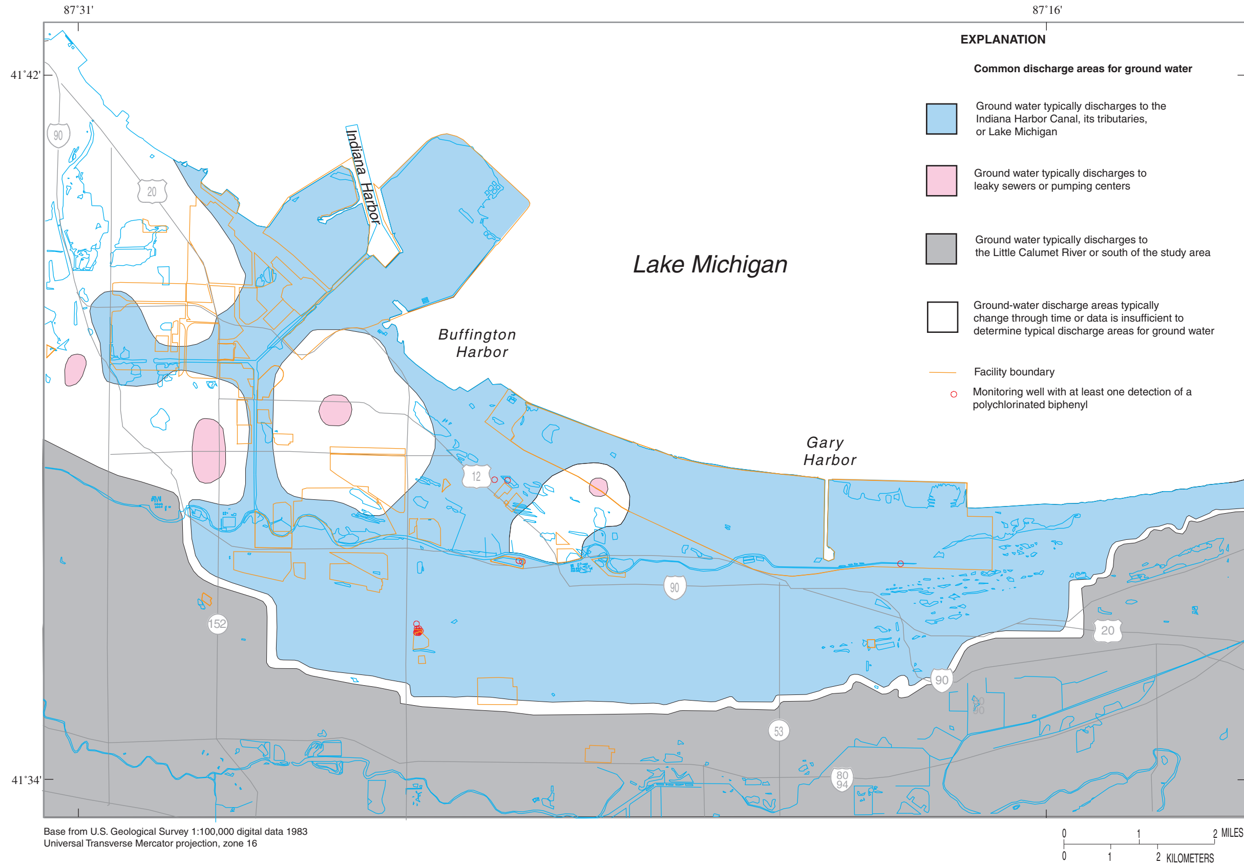
Figure 35. Common discharge areas for ground water in the Calumet aquifer and monitoring wells with at least one detection of a polychlorinated biphenyl in the study area, northwestern Indiana.
