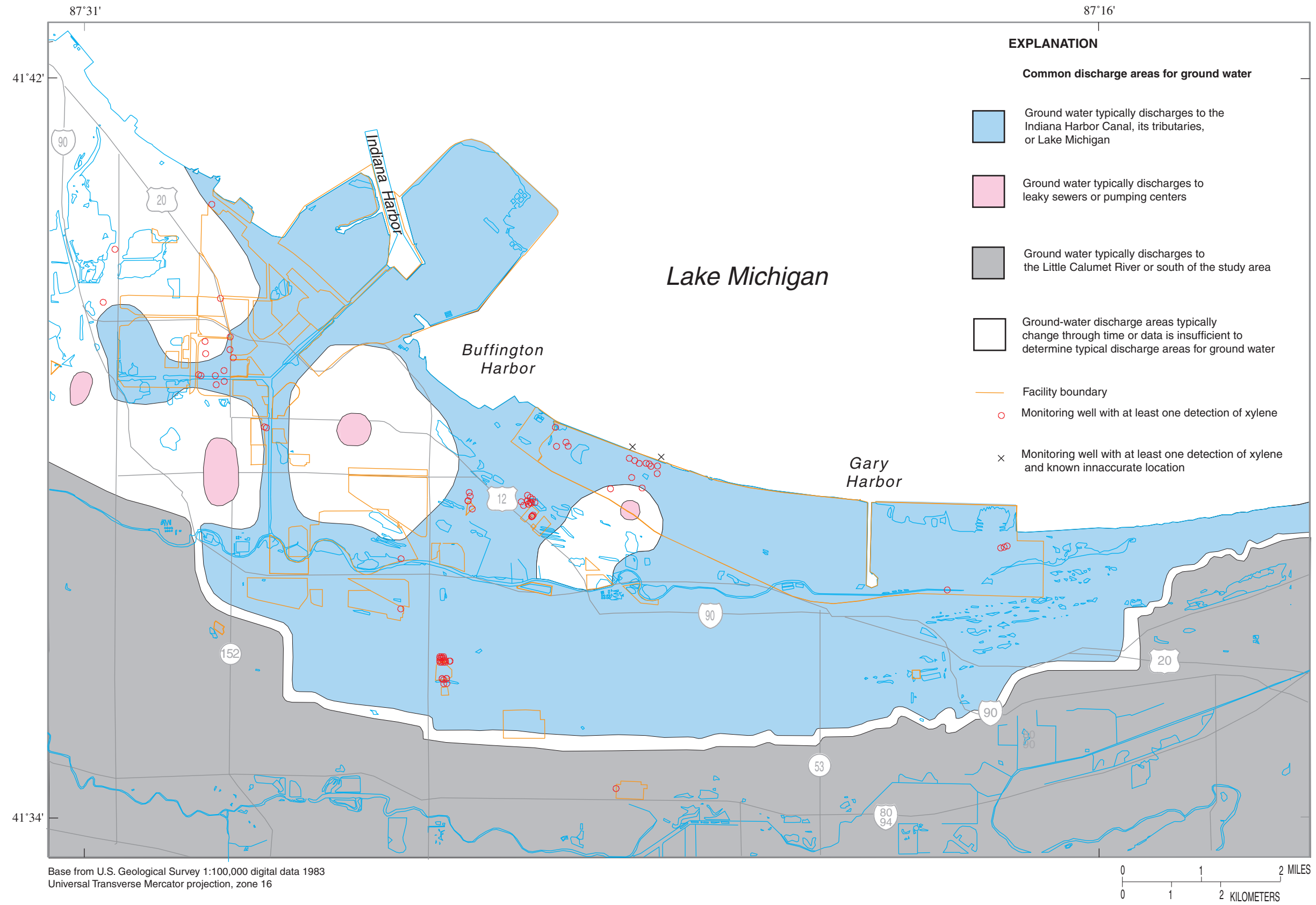
Figure 31. Common discharge areas for ground water in the Calumet aquifer and monitoring wells with at least one detection of xylene in the study area, northwestern Indiana.
