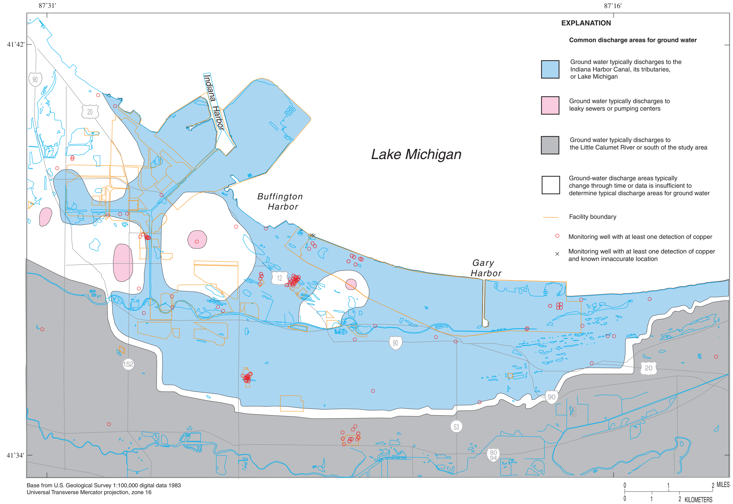
Figure 26. Common discharge areas for ground water in the Calumet aquifer and monitoring wells with at least one detection of copper in the study area, northwestern Indiana.
