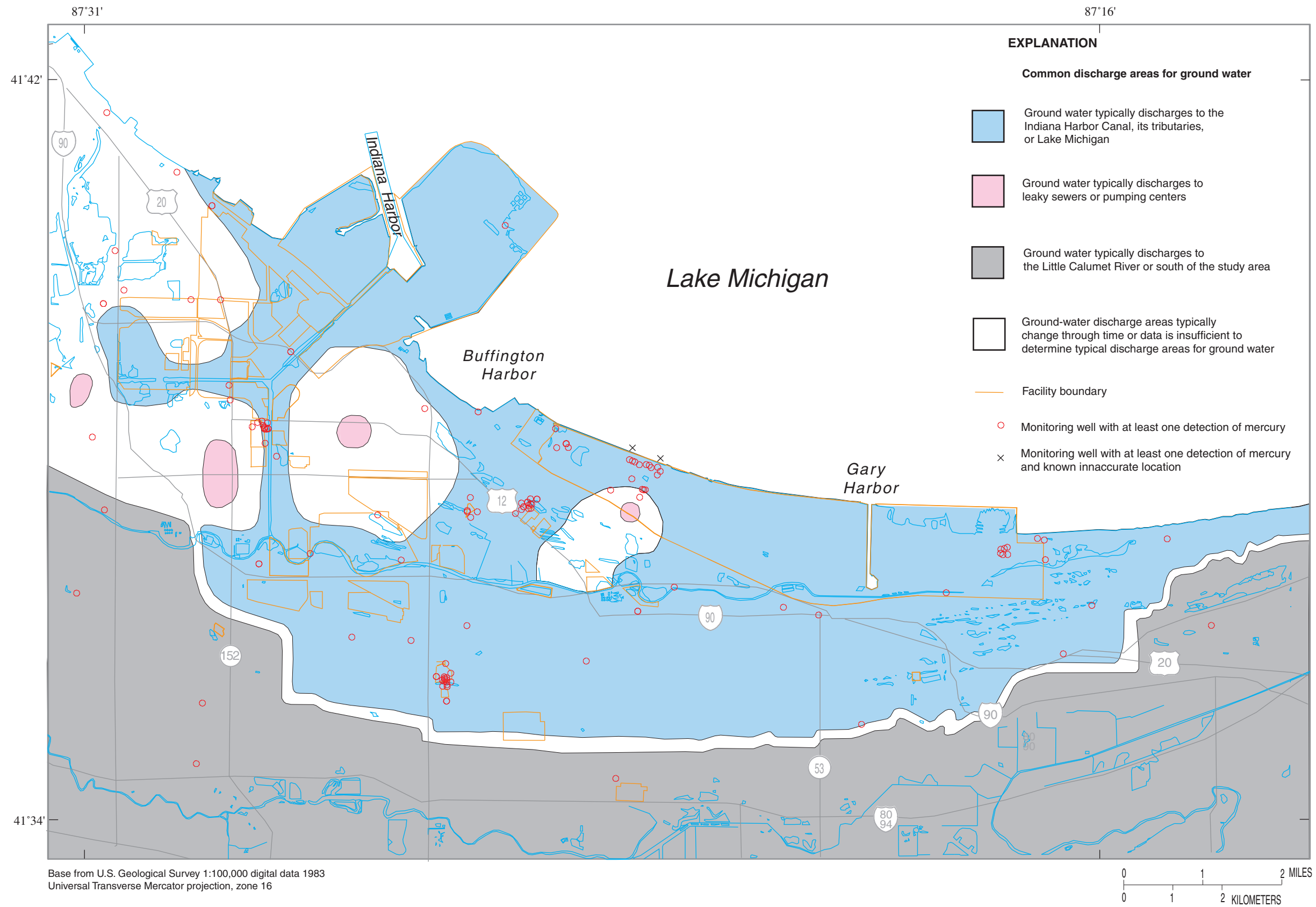
Figure 25. Common discharge areas for ground water in the Calumet aquifer and monitoring wells with at least one detection of mercury in the study area, northwestern Indiana.
