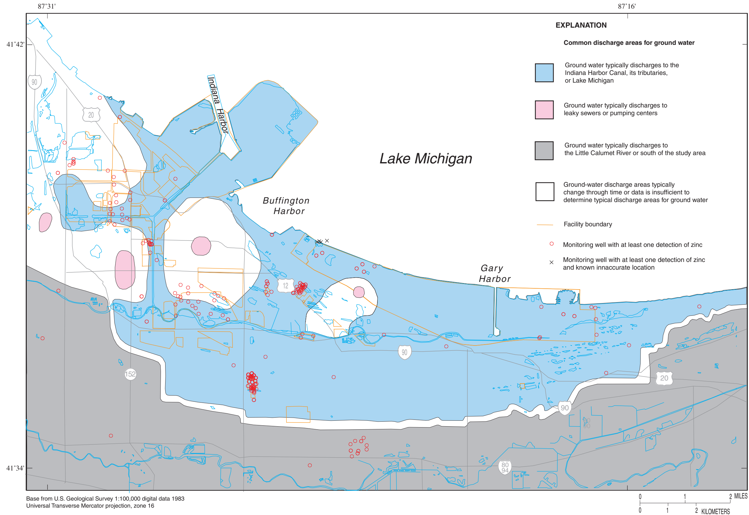
Figure 22. Common discharge areas for ground water in the Calumet aquifer and monitoring wells with at least one detection of zinc in the study area, northwestern Indiana.
