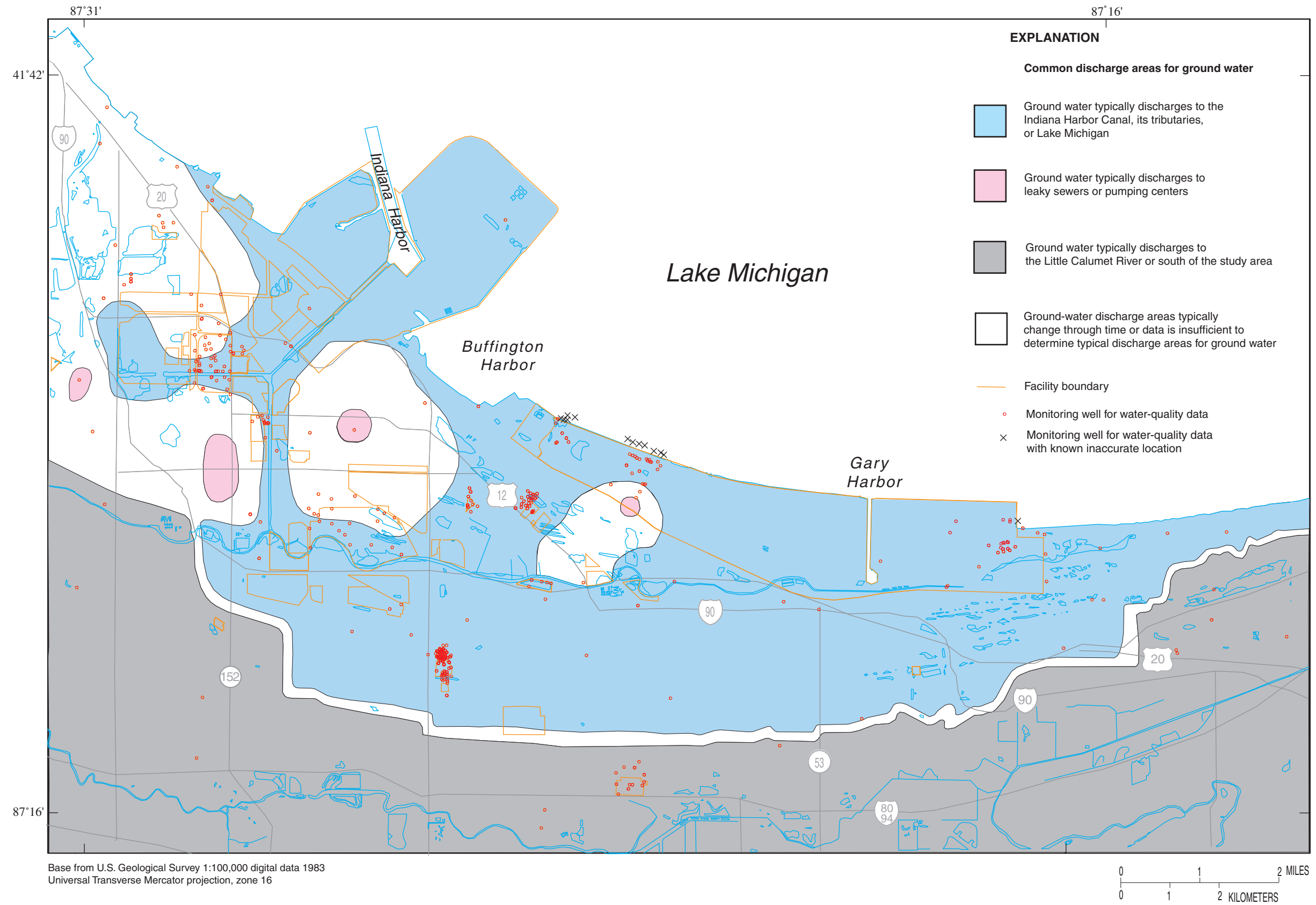
Figure 16. Common discharge areas for ground water in the Calumet aquifer underlying the study area, northwestern Indiana.
