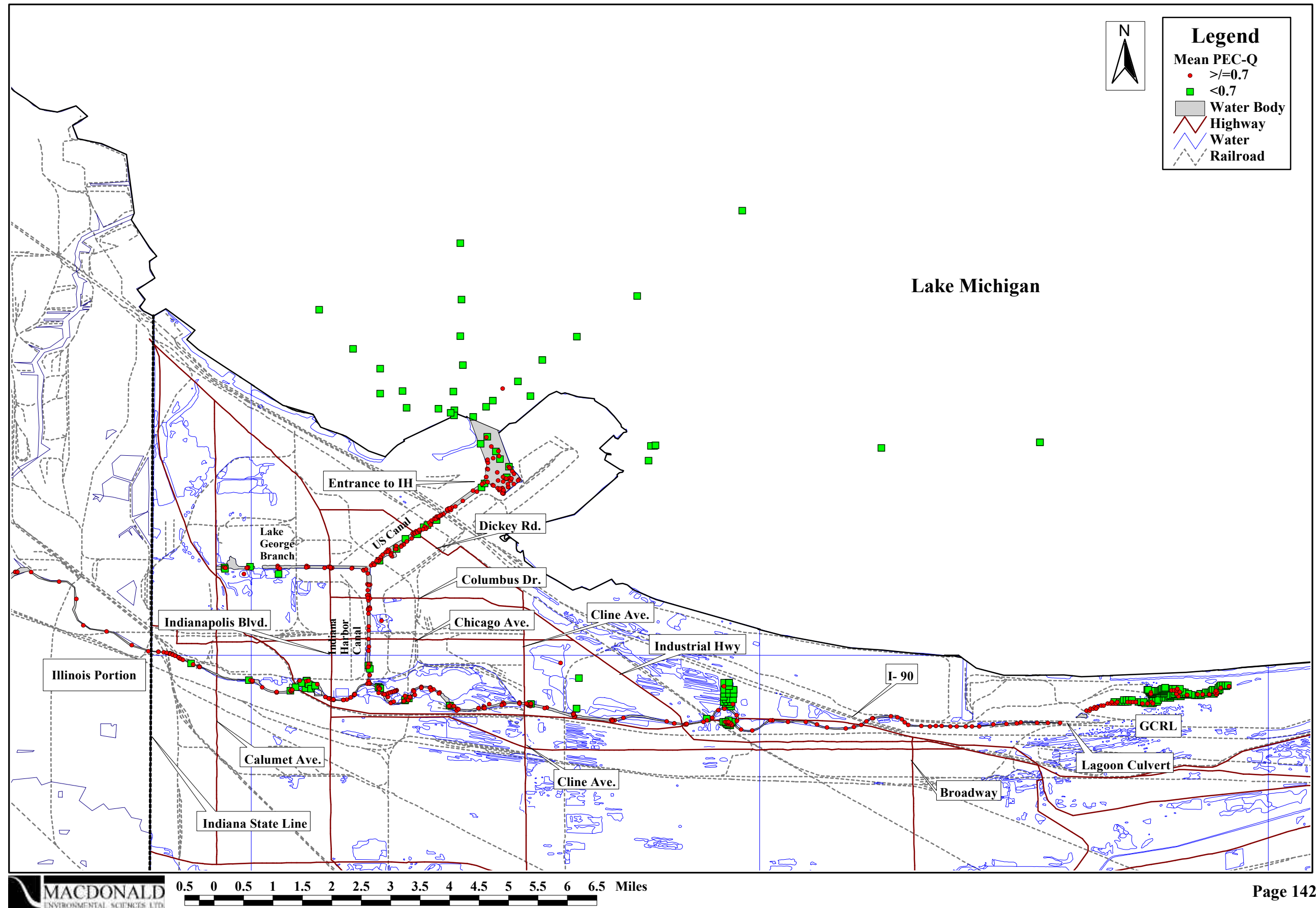
Figure 14.1. Areal extent of injury to surficial sediments in the Assessment Area.
