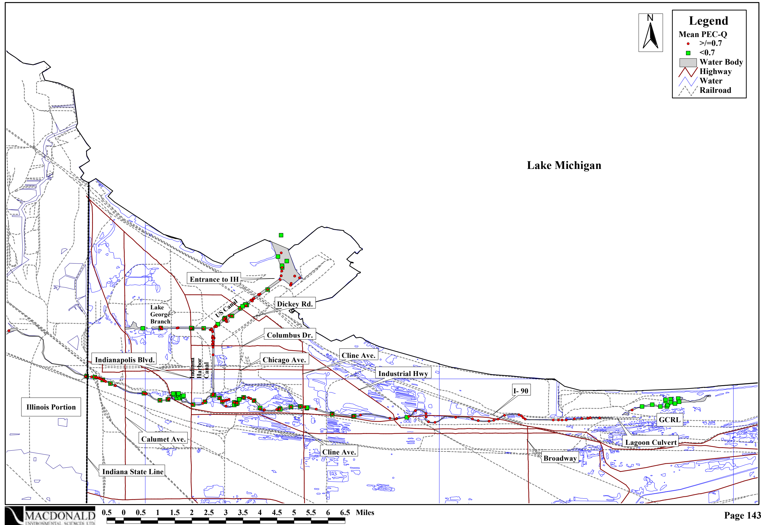
Figure 14.2. Areal extent of injury to sub-surface sediments in the Assessment Area.
