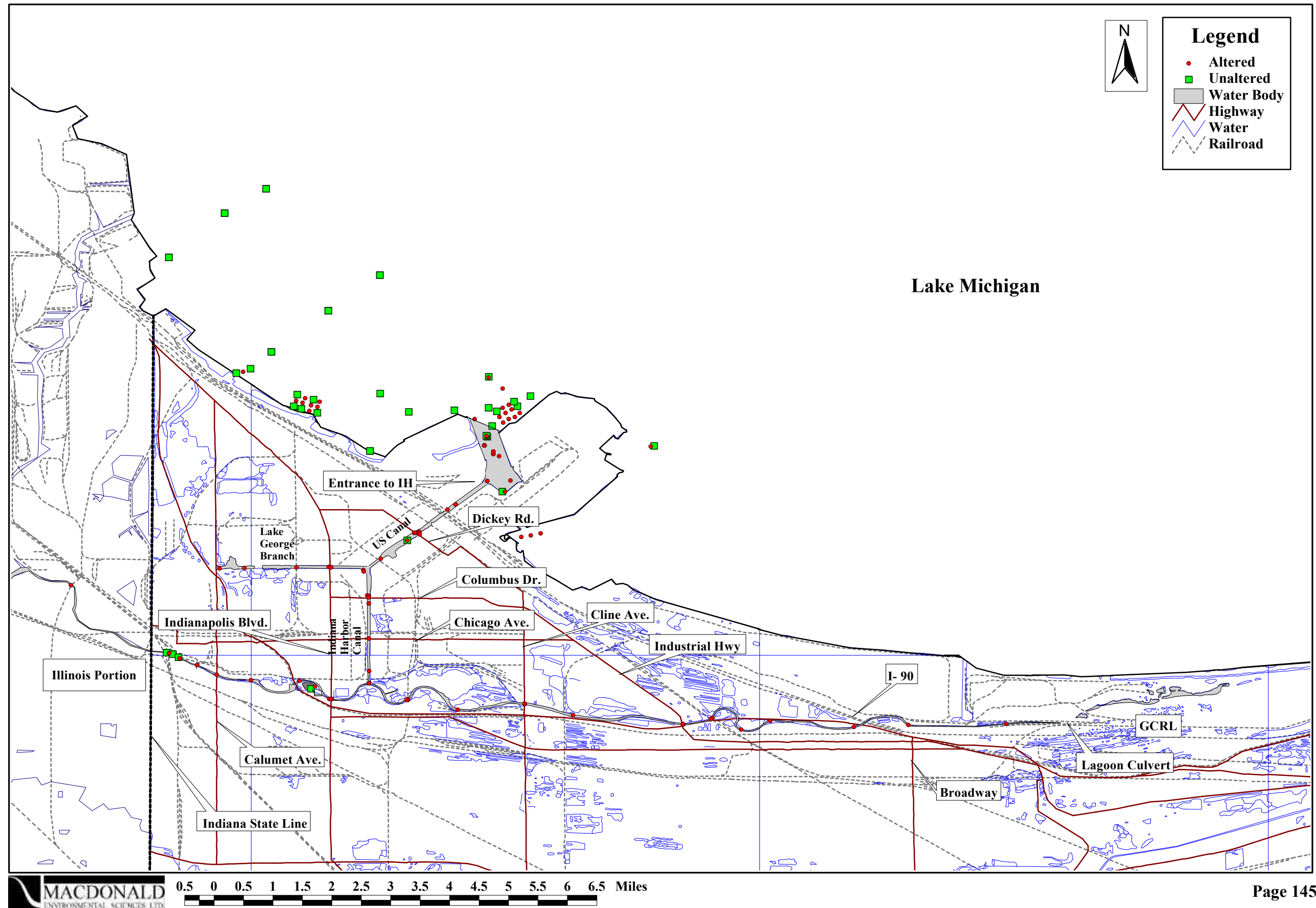
Figure 14.4. Areal extent of altered and unaltered benthic invertebrate communities in the Assessment Area.
