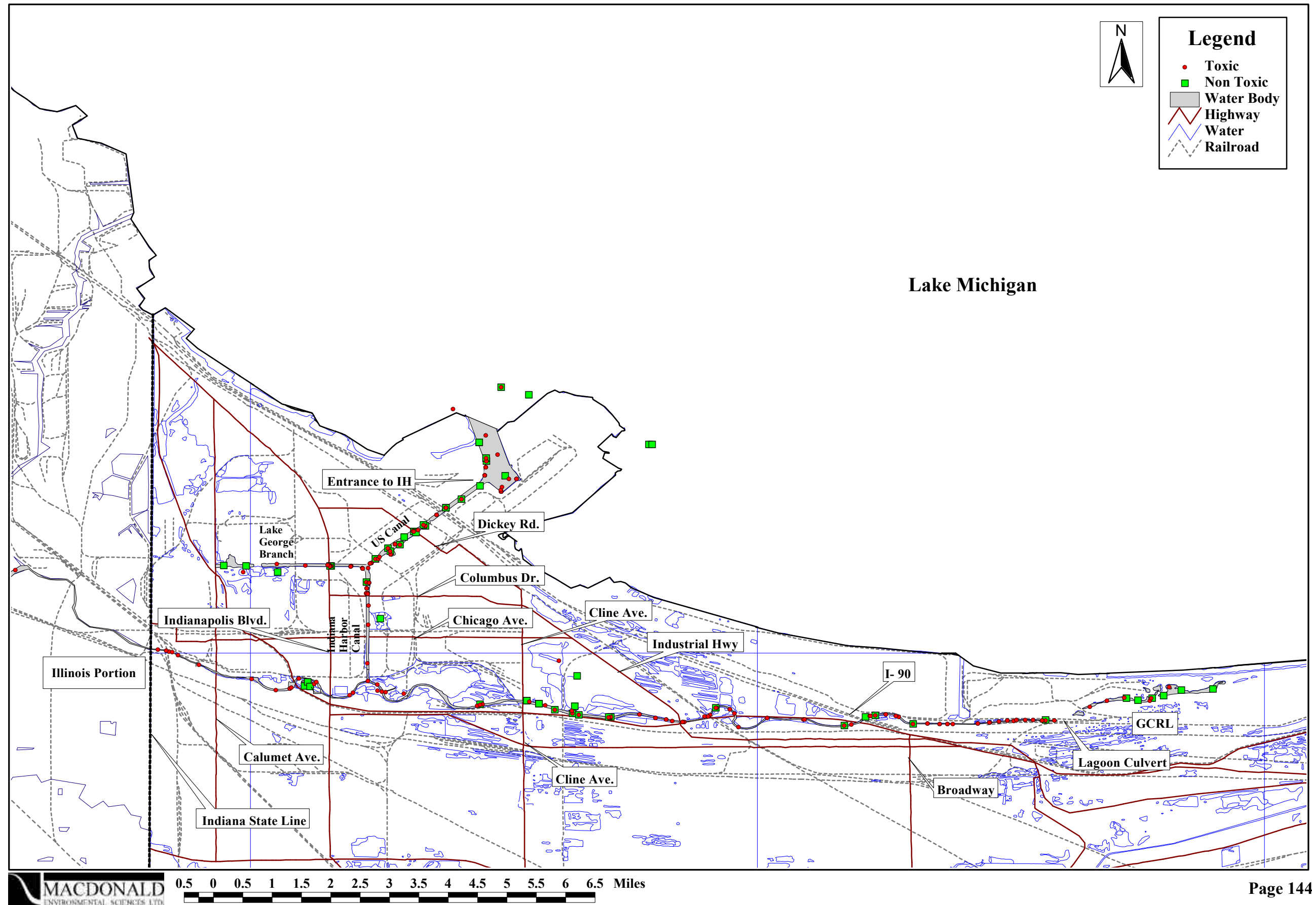
Figure 14.3. Areal extent of sediment toxicity in Assessment Area.
