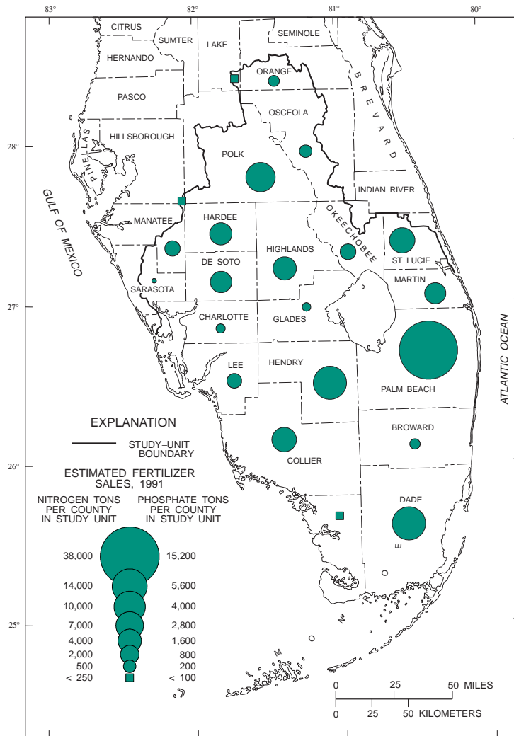
Figure 26. Estimated fertilizer sales, in tons of phosphate and nitrogen, in counties within the study unit, south Florida. (USEPA, 1990.) (1991 data calculated by Jerald Fletcher, West Virginia University, using a method described in the USEPA publication.)
