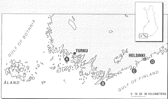
Figure 1. Locations in the Gulf of Finland where common eider Somateria mollissima carcasses and blood samples were collected for trace element analysis: Rymättylä (A), Tvärminne (B), Rönnskär (C), and Söderskär (D).
