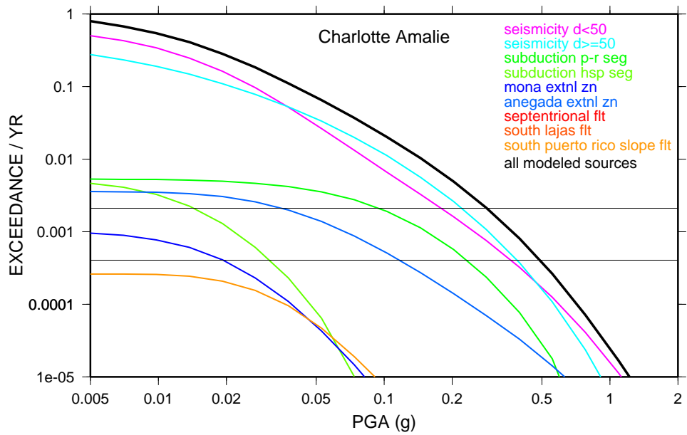
Fig.13d: PGA hazard curves for Charlotte Amalie.
