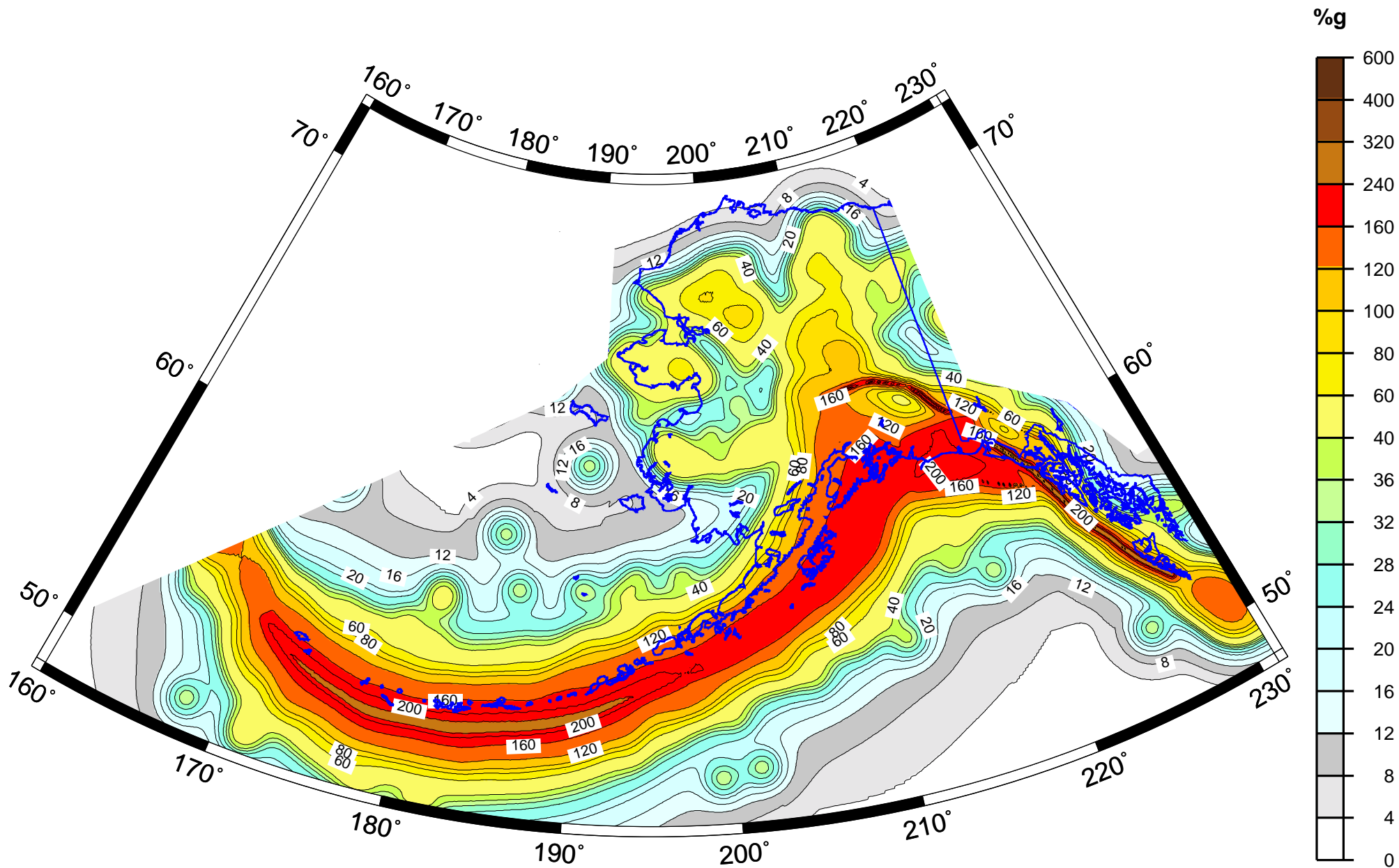
5 Hz Spectral Acceleration (%g) with 2% Probability of Exceedance in 50 Years
