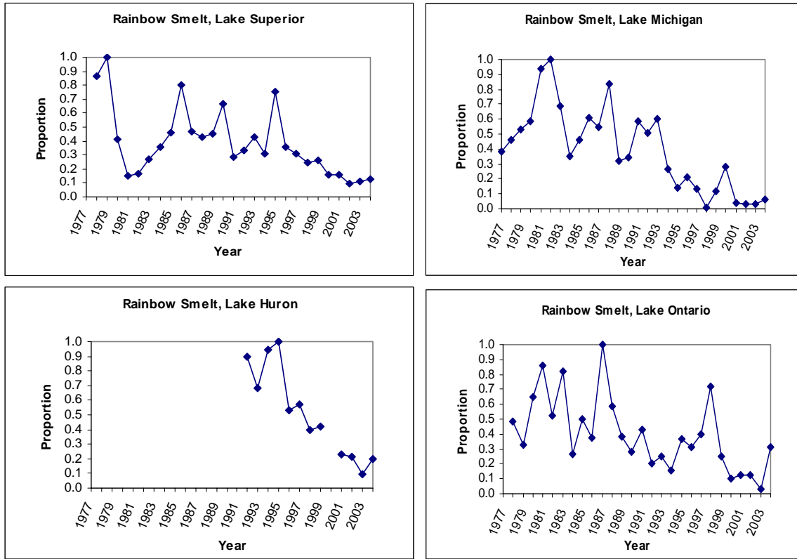
Figure 3. – Standardized indices of biomass for age-1 and older rainbow smelt in lakes Superior, Michigan, Huron, and Ontario 1977-2004. Lake Huron was not sampled in 2000 and the sampling gear used prior to 1992 differed from that used during 1992-2004.
