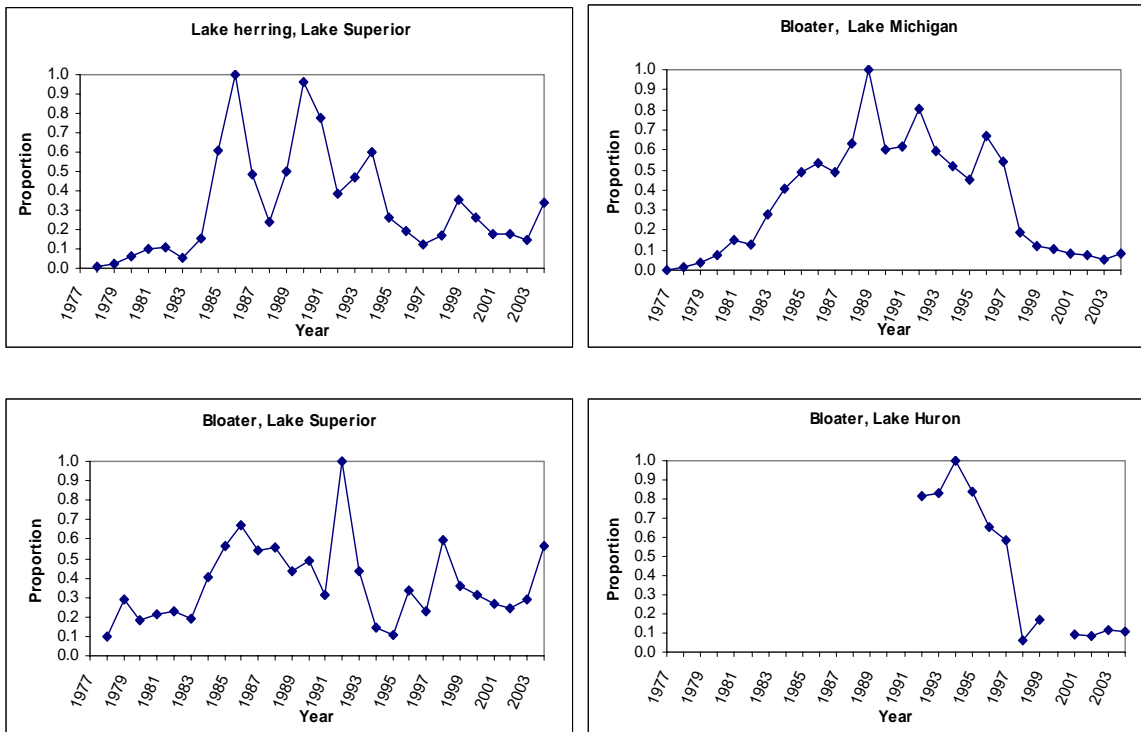
Figure 1. – Standardized indices of biomass for age-1 and older lake herring in Lake Superior and for age-1 and older bloater in lakes Superior, Michigan, and Huron, 1977-2004. Lake Huron was not sampled in 2000 and the sampling gear used prior to 1992 differed from that used during 1992-2004.
