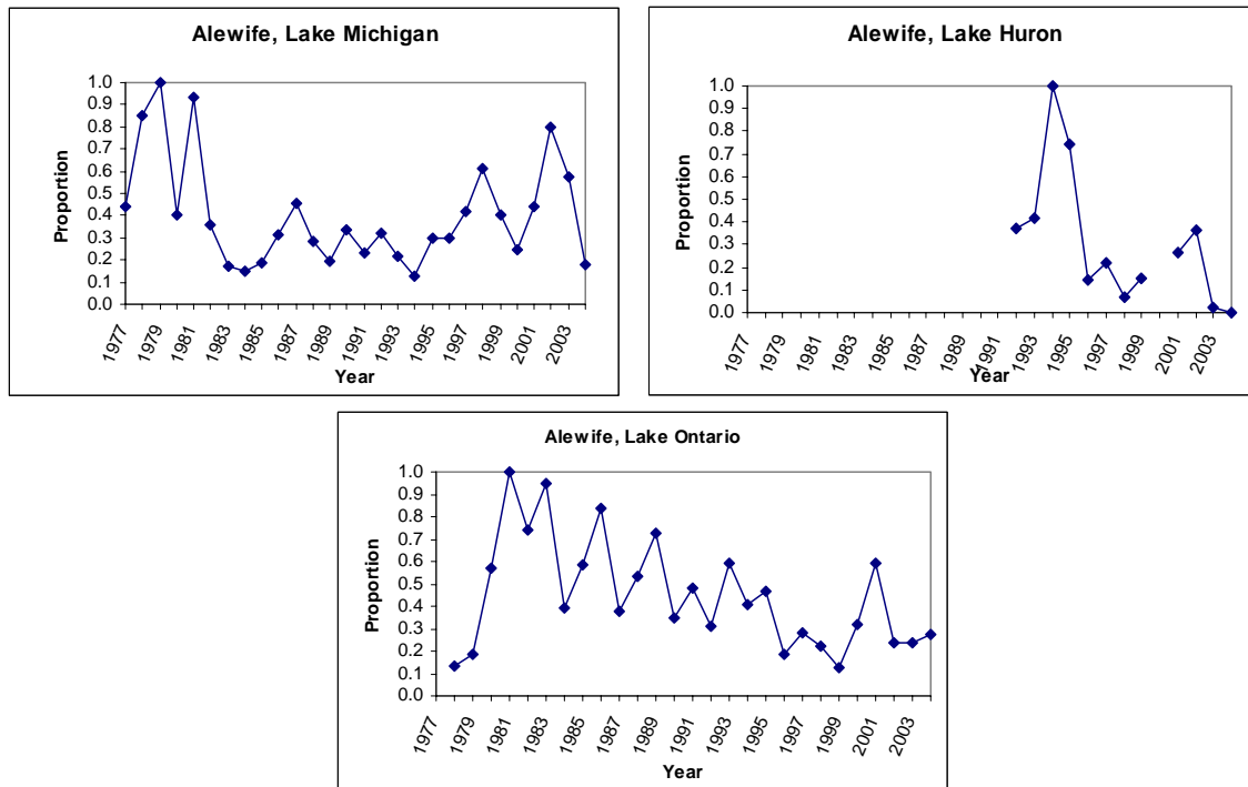
Figure 2. – Standardized indices of biomass for adult alewife in lakes Michigan, Huron, and Ontario, 1977-2004. Adult alewife are those fish that have completed two or more growing seasons; i.e. age 1 when surveys are conducted in fall (lakes Michigan and Huron) and age 2 when surveys are conducted in spring (Lake Ontario). Lake Huron was not sampled in 2000 and the sampling gear used prior to 1992 differed from that used during 1992-2004.
