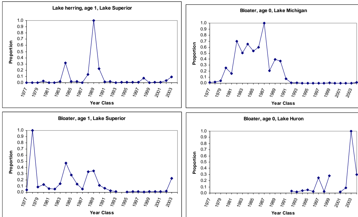
Figure 4. – Standardized indices of year-class strengths (age \leq 1 ) for lake herring and bloater in lakes Superior, Michigan, and Huron, 1977-2004. Lake Huron was not sampled in 2000 and the sampling gear used prior to 1992 differed from that used during 1992-2004.
