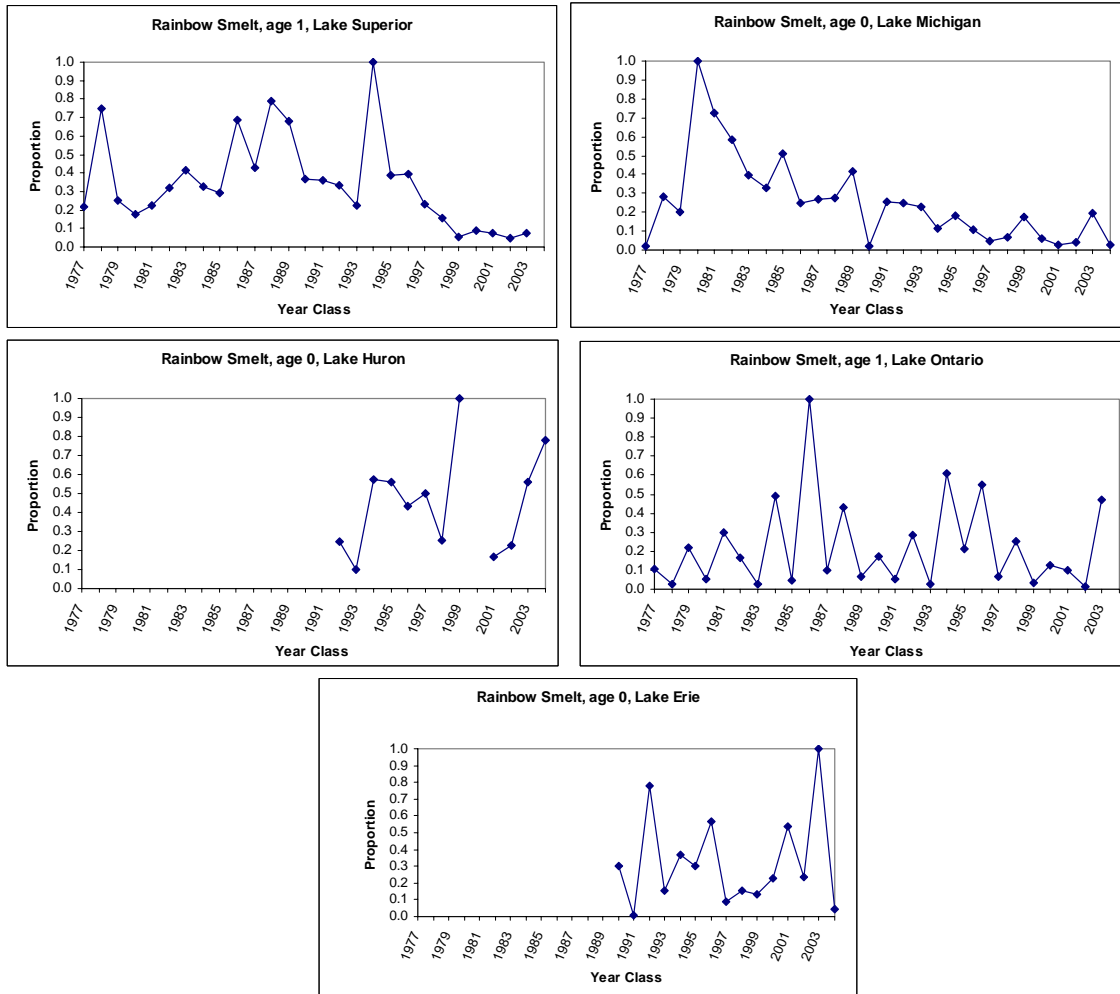
Figure 6. – Standardized indices of rainbow smelt year-class strengths measured at age 1, after the strength of the year-class is set in lakes Superior and Ontario and at age 0, after the strength of the year-class appears to be set in lakes Michigan and Huron, 1977-2004. Lake Huron was not sampled in 2000 and the sampling gear used prior to 1992 differed from that used during 1992-2004.
