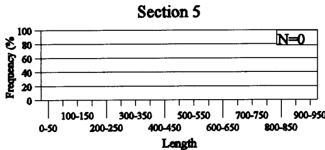
Figure 60. Length-frequency histograms of sand shiner collected from Missouri and Yellowstone River sections using drifting trammel nets, experimental gill nets, benthic trawls, bag seines, and boat electrofishing. Remaining data will appear in 1997 Age & Growth Analyses. See Table 1 for section definitions.
