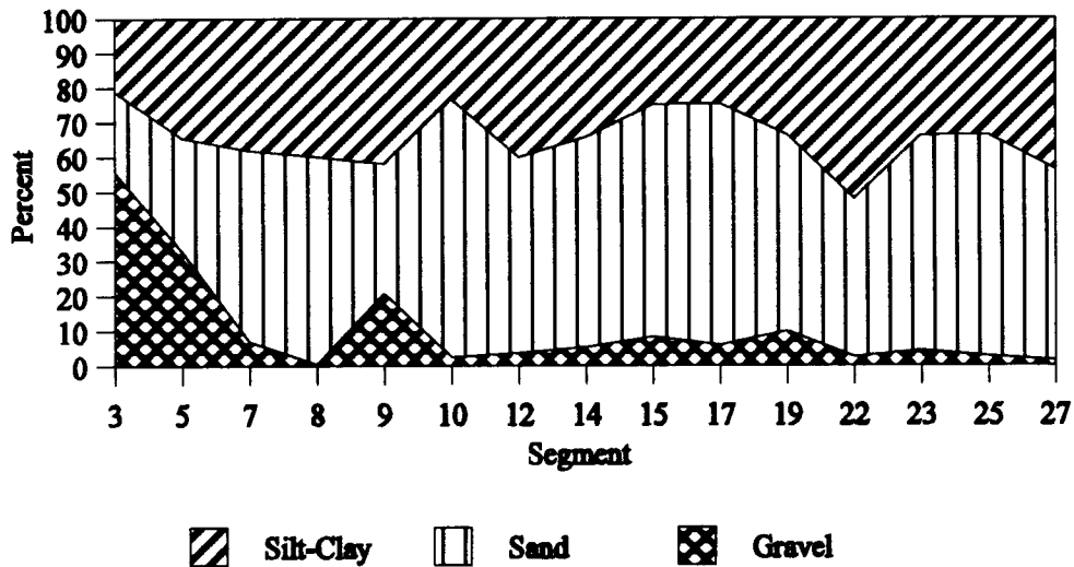
Figure 18. Average segment substrate proportions in Missouri and Yellowstone (9) study segments. Percentages are a proportional representation of the occurrence of each substrate in relation to the others. Top graph contains overlapping proportional percentage data for each substrate type. Bottom graph stacks the three substrate types to show the fractionation of the three substrate types. Least-impacted segments: 3, 5, and 9; Inter-reservoir segments: 7, 8, 10, 12, 14, and 15; Channelized segments: 17, 19, 22, 23, 25, and 27.
