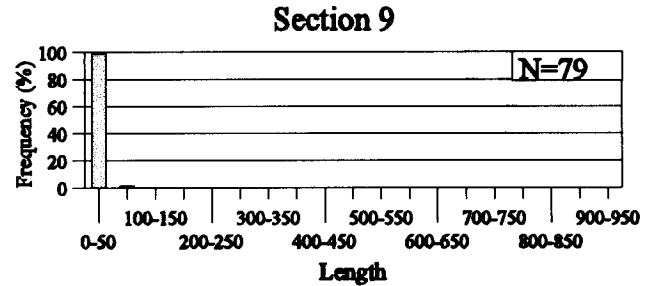
Figure 60. Length-frequency histograms of sand shiner collected from Missouri and Yellowstone River sections using drifting trammel nets, experimental gill nets, benthic trawls, bag seines, and boat electrofishing. Remaining data will appear in 1997 Age & Growth Analyses. See Table 1 for section definitions.
