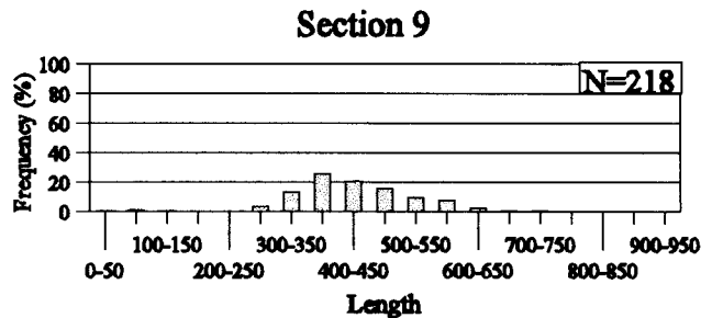
Figure 36. Length-frequency histograms of common carp collected from Missouri and Yellowstone River sections using drifting trammel nets, experimental gill nets, benthic trawls, bag seines, and boat electrofishing. See Table 1 for section definitions.
