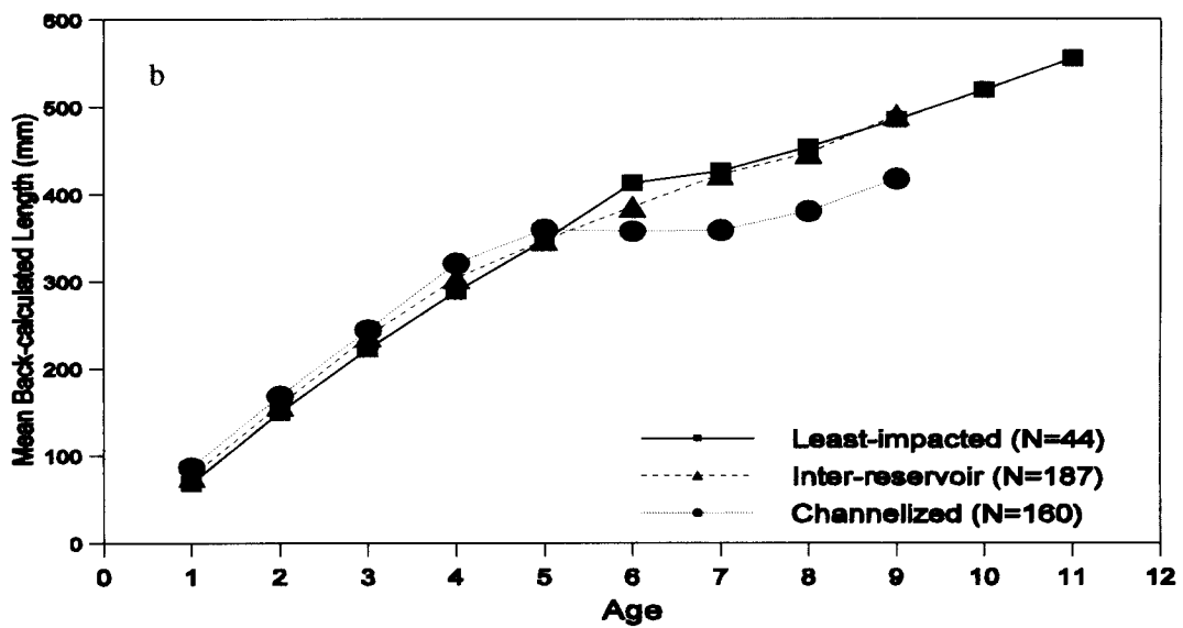
Figure 96. Age frequency distribution (a) and mean back-calculated length at age (b) for river carpsuckers collected in 1996.
