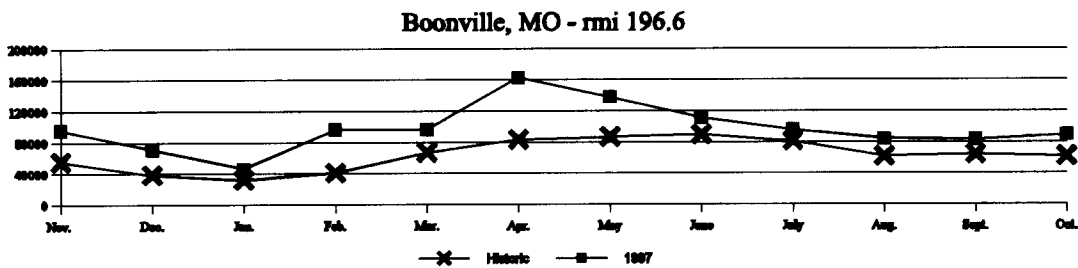
Figure 1. Historic (X's: Landusky- 1934-1996; Bismarck- 1954-1996; Omaha- 1953-1996; Booneville- 1953-1996) and 1997 (squares) mean monthly discharge for four locations along the Missouri River. Note y-axis scales vary with gauging station location.
