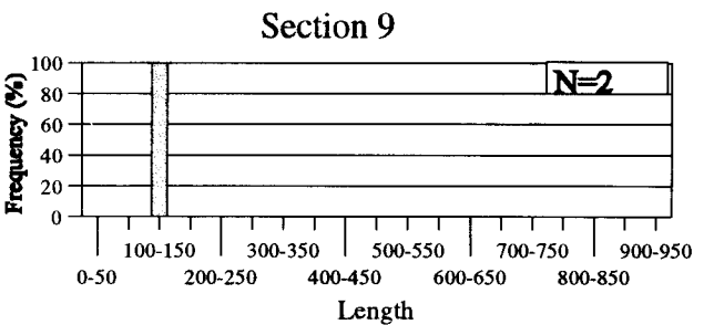
Figure 84. Length-frequency histograms of walleye collected from Missouri and Yellowstone River sections using drifting trammel nets, experimental gill nets, benthic trawls, bag seines, and boat electrofishing. See Table 1 for section definitions.
