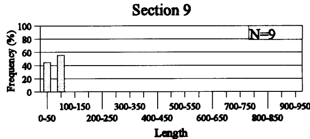
Figure 81. Length-frequency histograms of sturgeon chub collected from Missouri and Yellowstone River sections using drifting trammel nets, experimental gill nets, benthic trawls, bag seines, and boat electrofishing. Remaining data will appear in 1997 Age & Growth Analyses. See Table 1 for section definitions.
