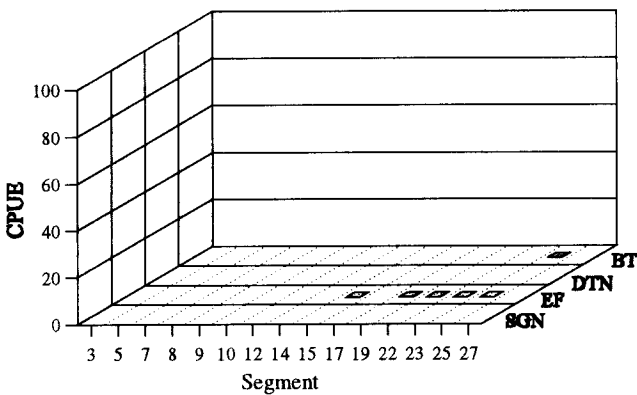
Figure 53. Trends of Hybognathus spp. catch rates among Missouri and Yellowstone River study segments and macrohabitats in 1997. This graph only shows species reported as Hybognathus spp. Any specific W. Silvery Minnow, Plains Minnow, or Brassy Minnow data will appear in the 1998 annual report as the 1997 Age & Growth Analyses. Catch rates are reported as #fish/100m for benthic trawl (BT) and drifting trammel net (DTN), #fish/180 degree haul for a bag seine (BS), #fish/hr for a statinary gill net (SGN), and #fish/min for electrofishing (EF). See Appendix A for list of macrohabitat acronyms.
