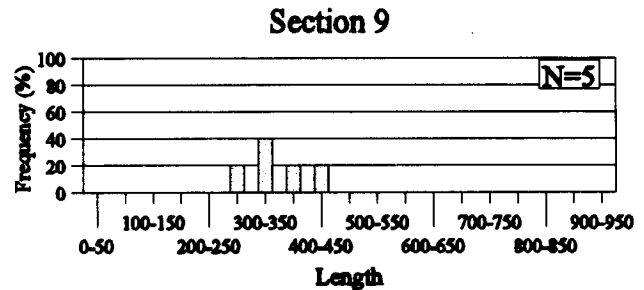
Figure 21. Length-frequency histograms of bigmouth buffalo collected from Missouri and Yellowstone River sections using drifting trammel nets, experimental gill nets, benthic trawls, bag seines, and boat electrofishing. See Table 1 for section definitions.
