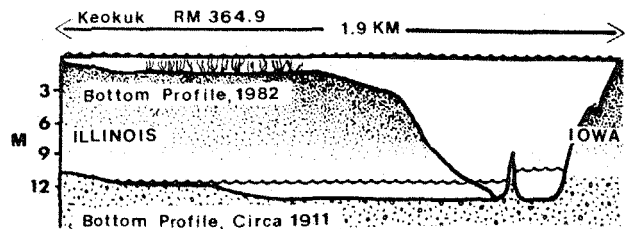
Figure 8. Bottom profile of the Mississippi River at RM 364.9, just above Lock and Dam 19.
