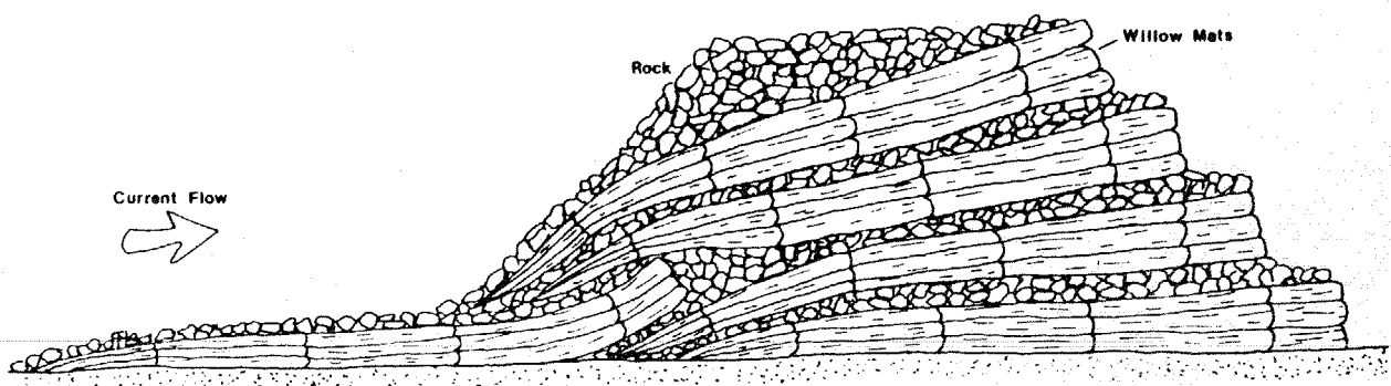
Figure 7. Cross section of a rock and brush wing dam on the Upper Mississippi River (from Boland 1980).
