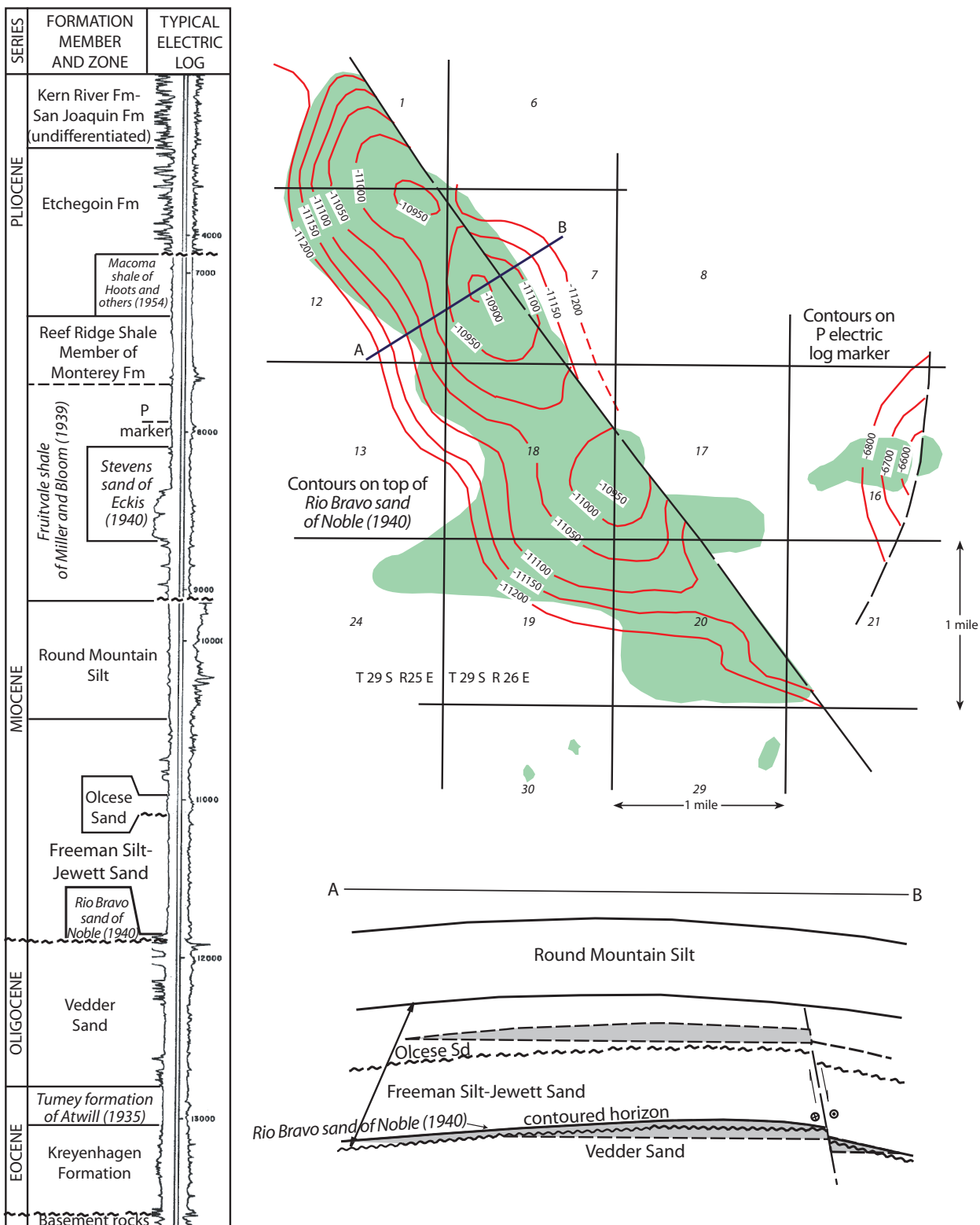
Figure 14.8. Figure of Greeley oil field, illustrating productive horizons below the Stevens sand. The large-offset Greeley fault confines up-dip production in the Olcese Sand, Rio Bravo sand of Noble (1940), and Vedder Sand pools. Green shading (underlying township-range grid) denotes reported 1998 limits of productive sand units within the field. All depths are in feet. Formations in italics denote informal geologic names. See figure 14.2 for location of field. Figure redrafted from CDOGGR (1998). Fm, Formation; Sd, Sand.
