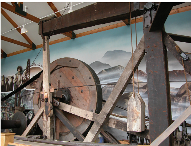
Figure 3.15. A partial view of the flywheel and beam used in early steam-powered drilling rigs. This is an authentic, cable-tool drill rig that has been reconstructed and is on display in the California Oil Museum in Santa Paula, California.
