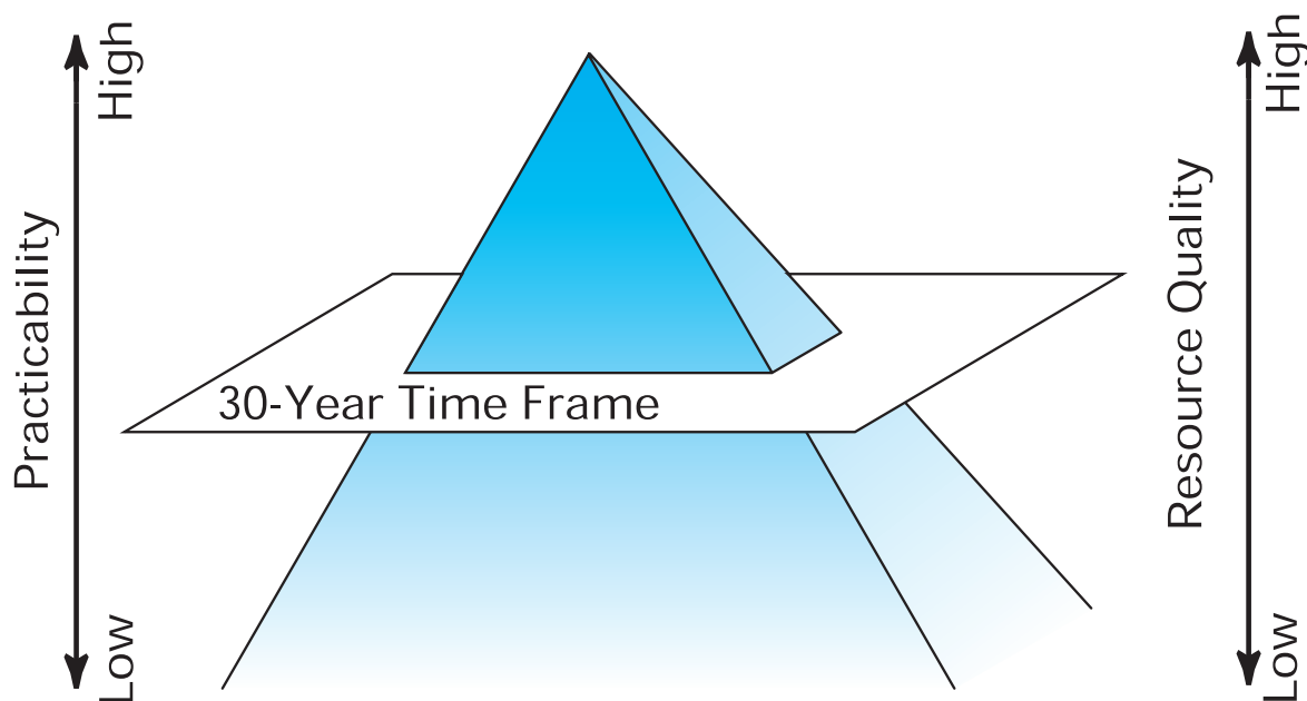
Figure 1. Sketch depicting a 30-year resource-assessment forecast span as a slice through the conventional-accumulation resource pyramid at some quality level. Accumulation categories below the selected slice level are excluded from assessment consideration. (Modified from McCabe, 1998.)
